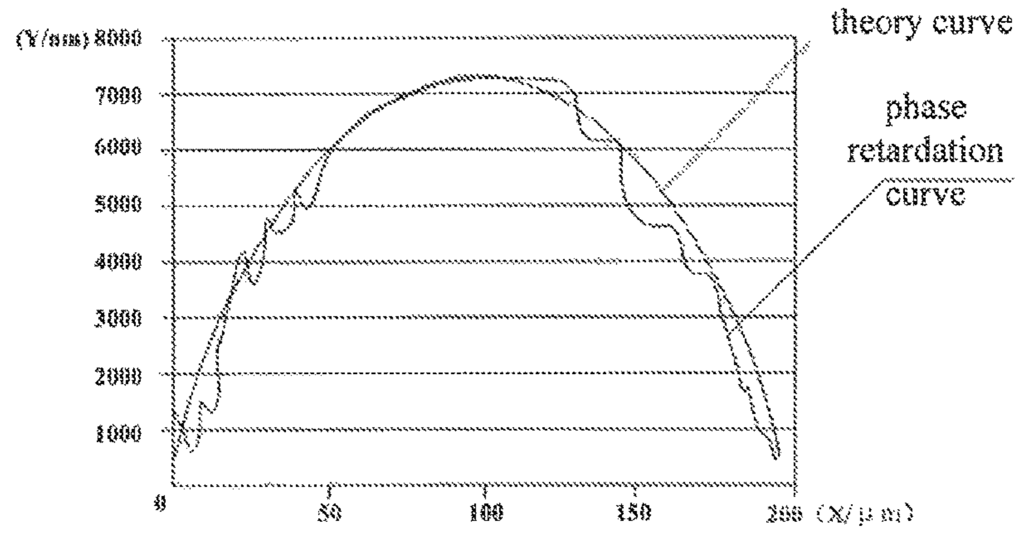
Fig. 3 (Prior Art)
