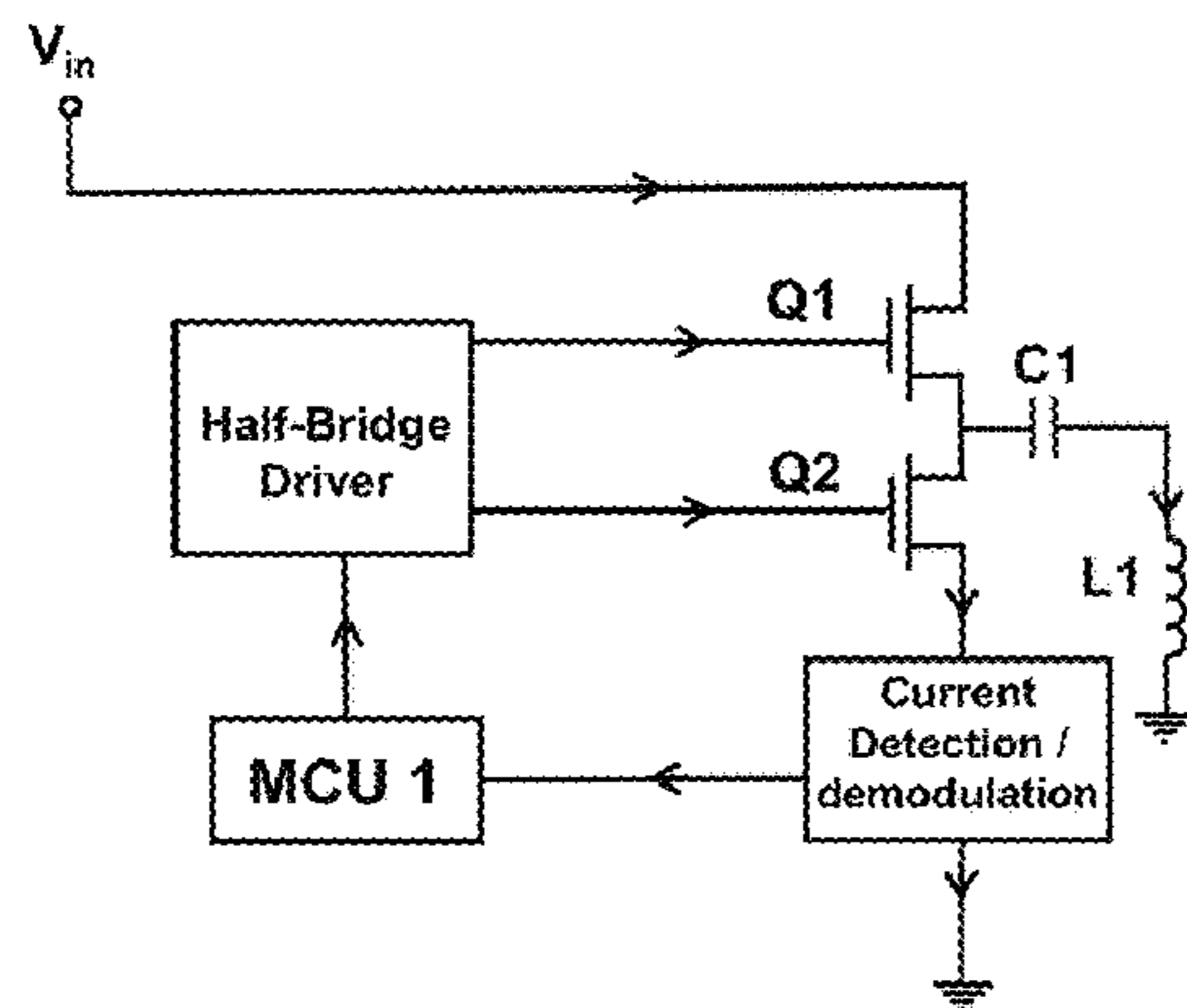
Charger 130
