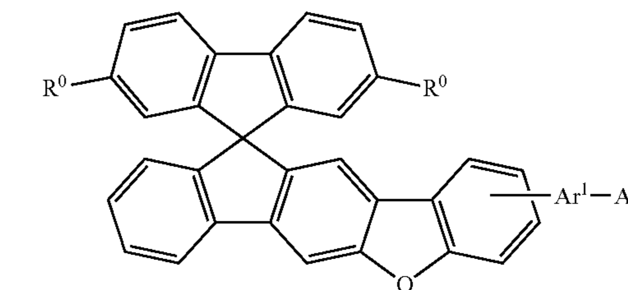
formula (I-9)
