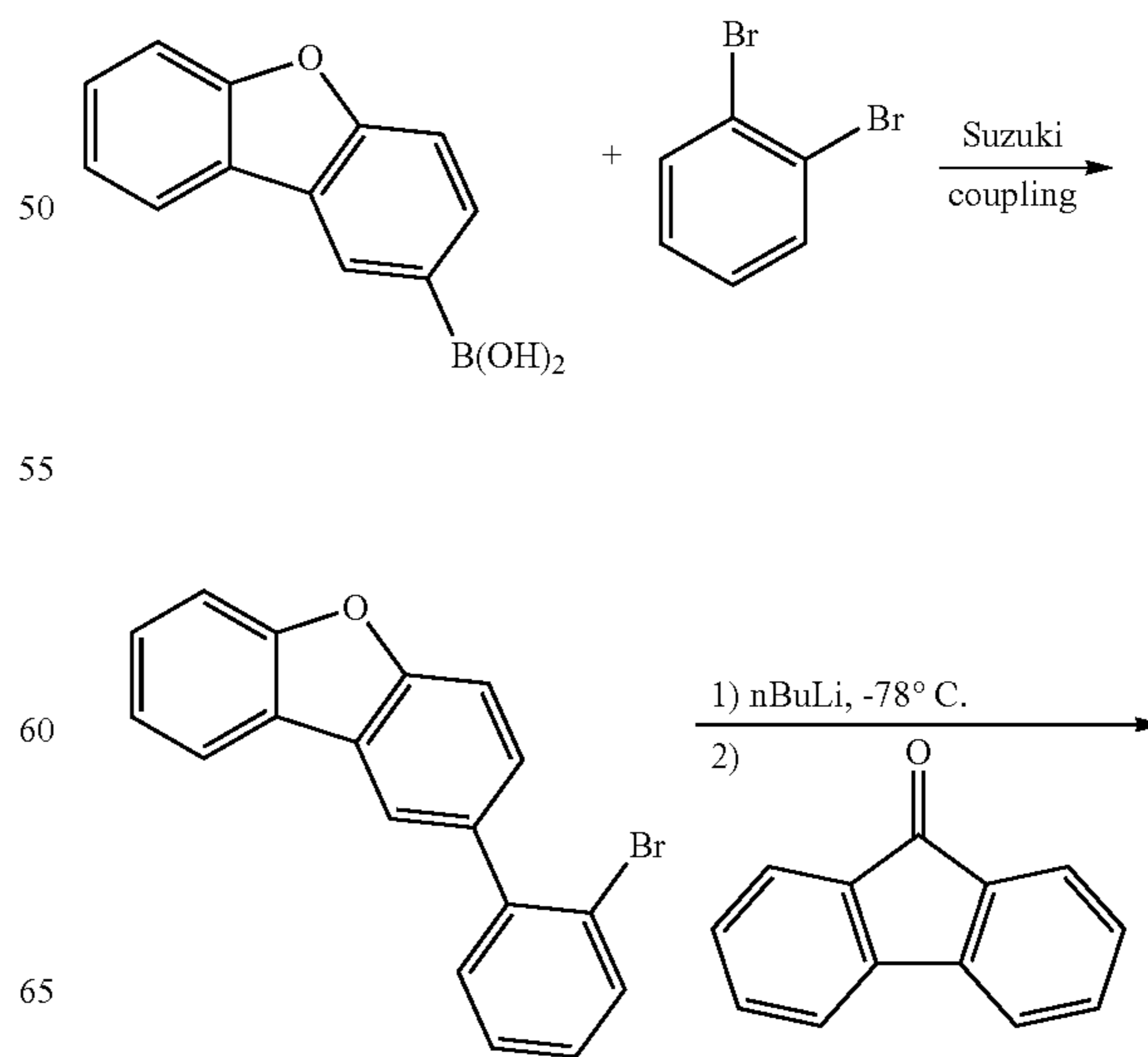
Scheme 8
