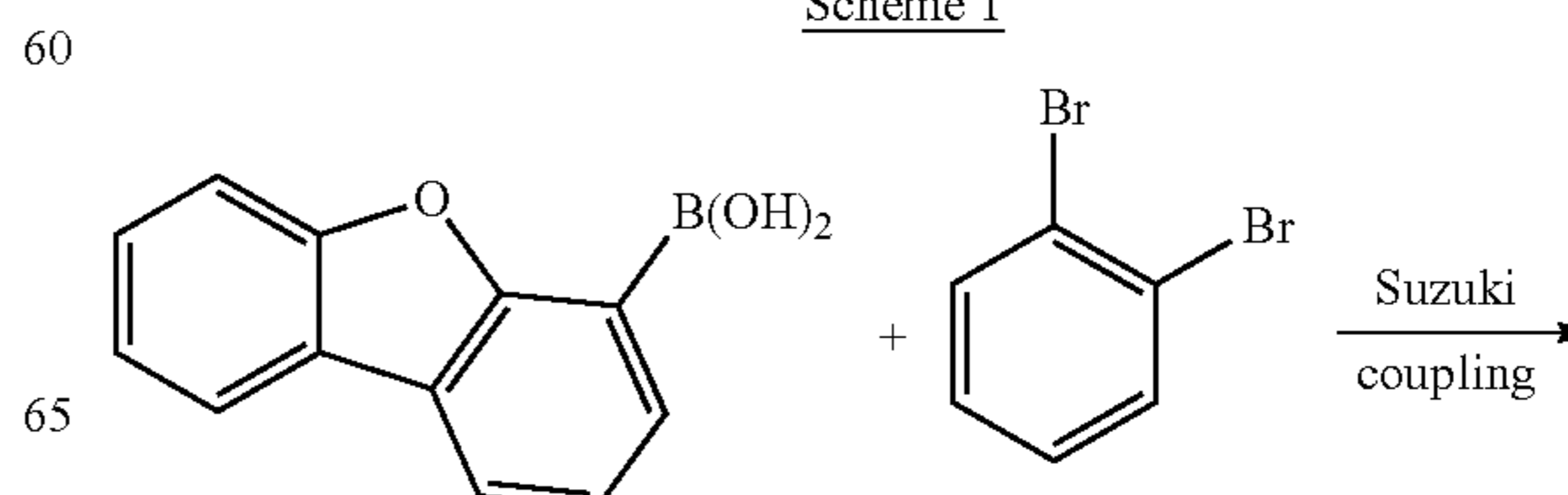
Scheme 1
