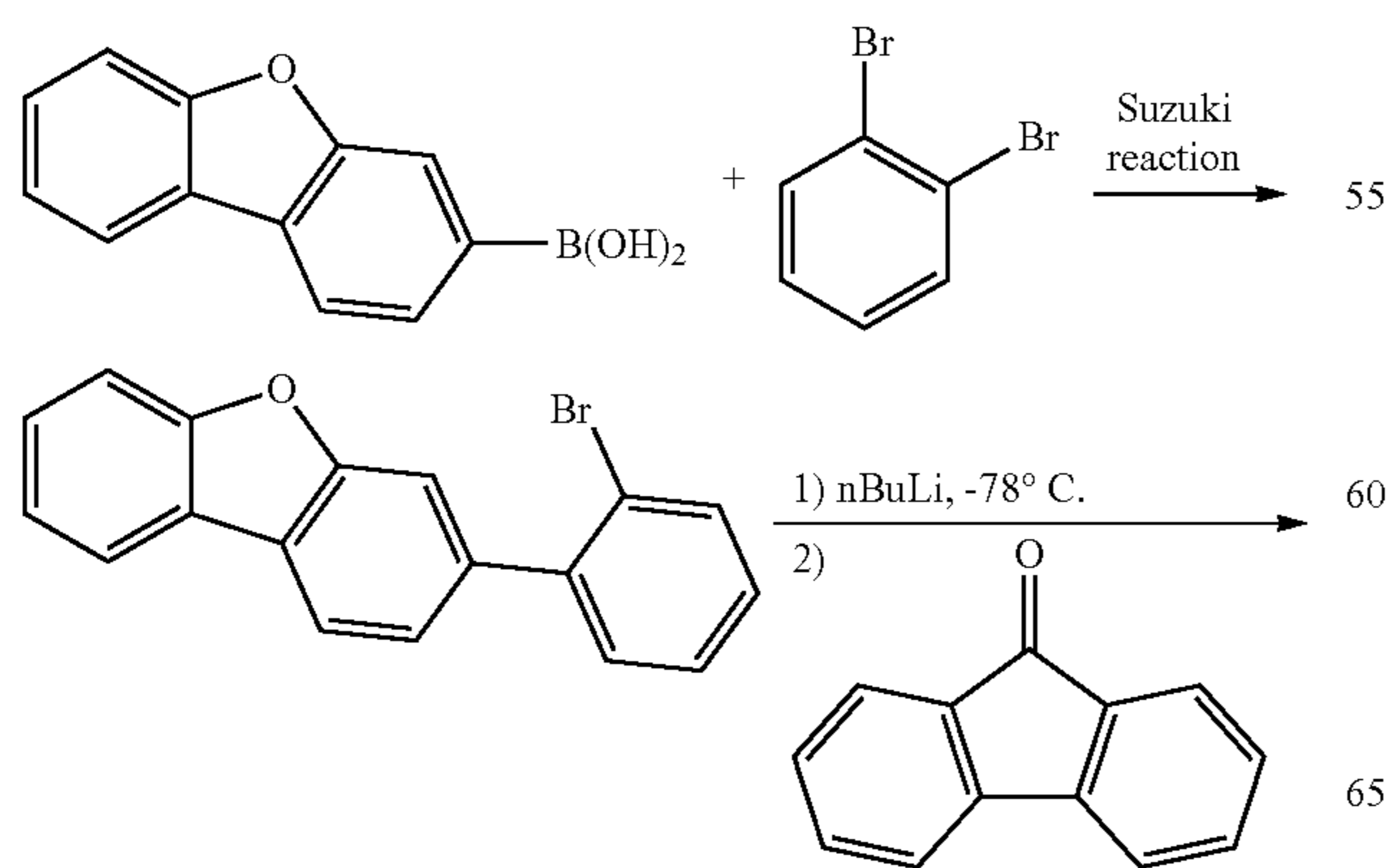
Scheme 7
