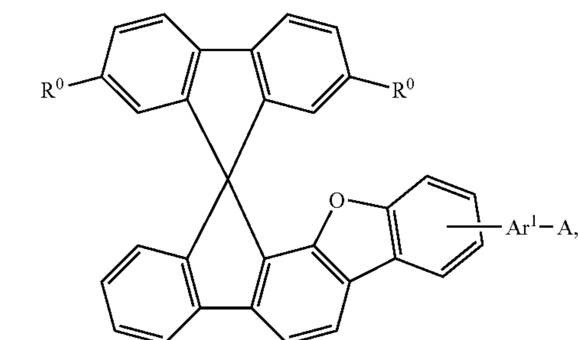
formula (I-18)
