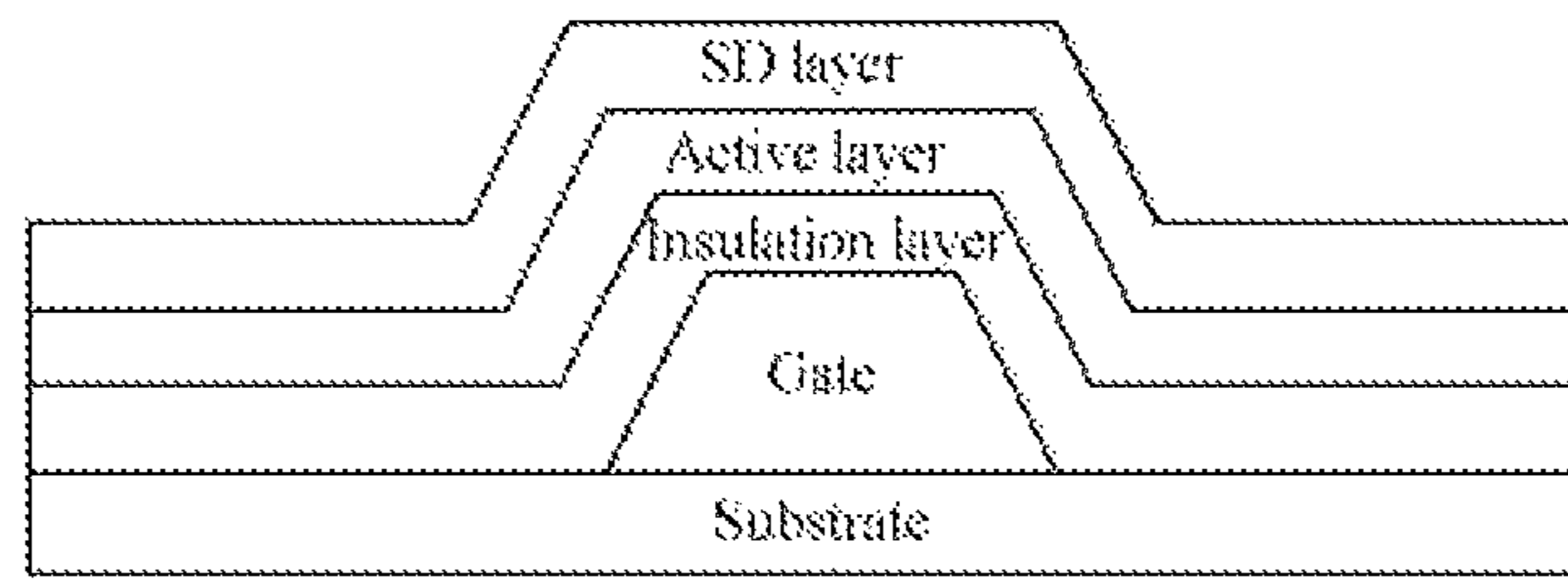
Fig. 3 Prior Art
