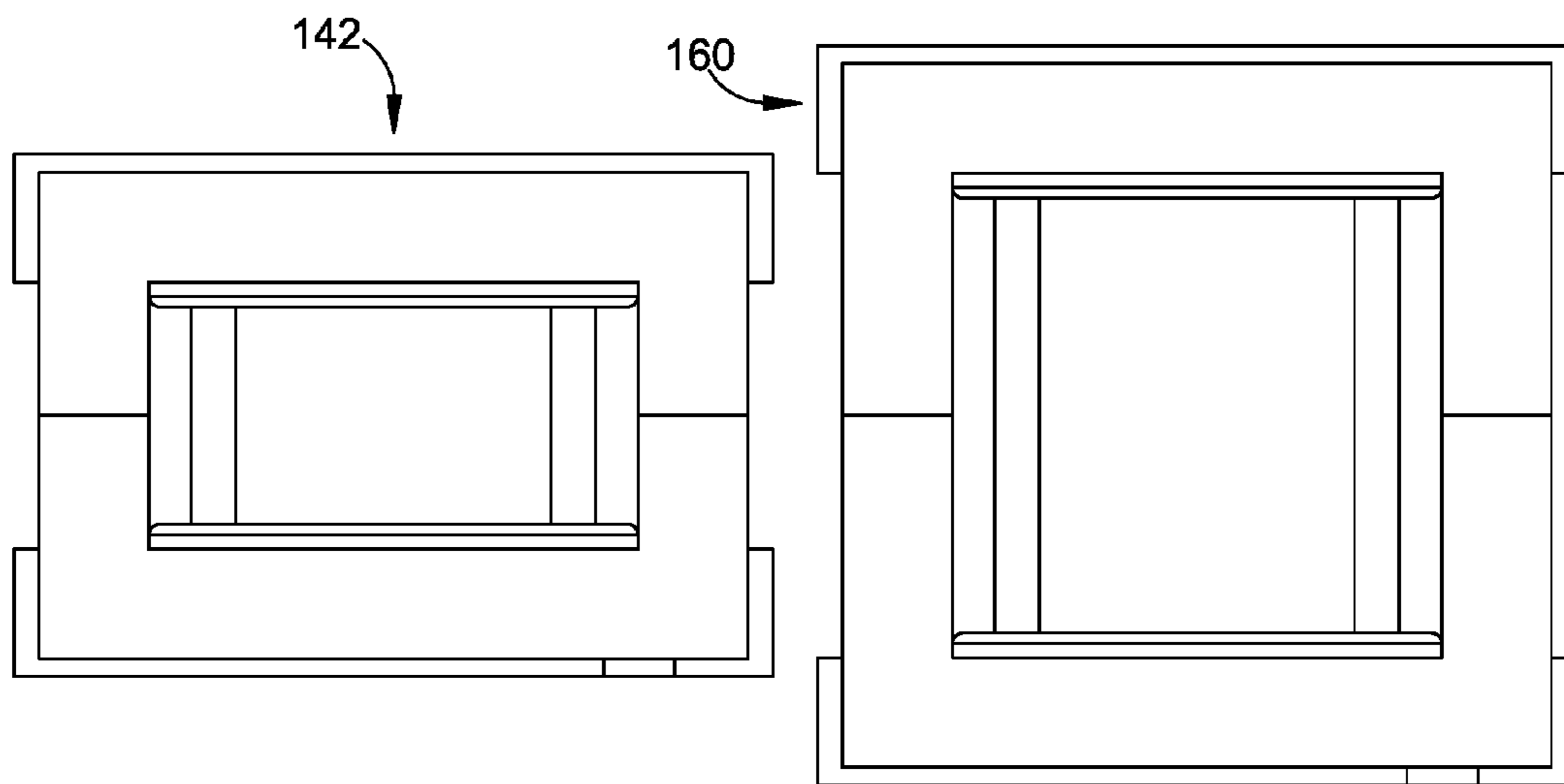
FIG. 6 (Prior Art)
