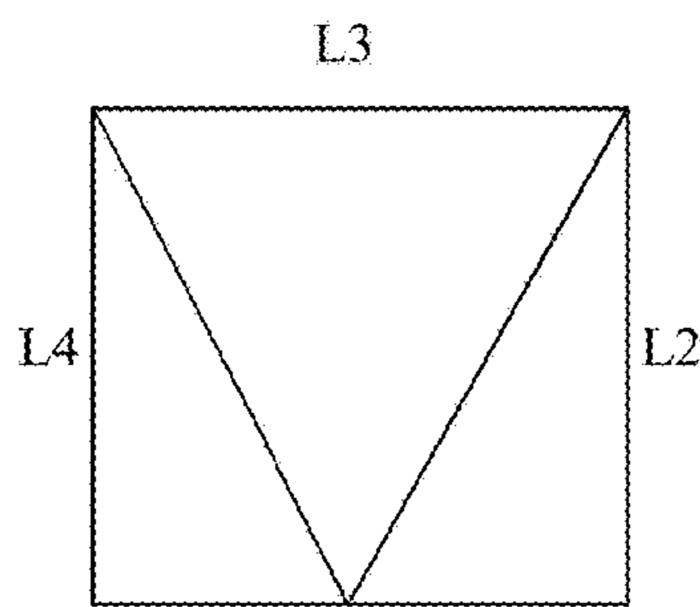
L1 L1=1, L2=0, L3=0, L4=0
