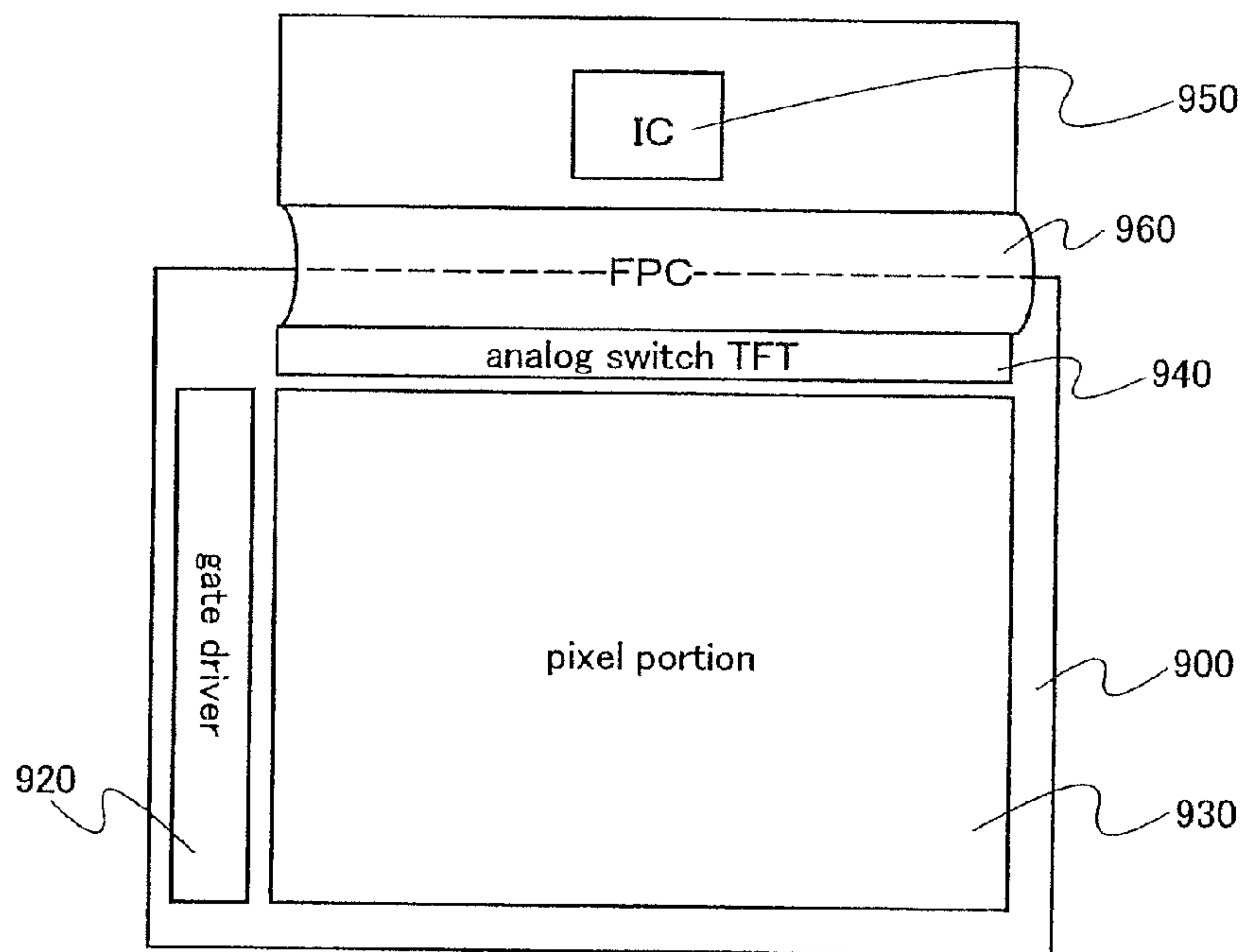
FIG. 17A IC connected by FPC
