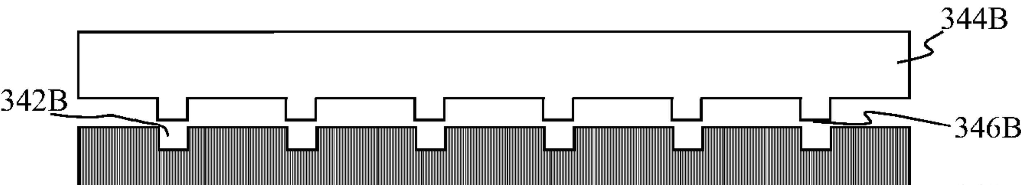
FIG. 43B (molding)
