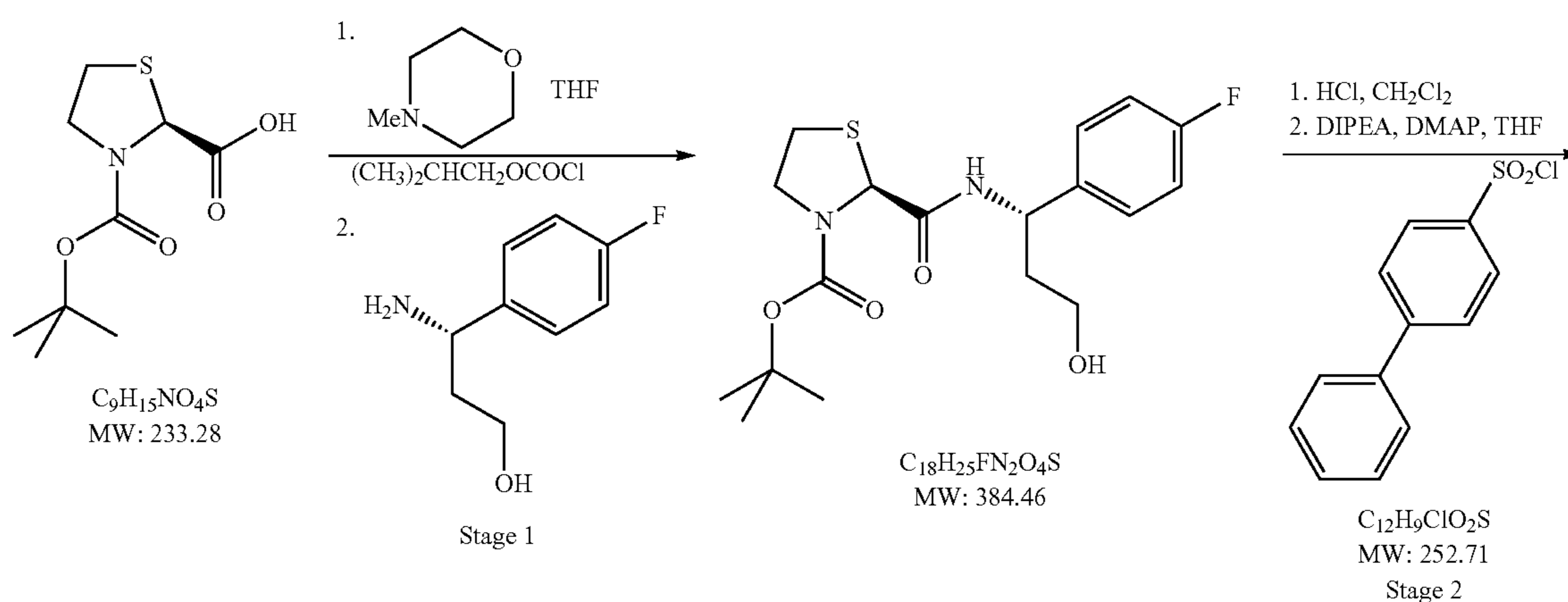
Scheme 1. Preparation of compound I and the chloride salt thereof
