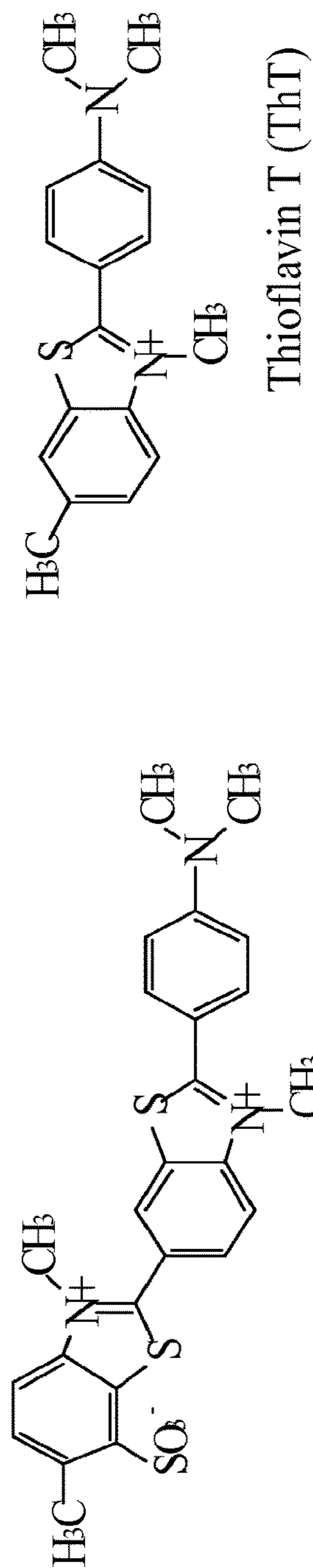
Proposed Structure of a Major Component of Thioflavin S (ThS)
