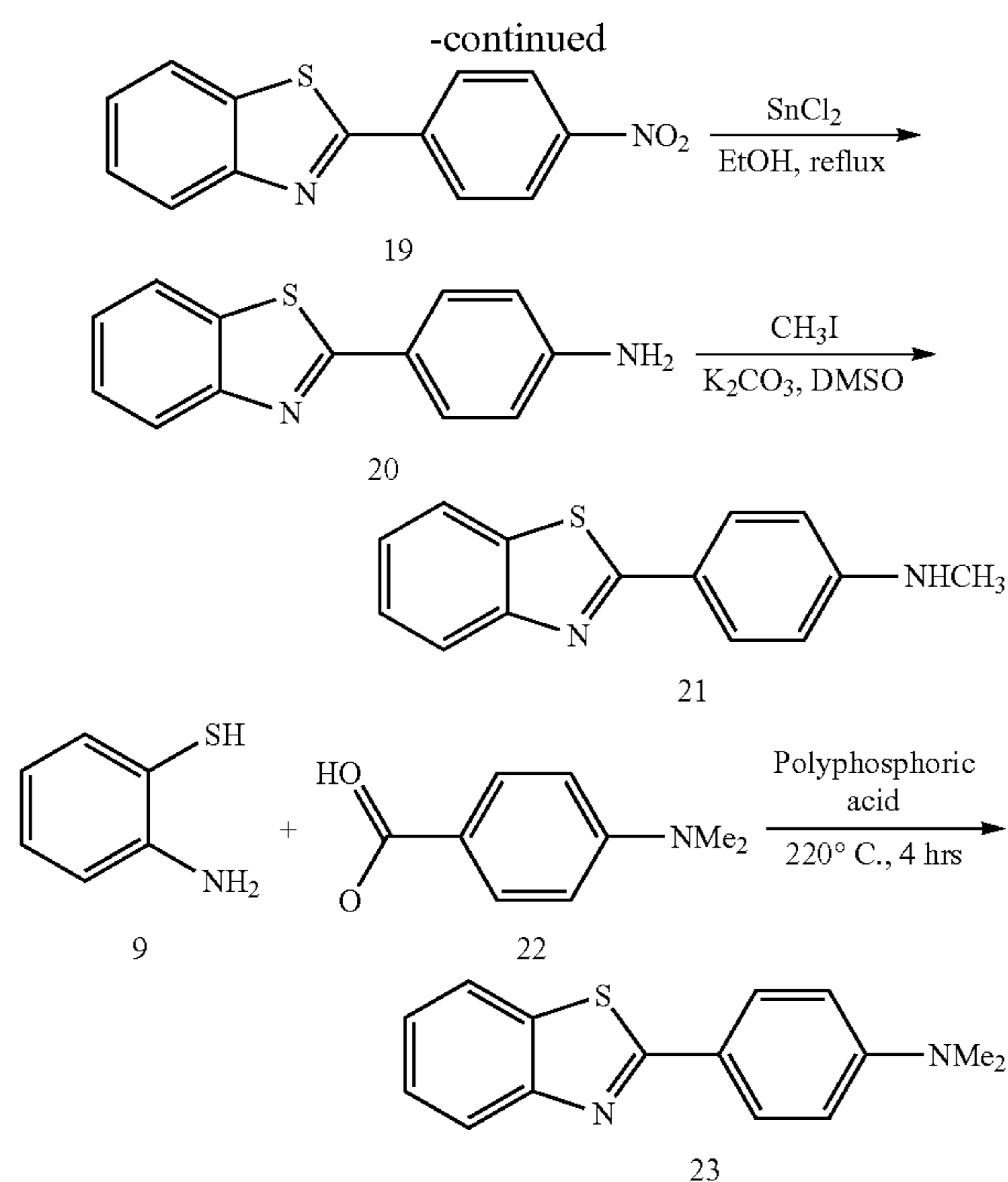
(a) 2-(4-Nitrophenyl)benzothiazole (19)
