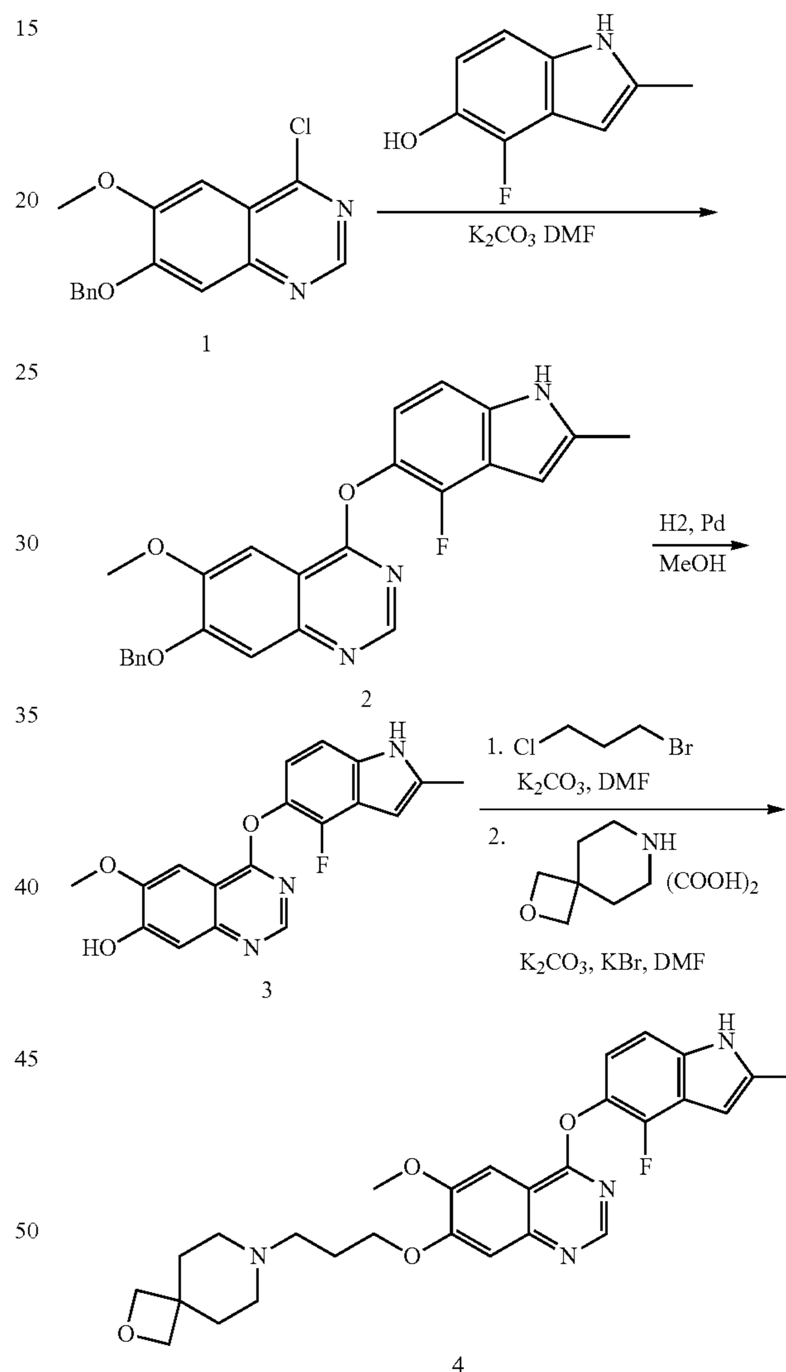
Scheme 1
