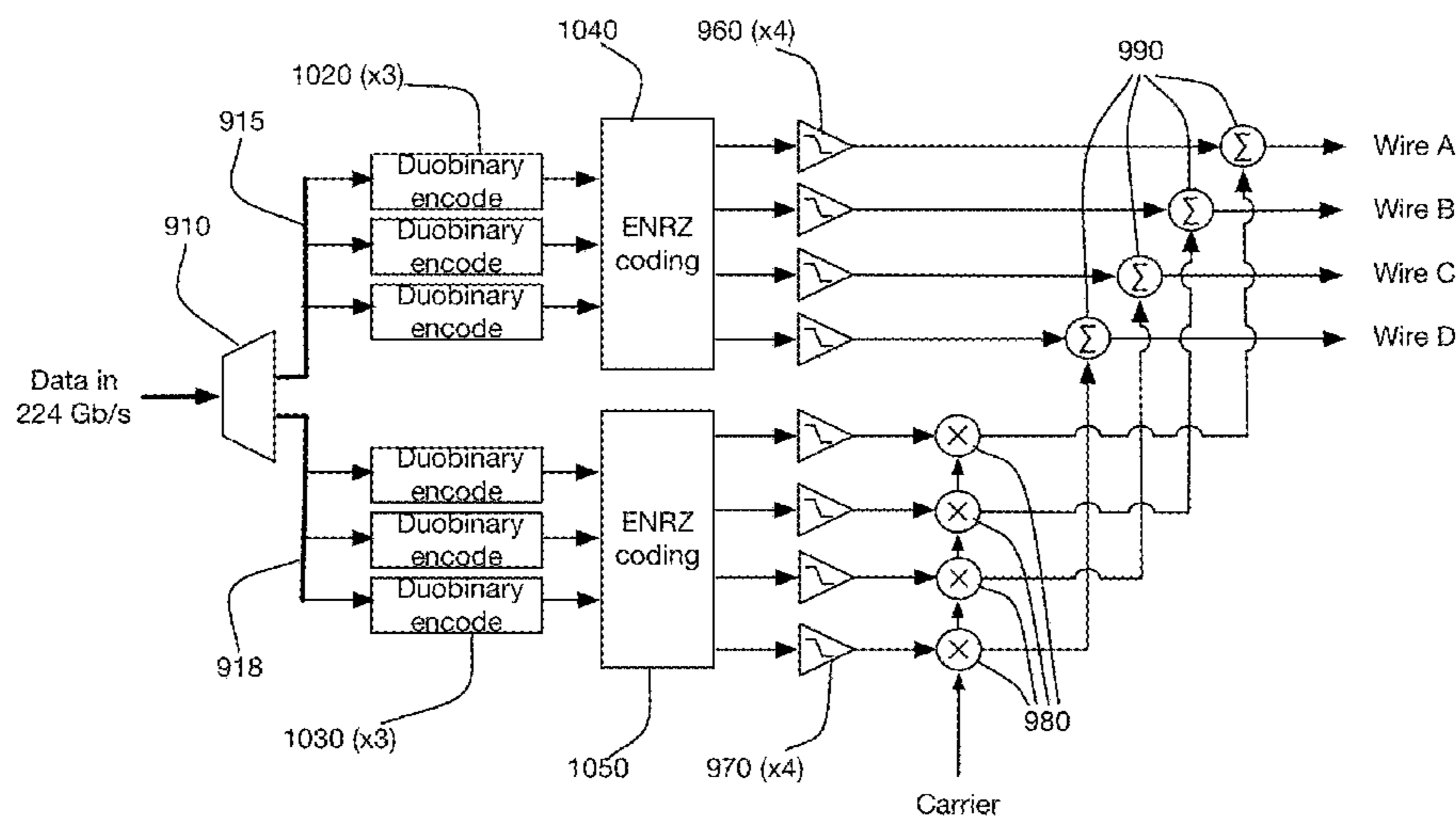
Alternative Transmitter
