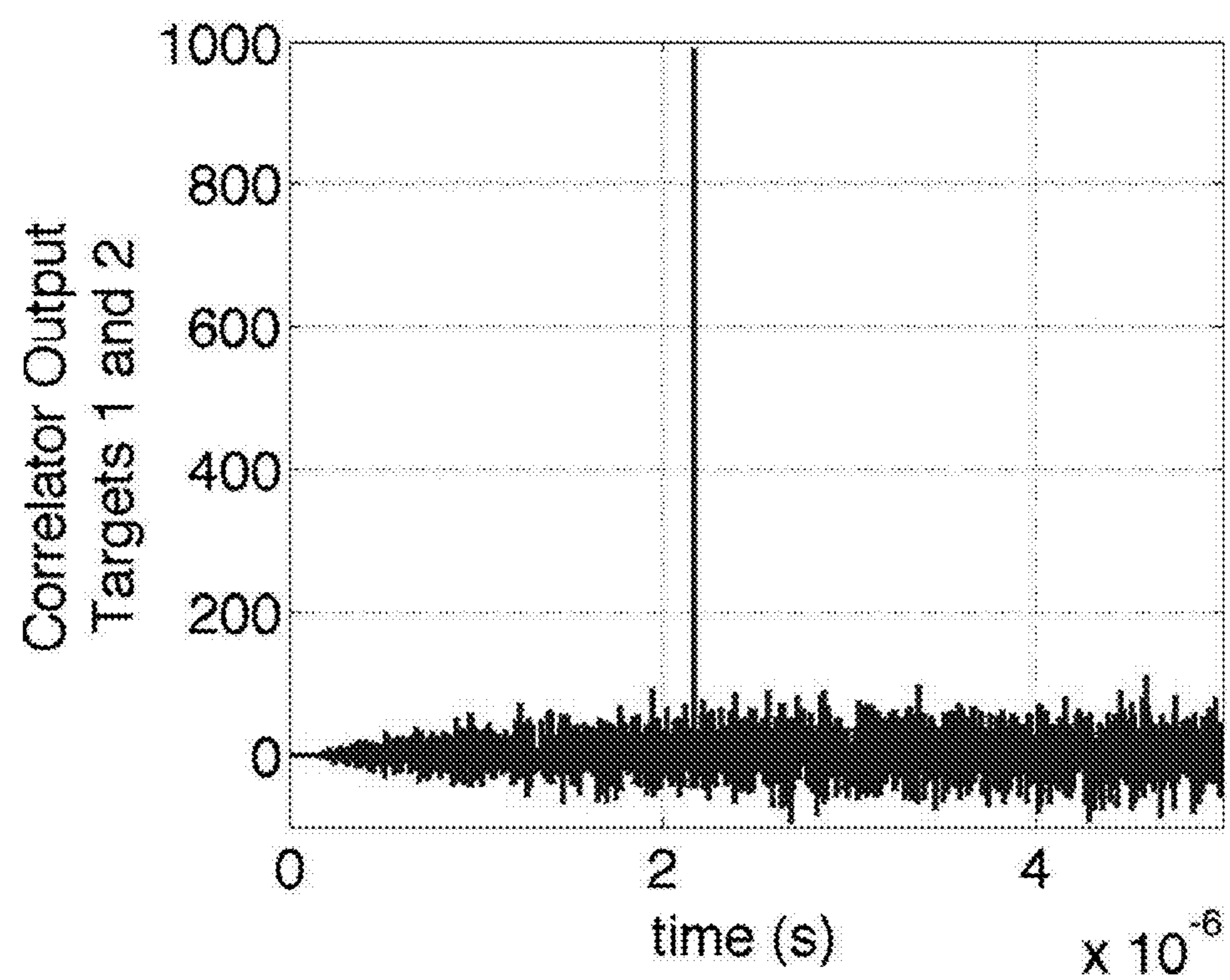
FIG. 14: Correlator outputs for total signal
