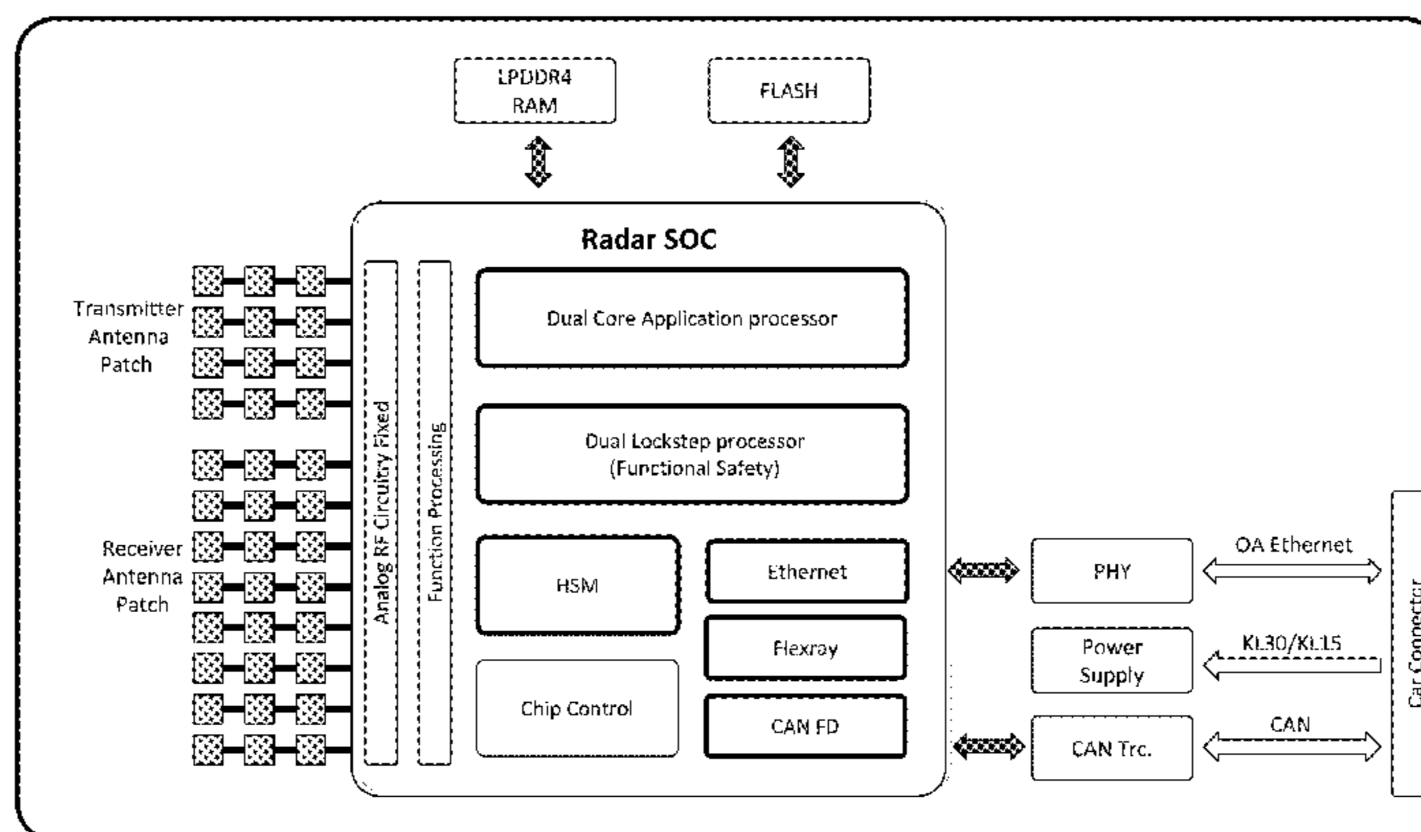
Radar system architecture
