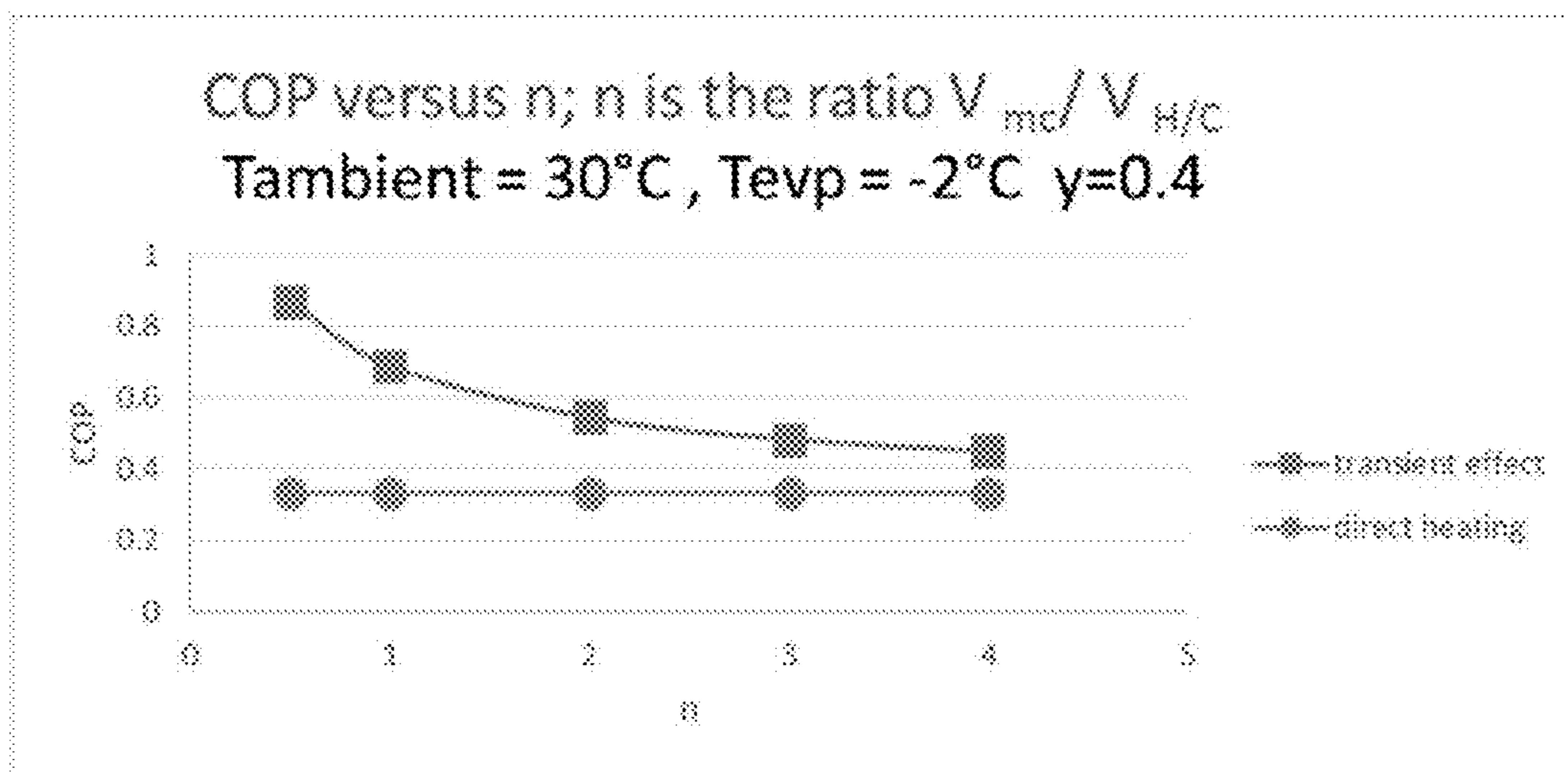
Fig. 16A COP versus n for R410a, T ambient = 30°C, T evp = -2°C, \gamma=0.4
