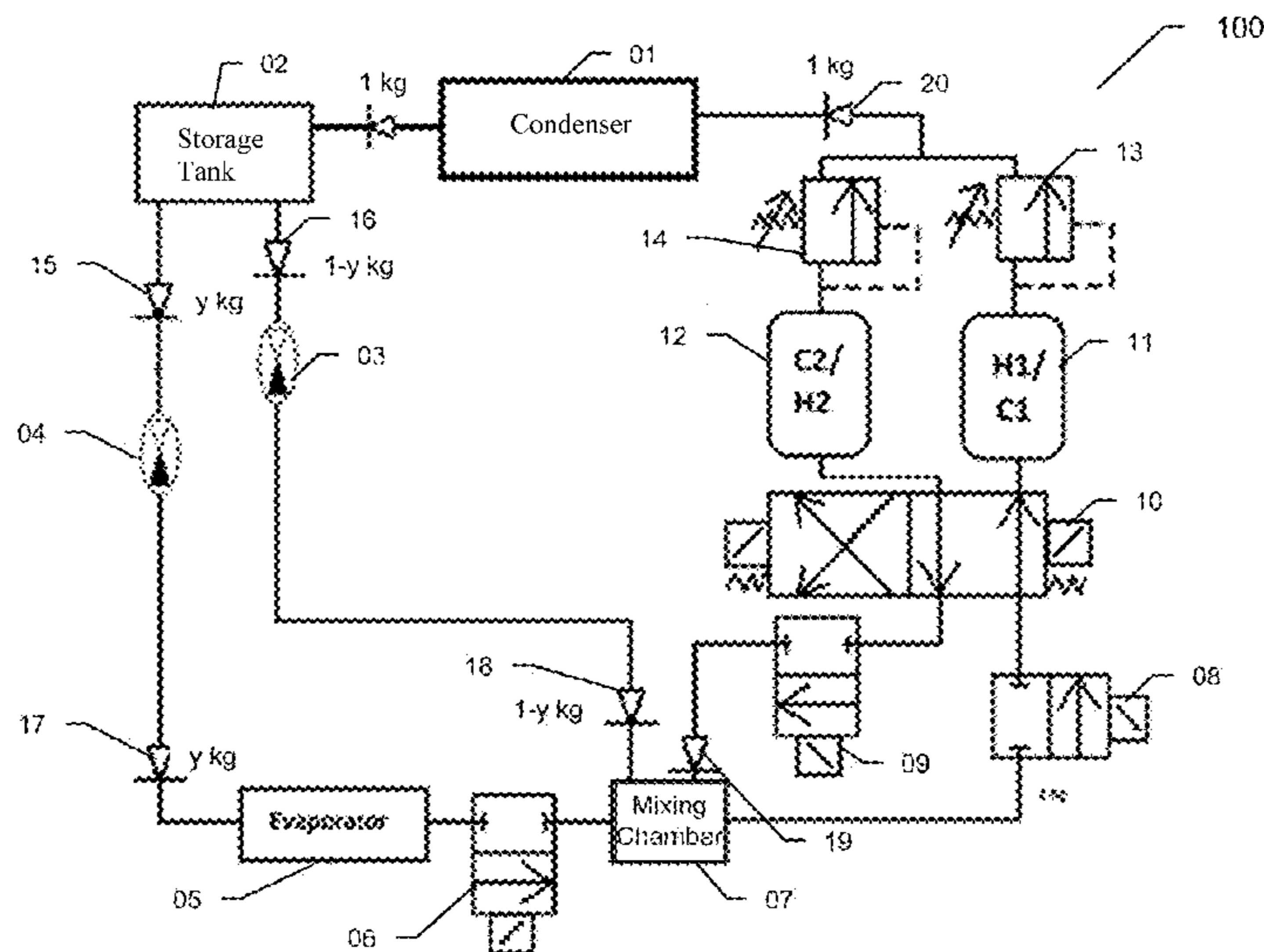
Refrigeration system
