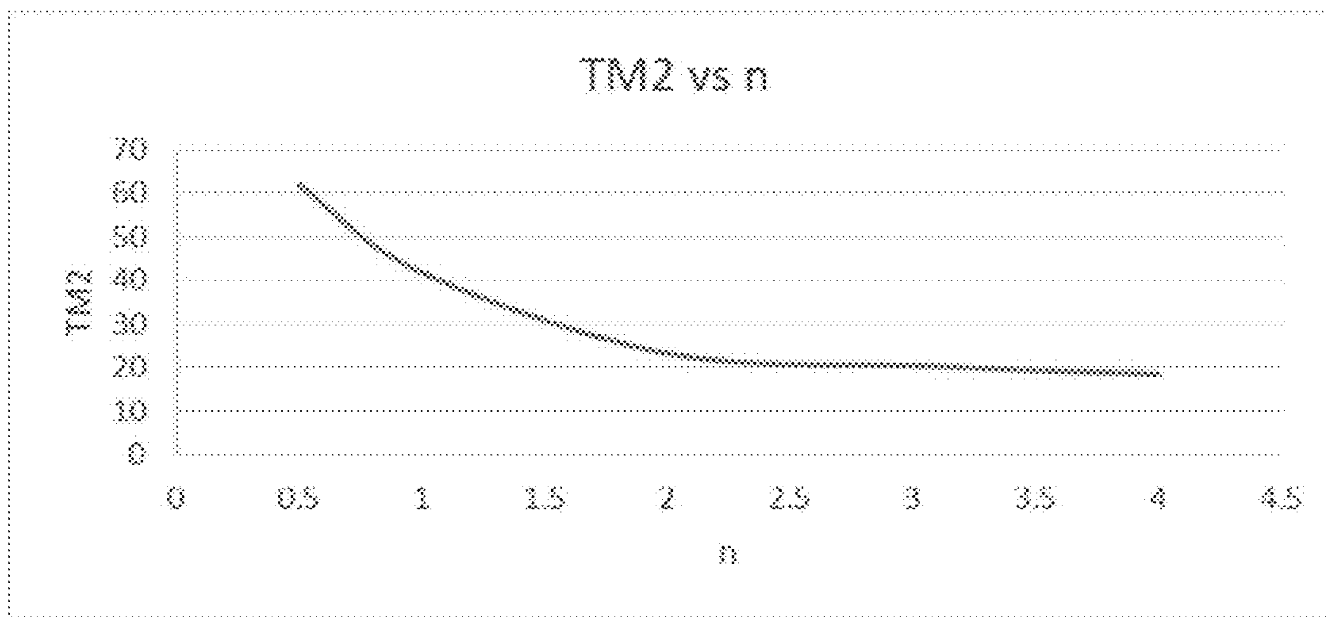
Fig. 14B TM2 versus n for R410a, T ambient = 40°C, T evaporator = 10°C, y=0.4
