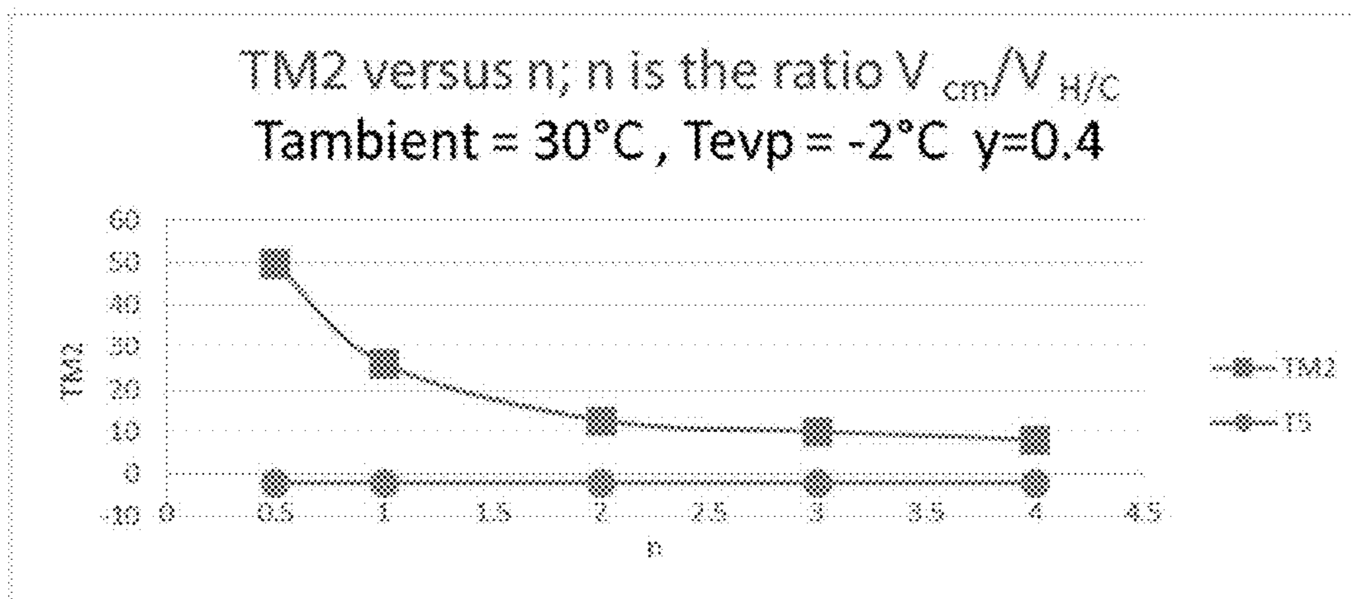
Fig. 16B TM2 versus n for R410a, T ambient = 30°C, T evp = -2°C, \gamma=0.4
