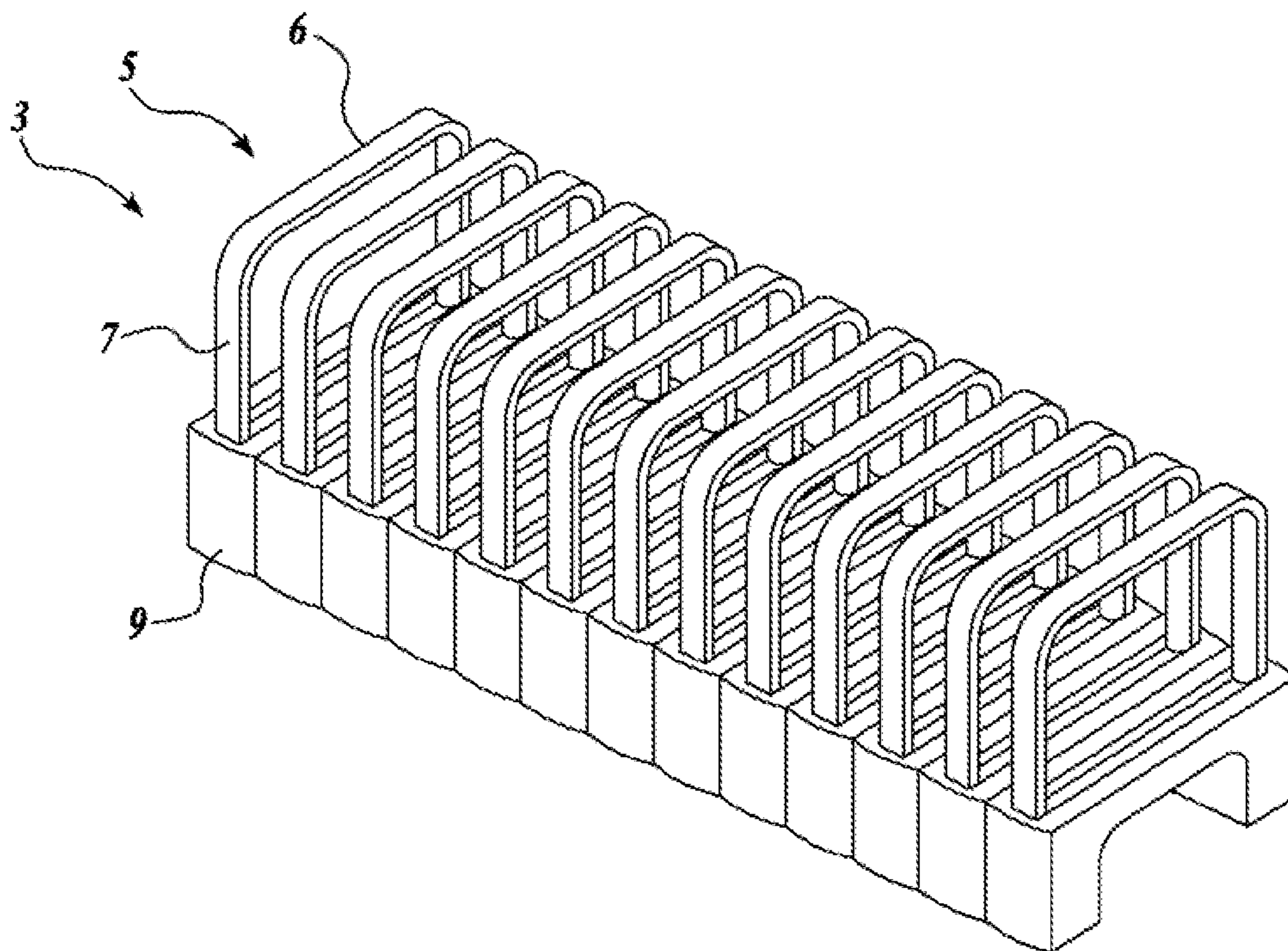
Fig. 1. (PRIOR ART)
