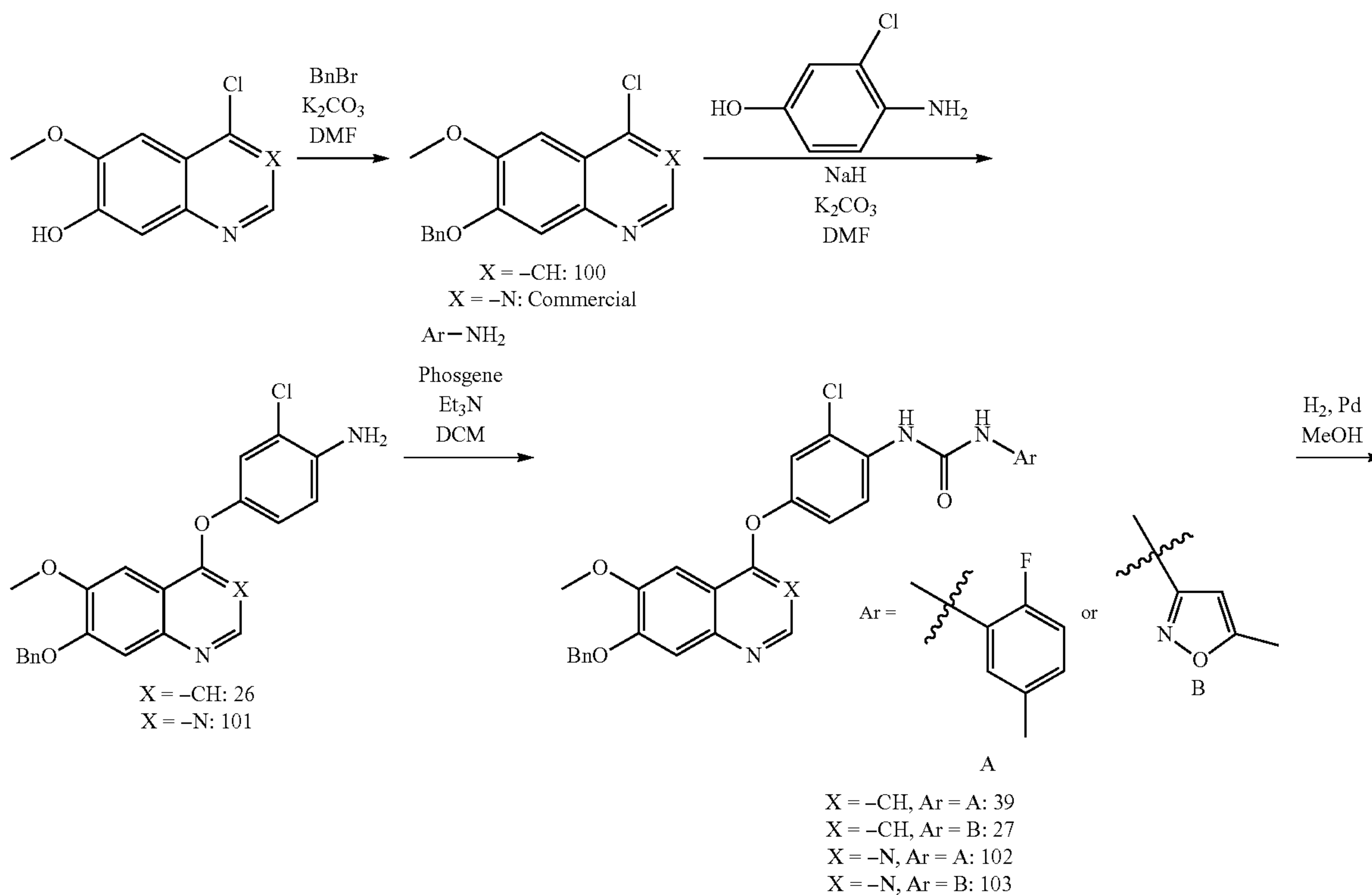
Scheme 1
