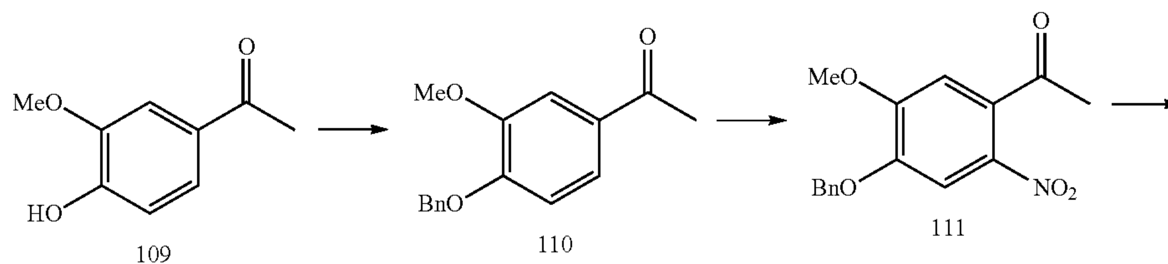
Scheme 2
