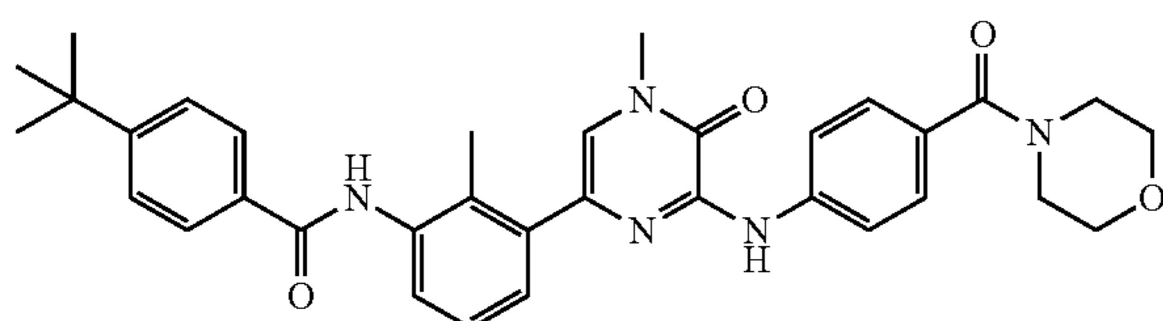
CGI-1746
