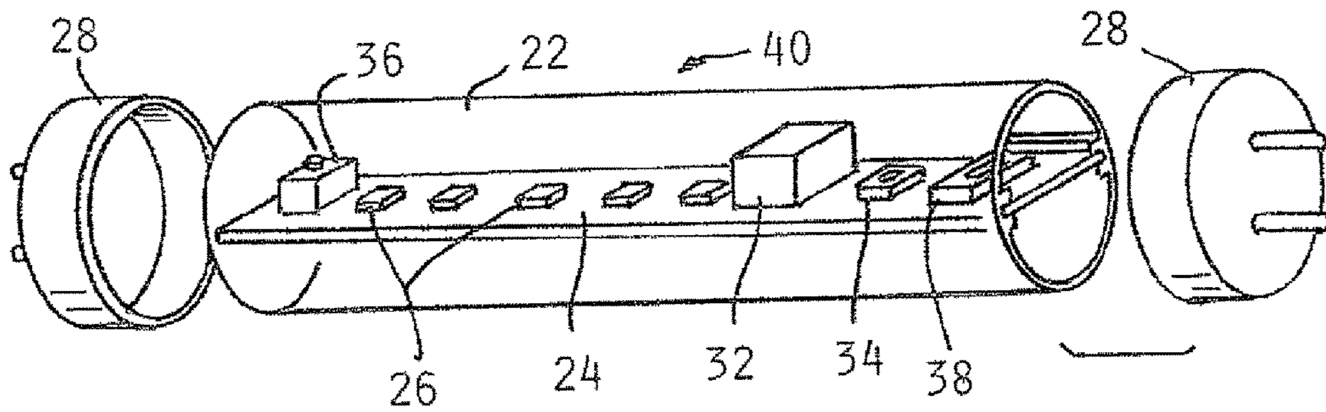
FIG. 2 (PRIOR ART)
