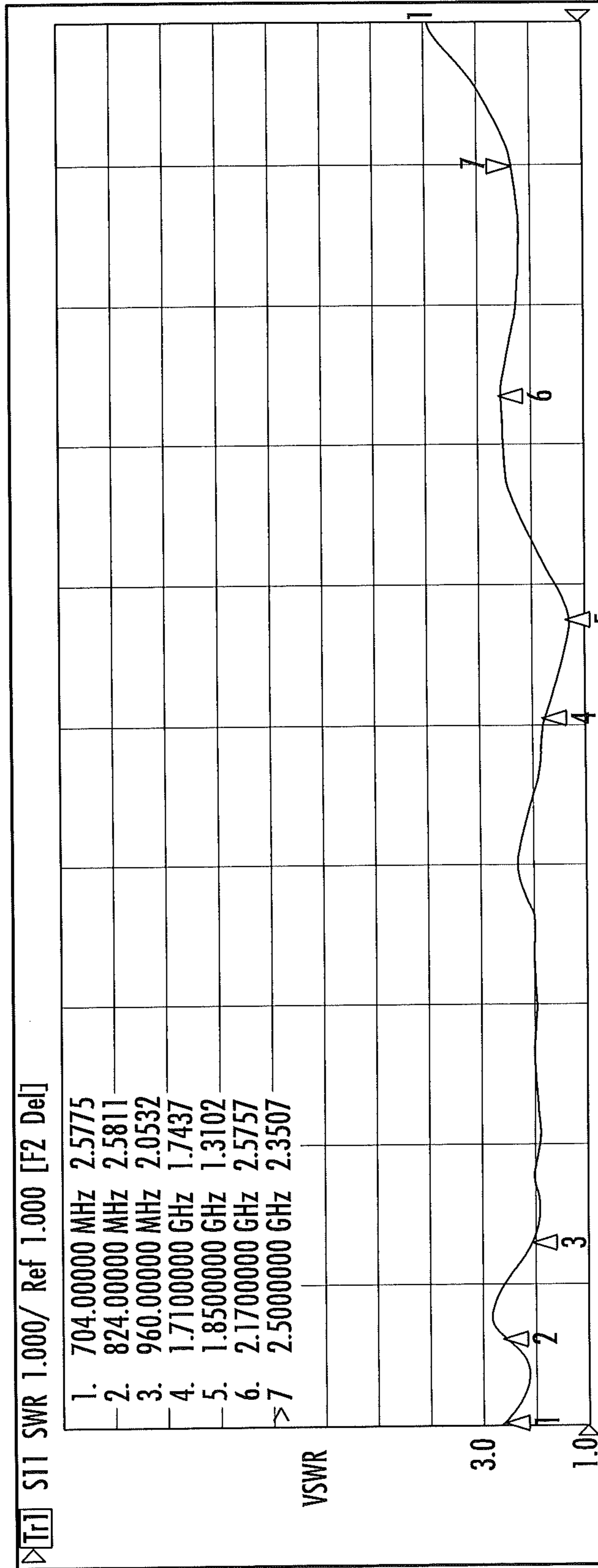
FIG. 8A (PRIOR ART)
