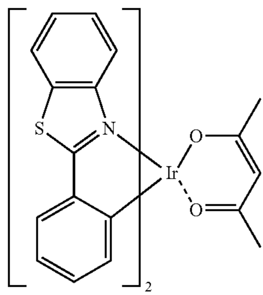
Ir(BT) 2 (acac)
