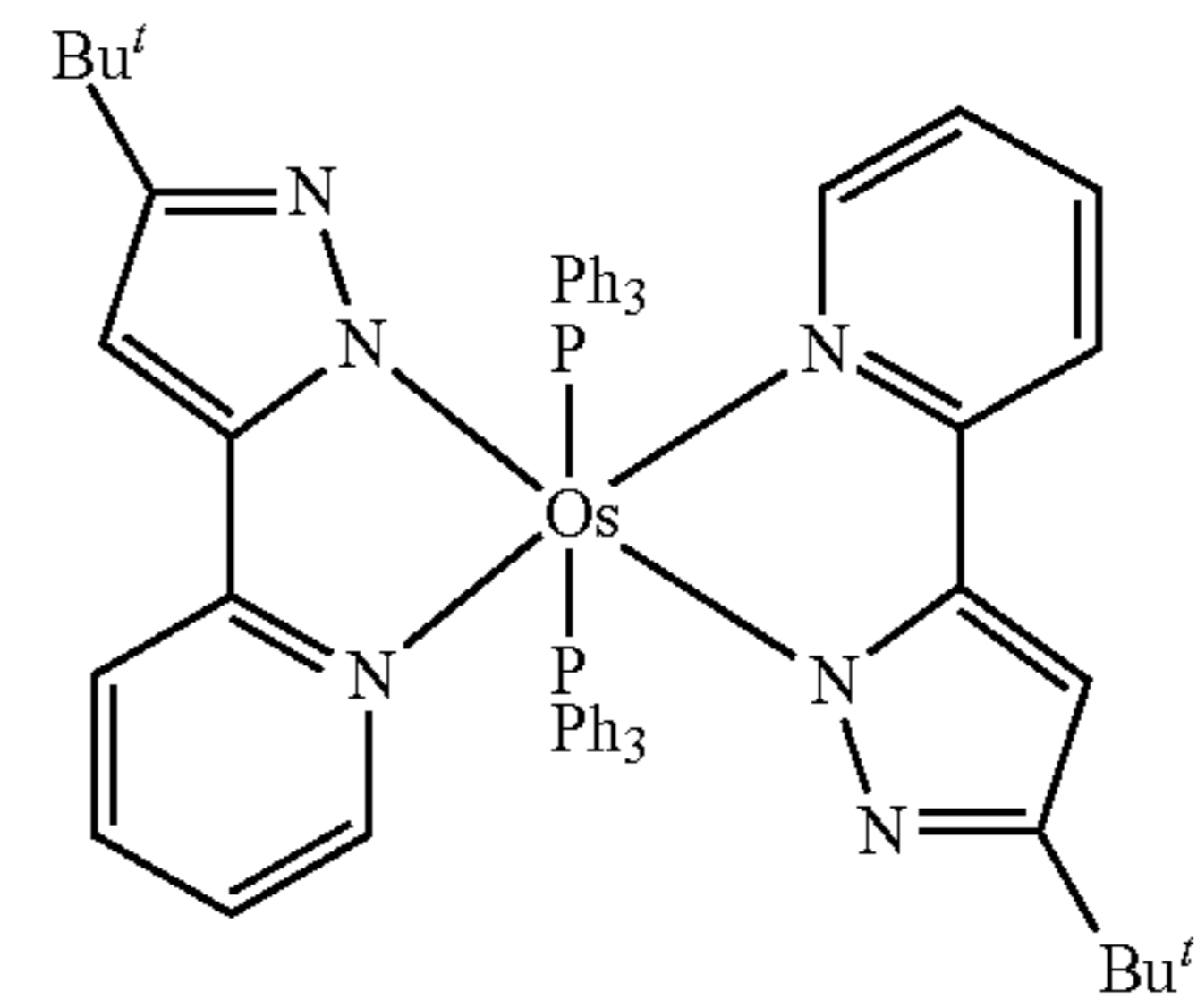
Os(bppz) 2 (PPh 3 ) 2
