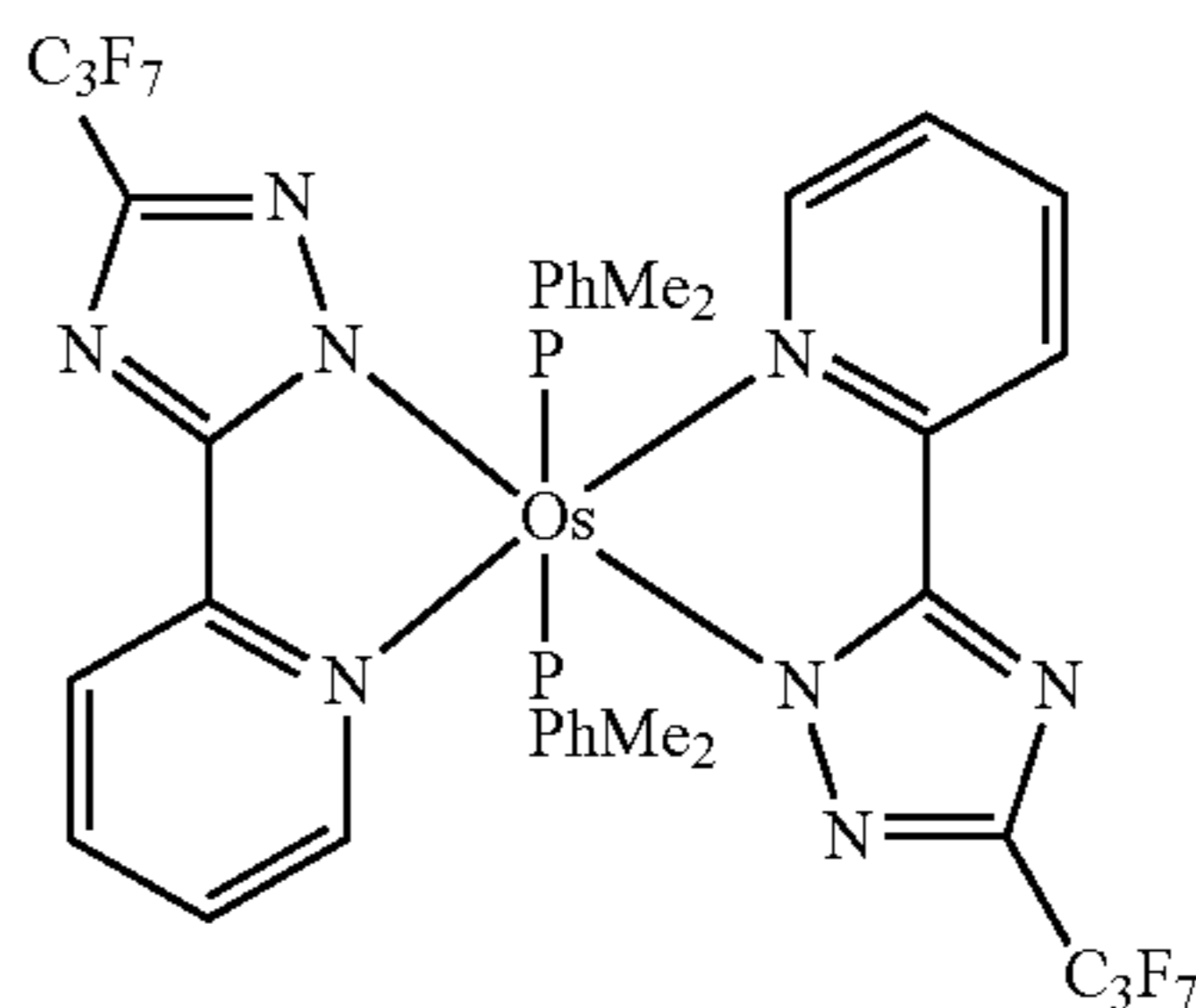
Os(bptz) 2 (PPhMe 2 ) 2
