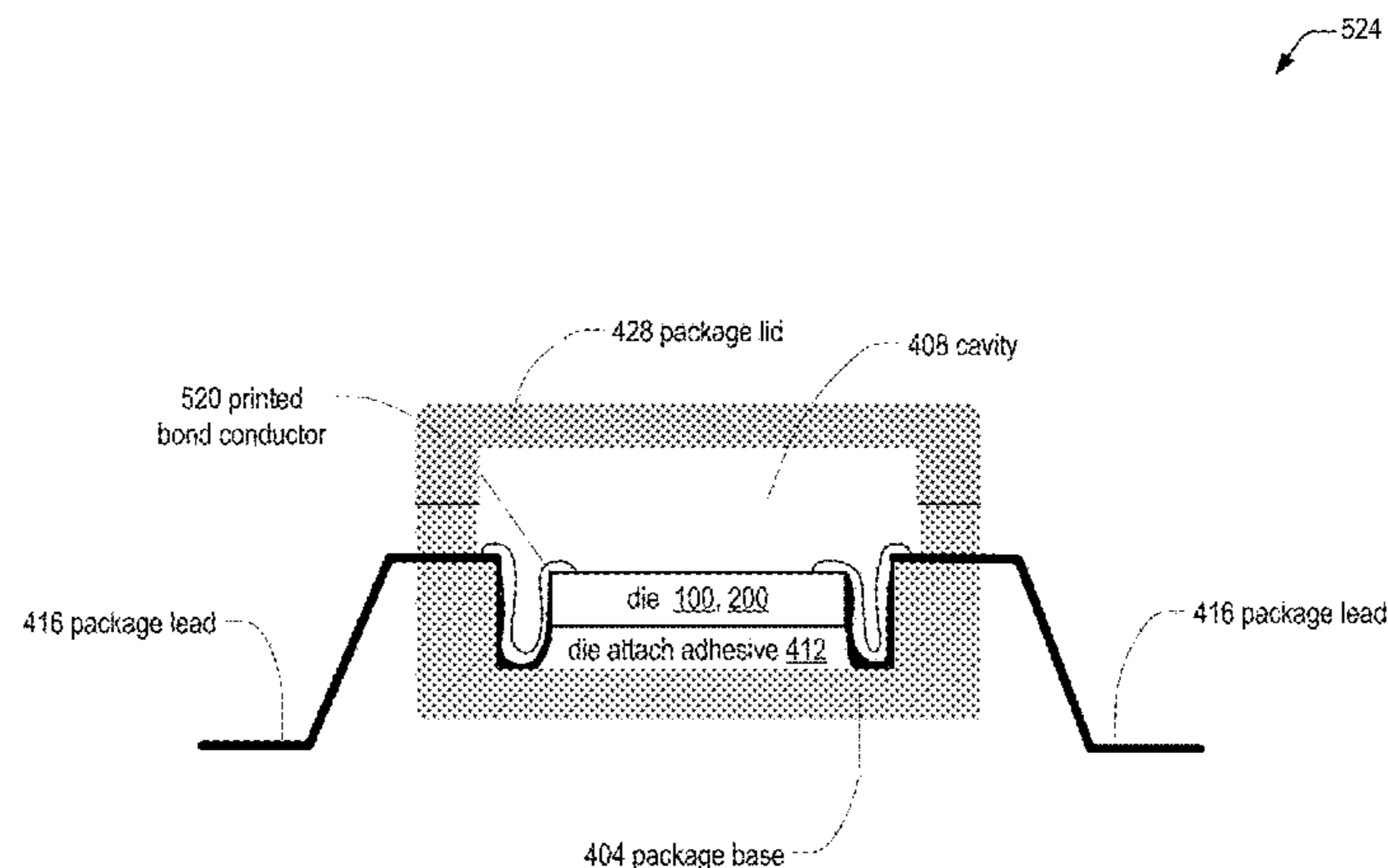
Packaged integrated circuit using printed bond conductors
