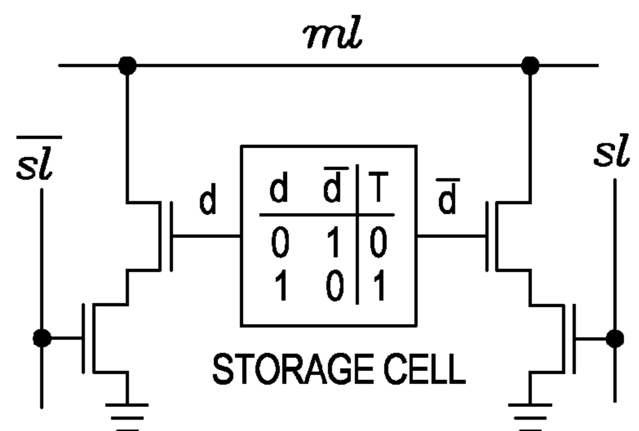
BINARY CAM CELL
