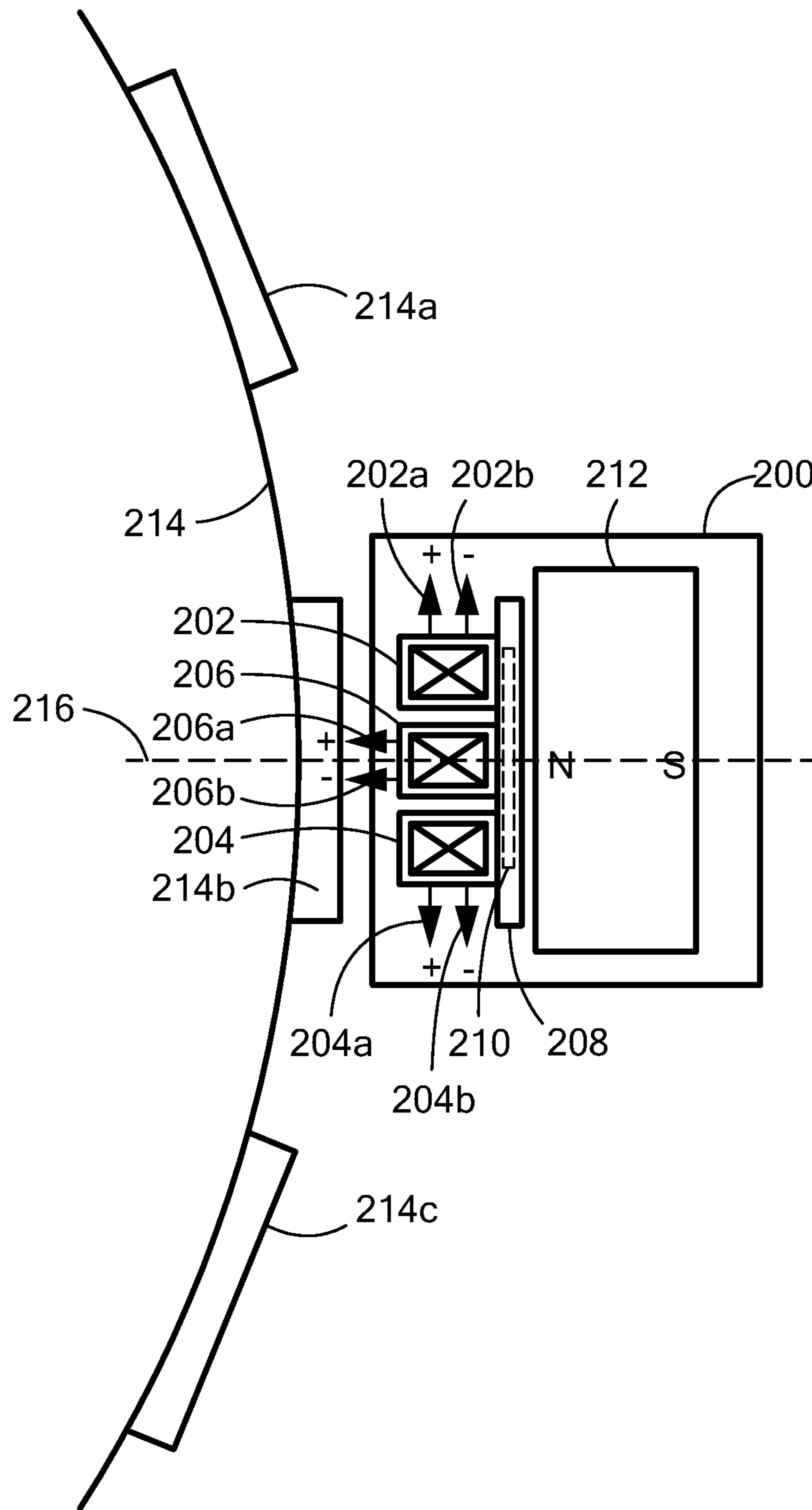
FIG. 2 PRIOR ART
