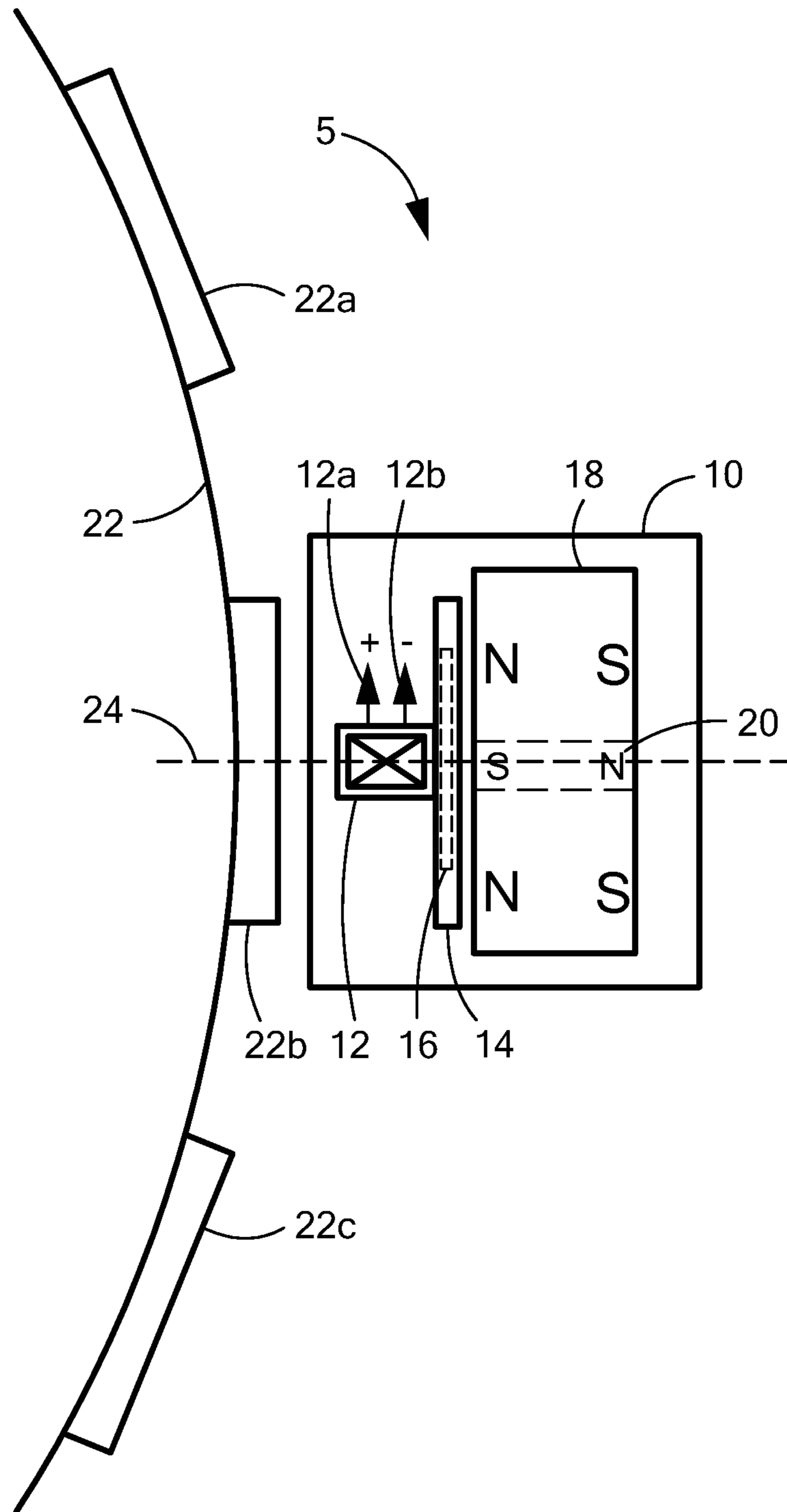
FIG. 1 PRIOR ART
