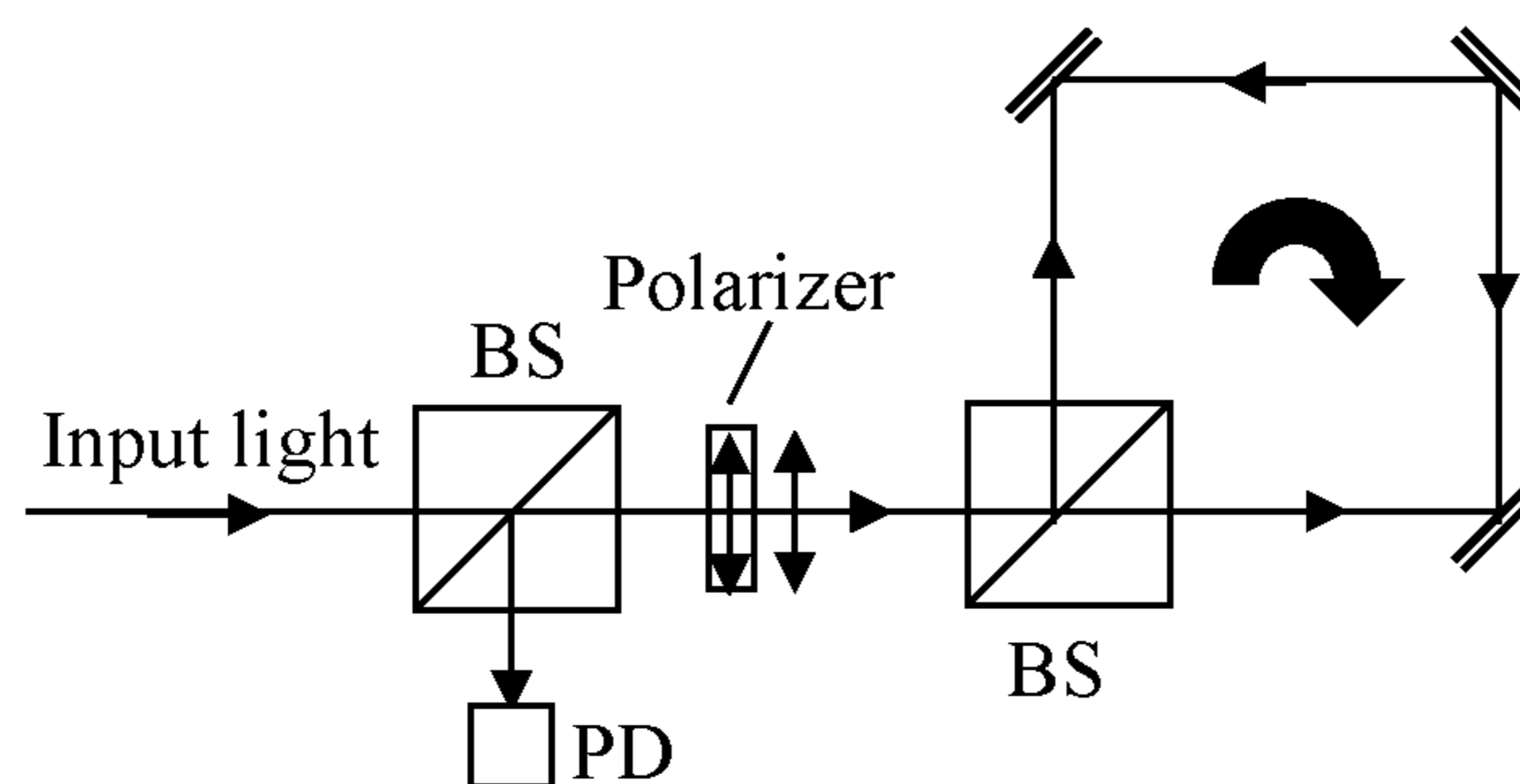
FIG. 1 (Prior Art)
