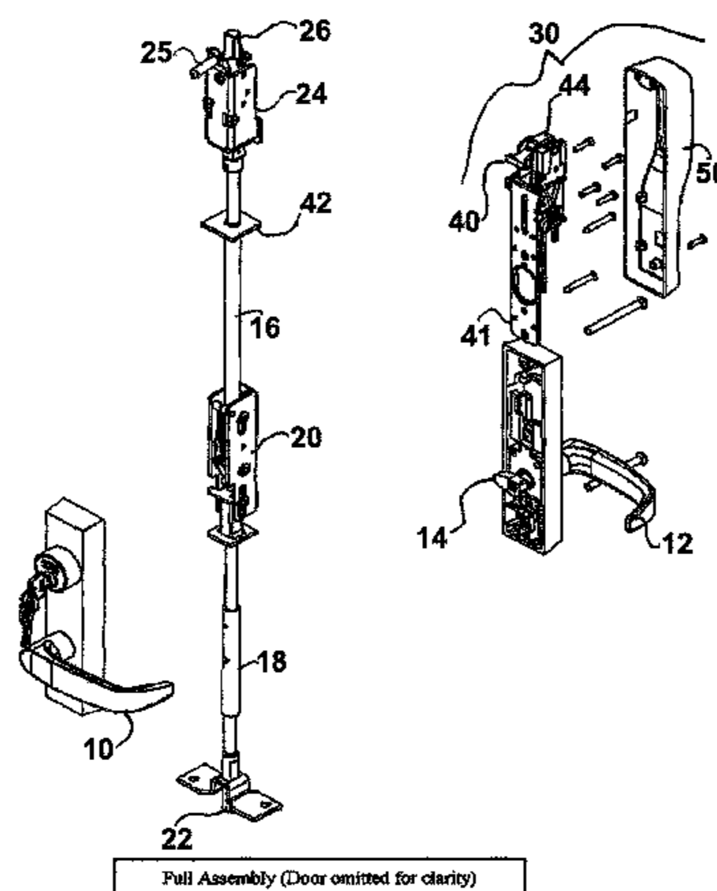
Full Assembly (Door omitted for clarity)
