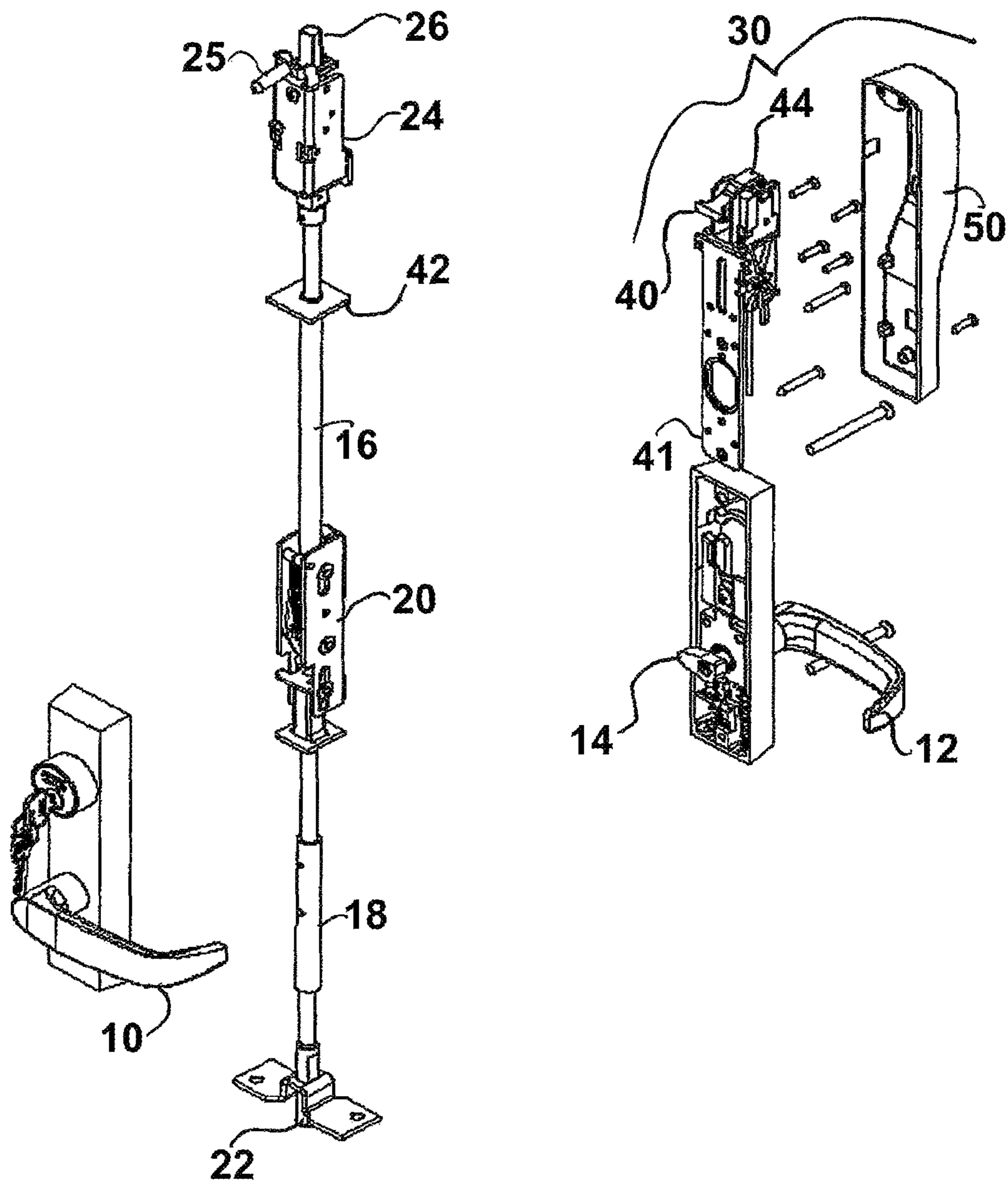
Full Assembly (Door omitted for clarity)
