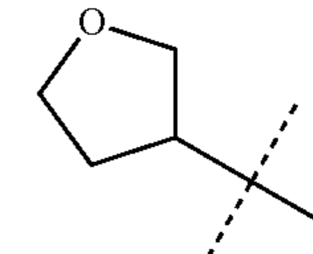
Tetrahydrofuran-3-yl
