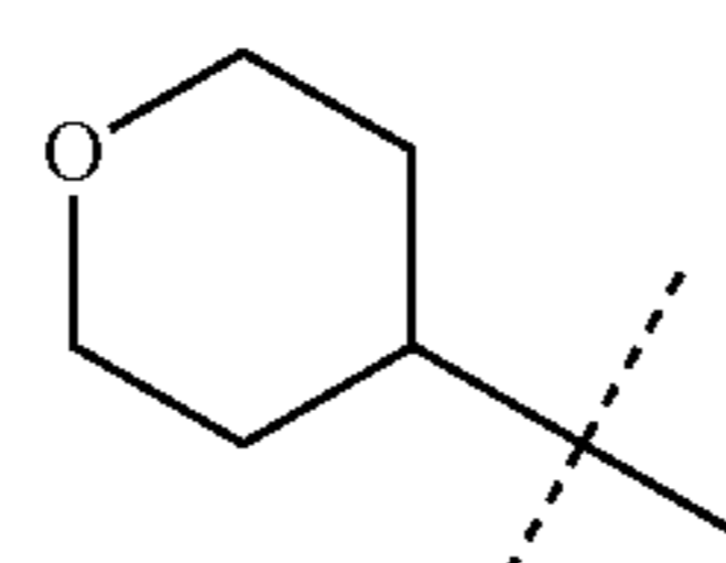
Oxan-4-yl
