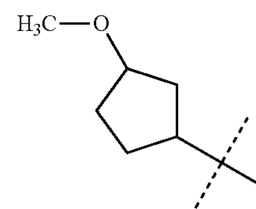
1-methoxycyclopent-3-yl/3-methoxycyclopent-1-yl
