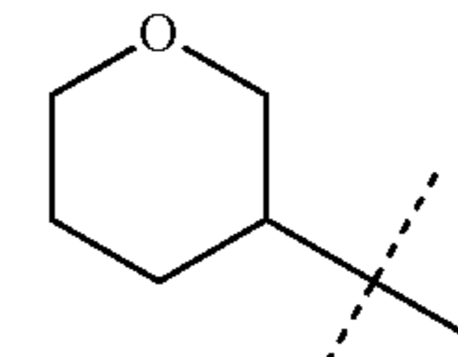
Oxan-3-yl
