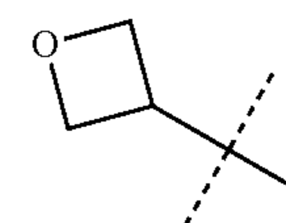
Oxtetan-3-yl
