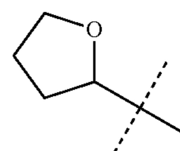
Tetrahydrofuran-2-yl
