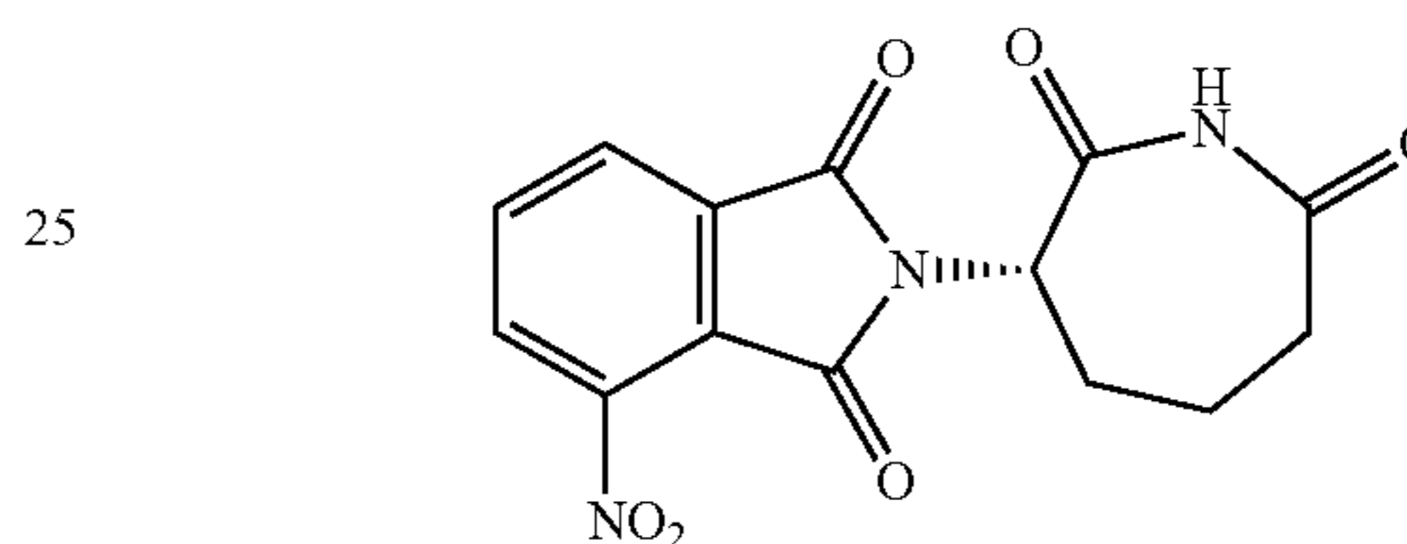
4-Nitro-2-[(3S)-2-oxoazepan-3-yl]isoindoline-1,3-dione (Compound 5)
