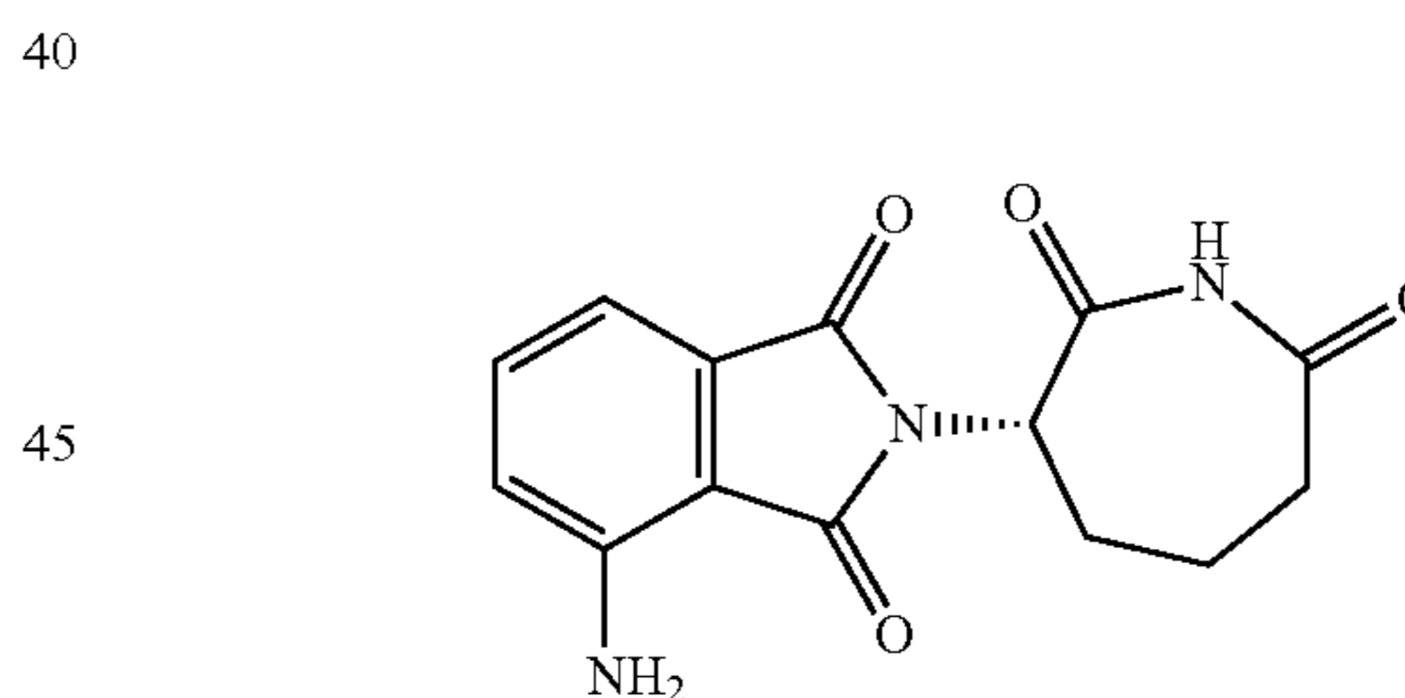
4-Amino-2-[(3S)-2,7-dioxoazepan-3-yl]isoindoline-1,3-dione (Compound 10)
