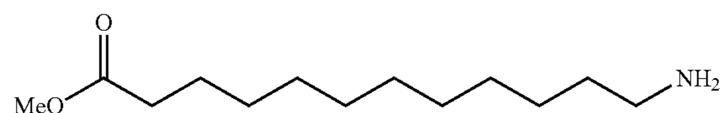
C_{13}H_{27}NO_2 Exact Mass: 229.2 Mol. Wt.: 229.36
