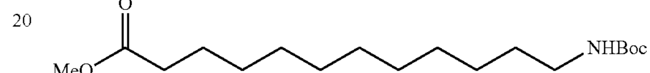
C_{18}H_{35}NO_4 Exact Mass: 329.26 Mol. Wt.: 329.47
