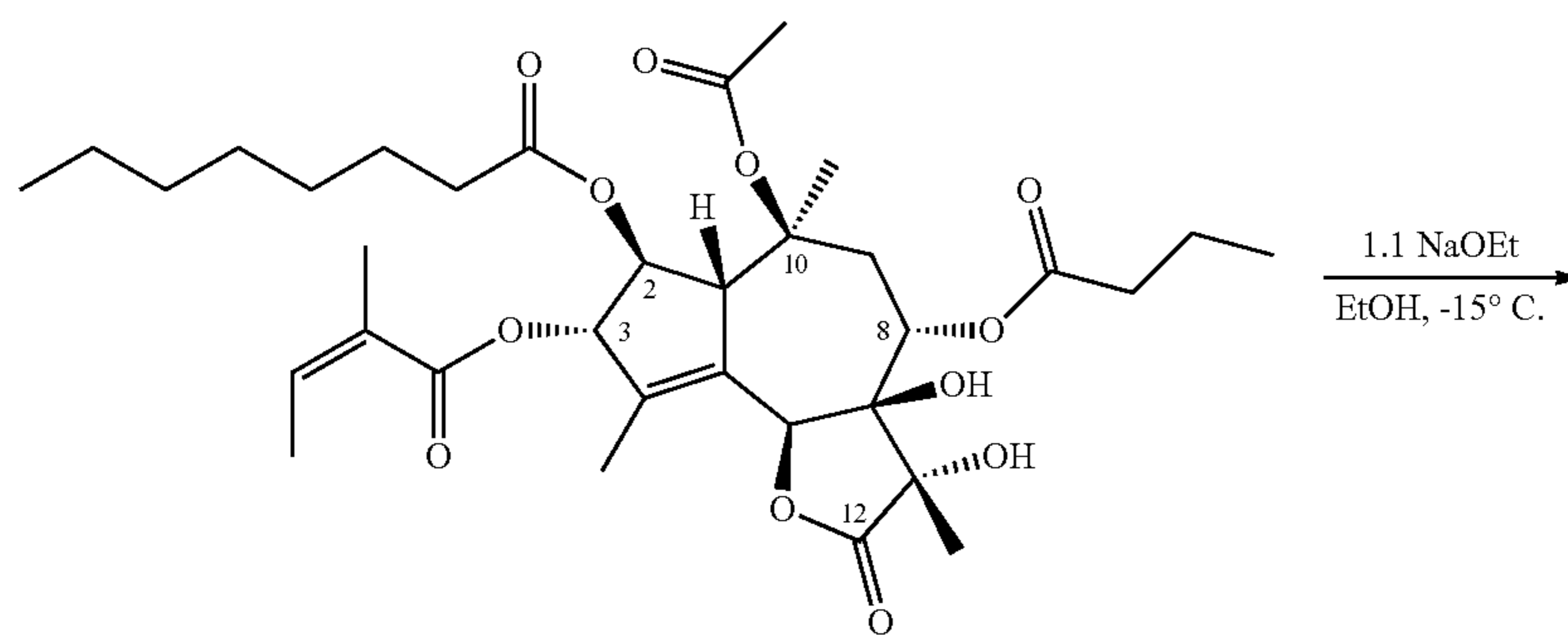
Thapsigargin (Tg) C 34 H 50 O 12 Mol. Wt.: 650.75
