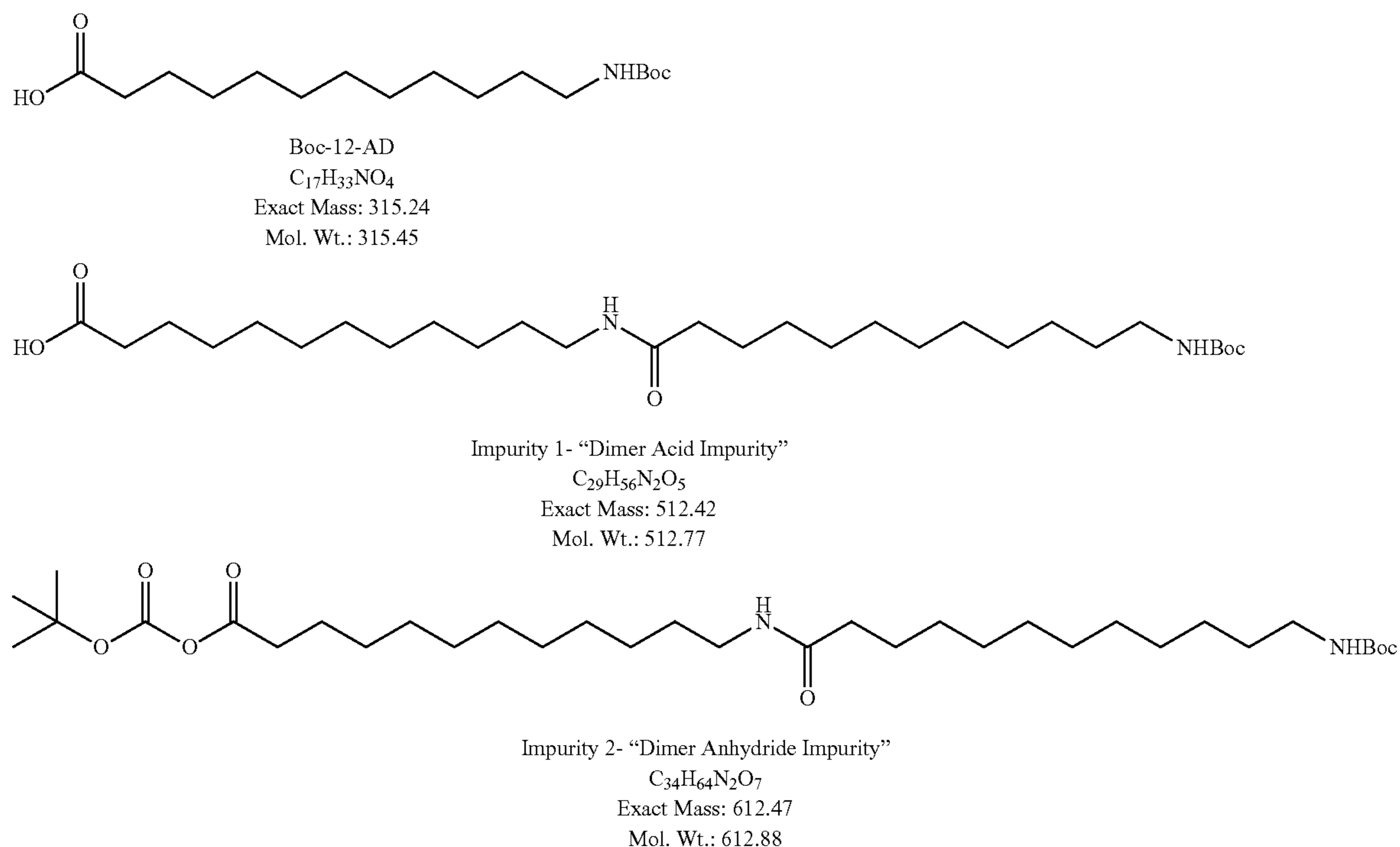
Scheme 2
