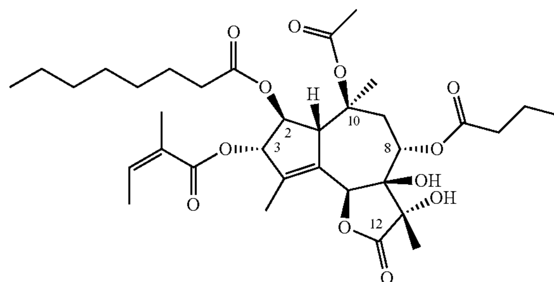
Thapsigargin (Tg) C 34 H 50 O 12 Mol. Wt.: 650.75
