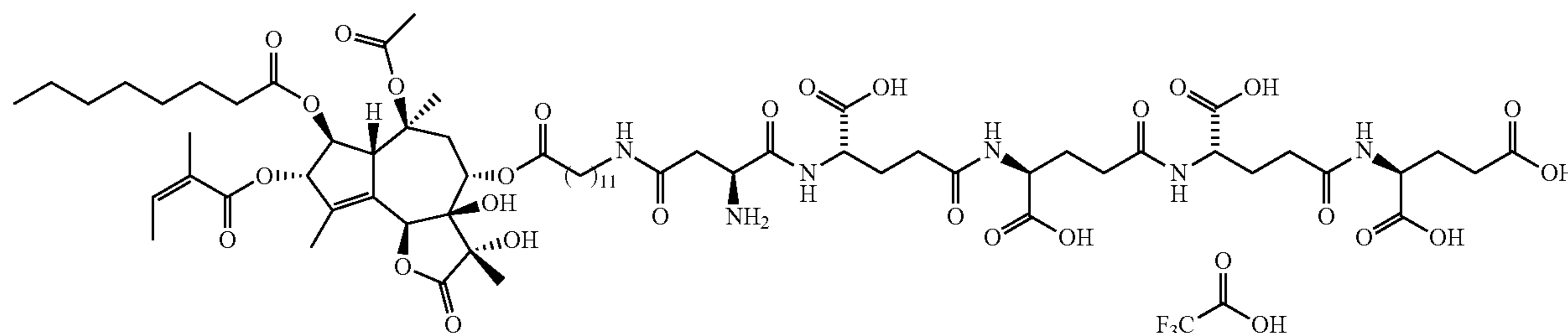
Crude G-202 Formula: \text{C}_{68}\text{H}_{101}\text{F}_3\text{N}_6\text{O}_{29} FW: 1523.55
