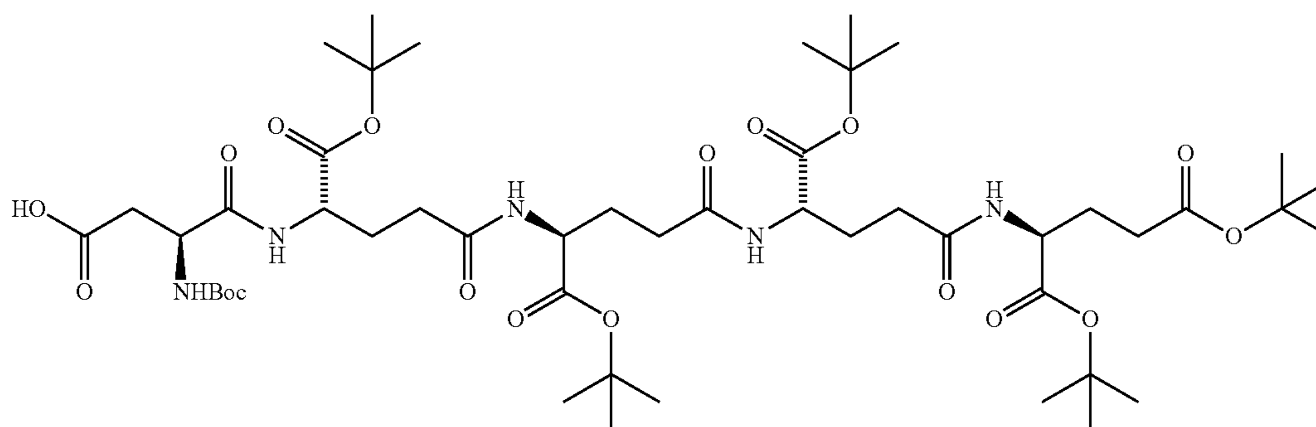
Boc-Asp-Glu(OtBu)-Glu(OtBu)-Glu(OtBu)-OtBu
