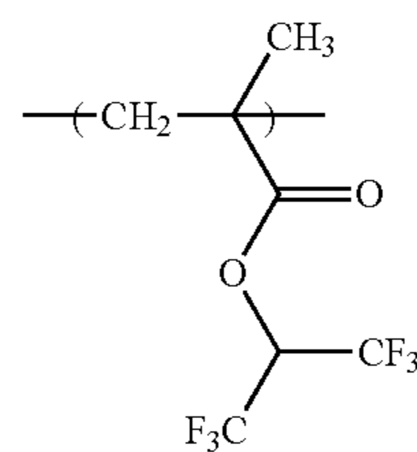
Example 7: Synthesis of Resin X4
