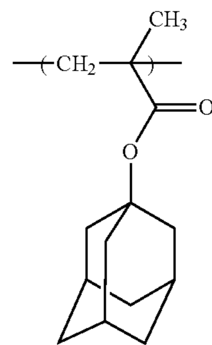
Example 8: Synthesis of Resin X5
