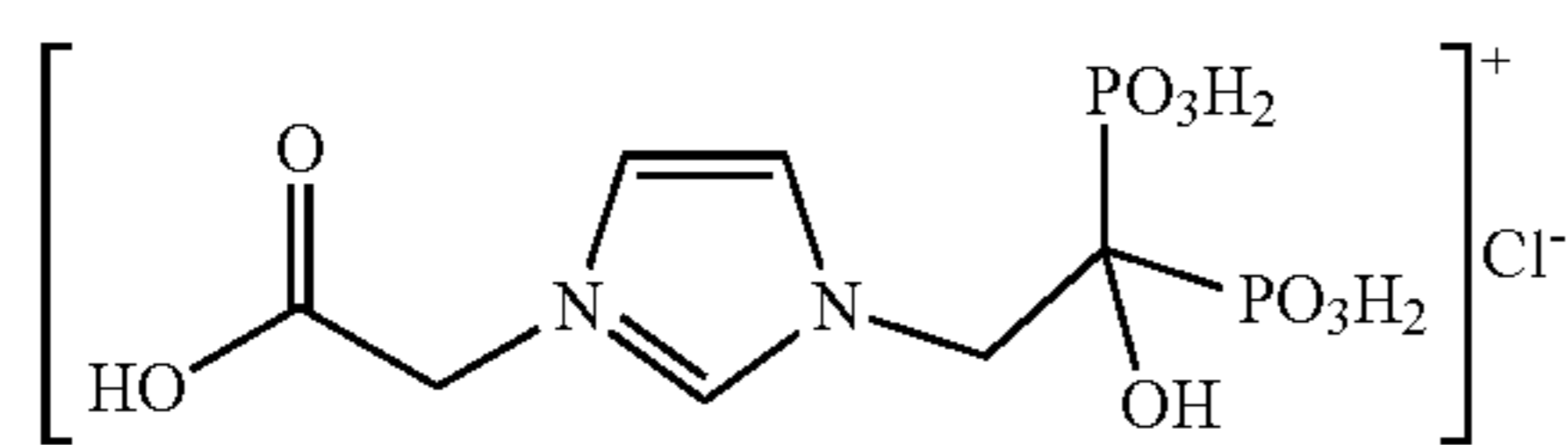
Compound 1
