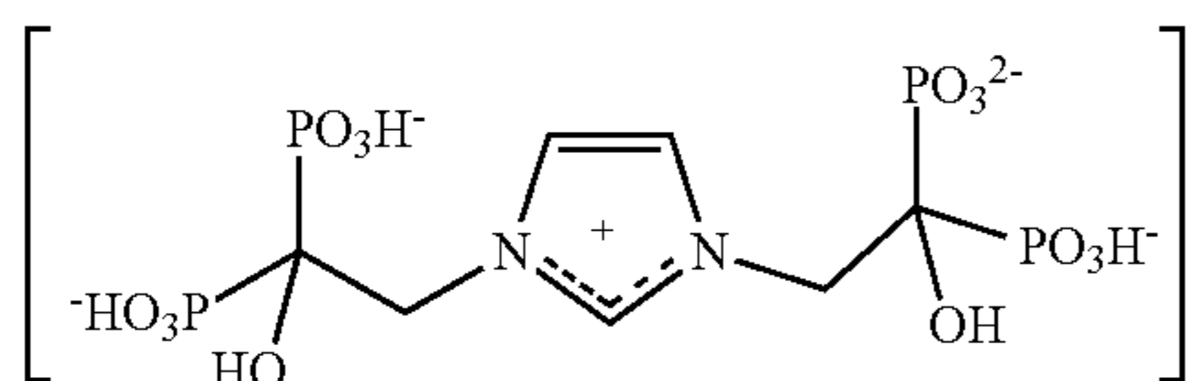
Na salt of Compound 2
