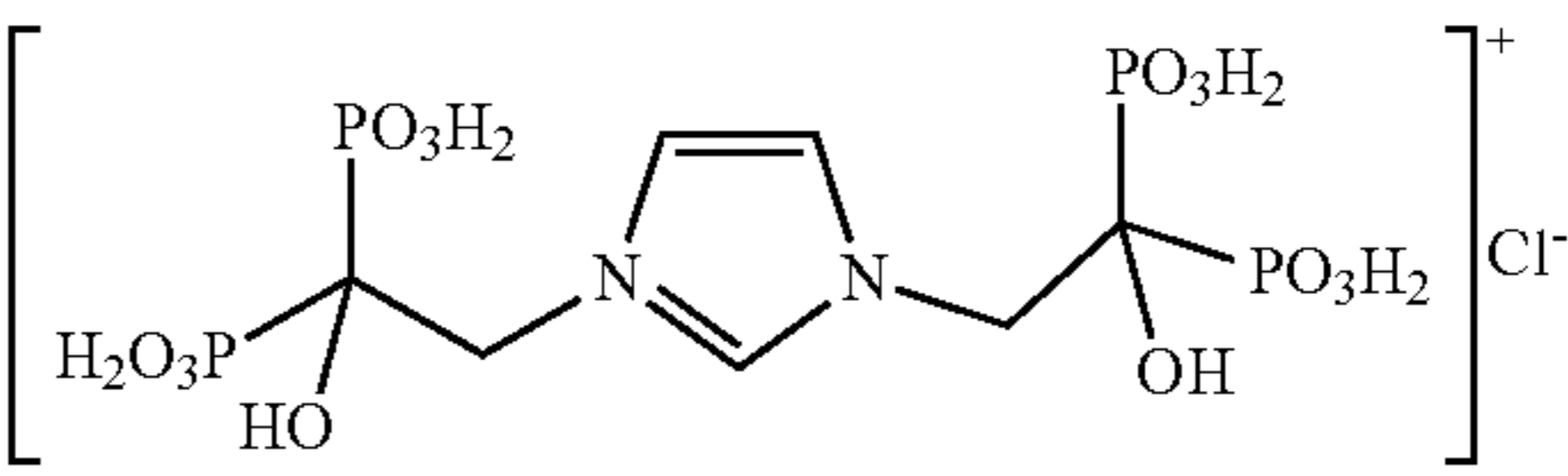
Compound 2
