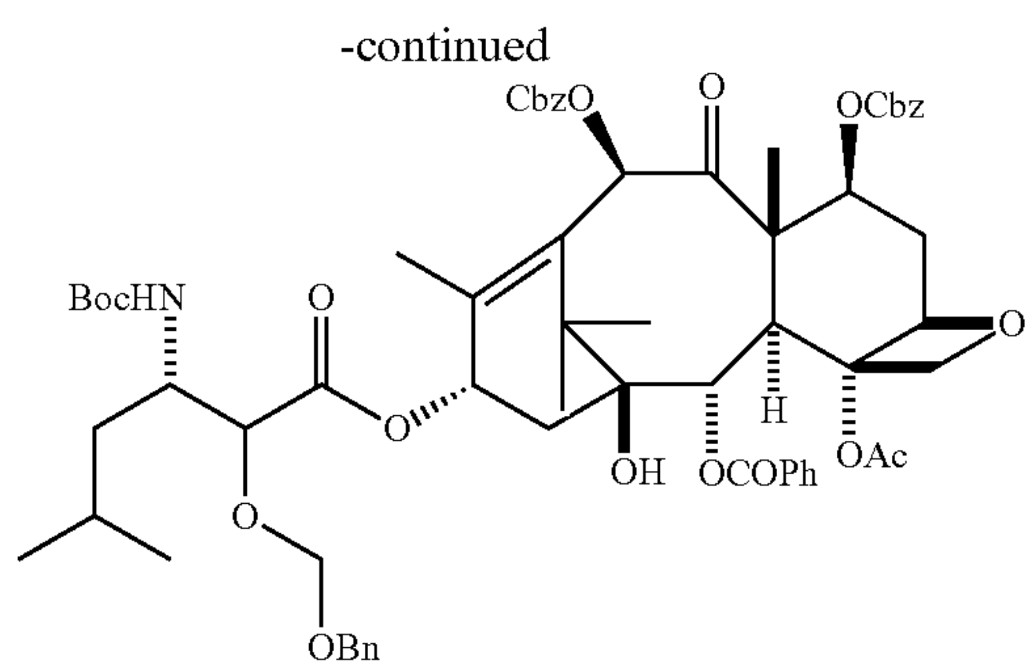
C_{65}H_{77}NO_{19} Mol. Wt.: 1176.3 Formula 37
