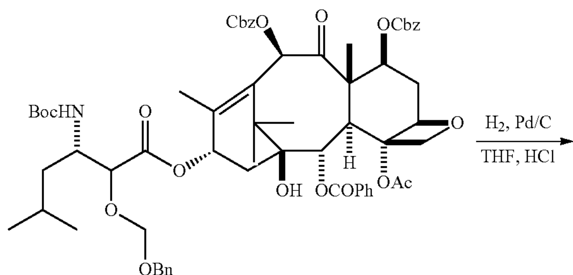
C_{65}H_{77}NO_{19} Mol. Wt.: 1176.3 Formula 37
