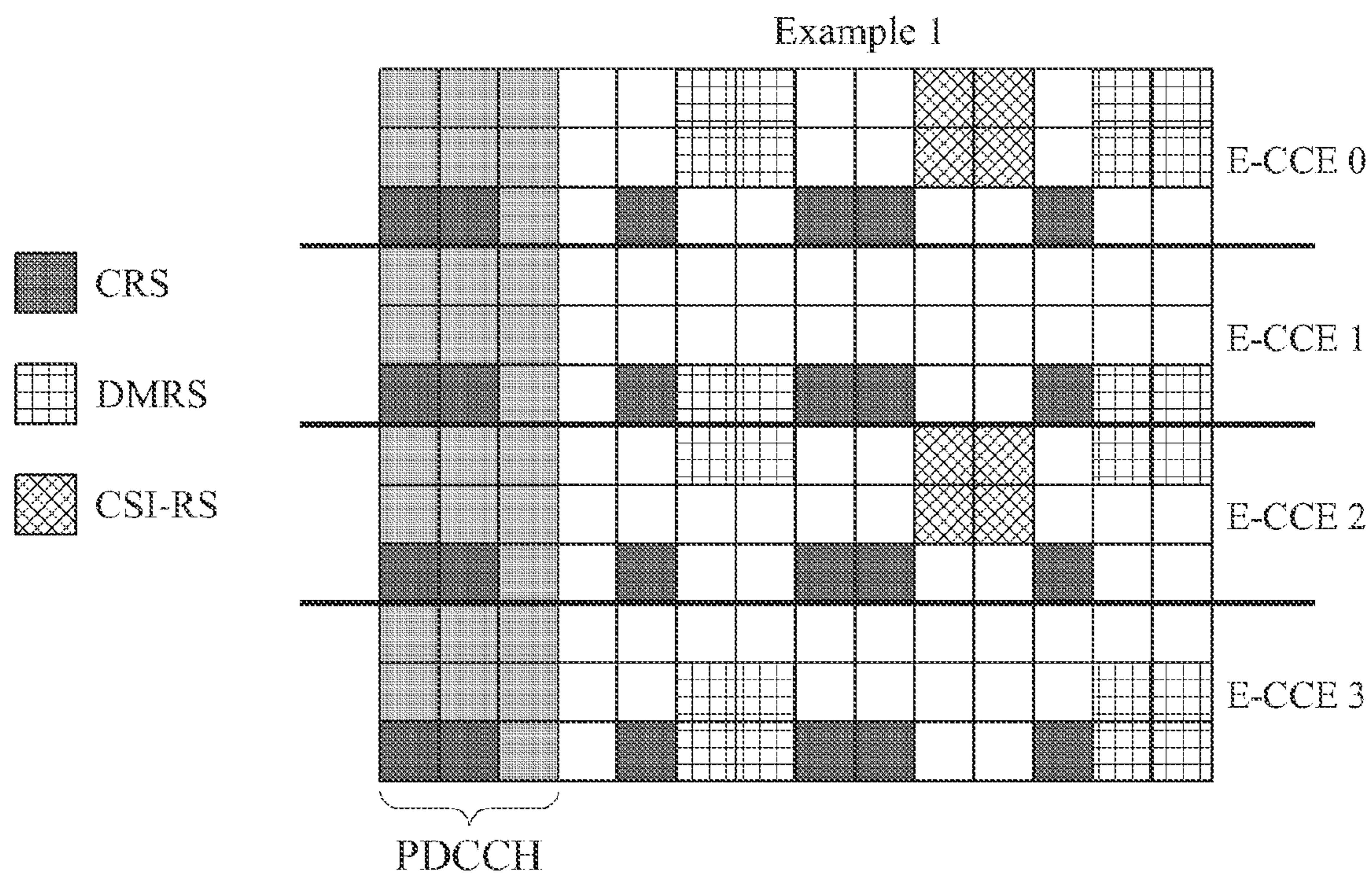
FIG. 3 (RELATED ART)
