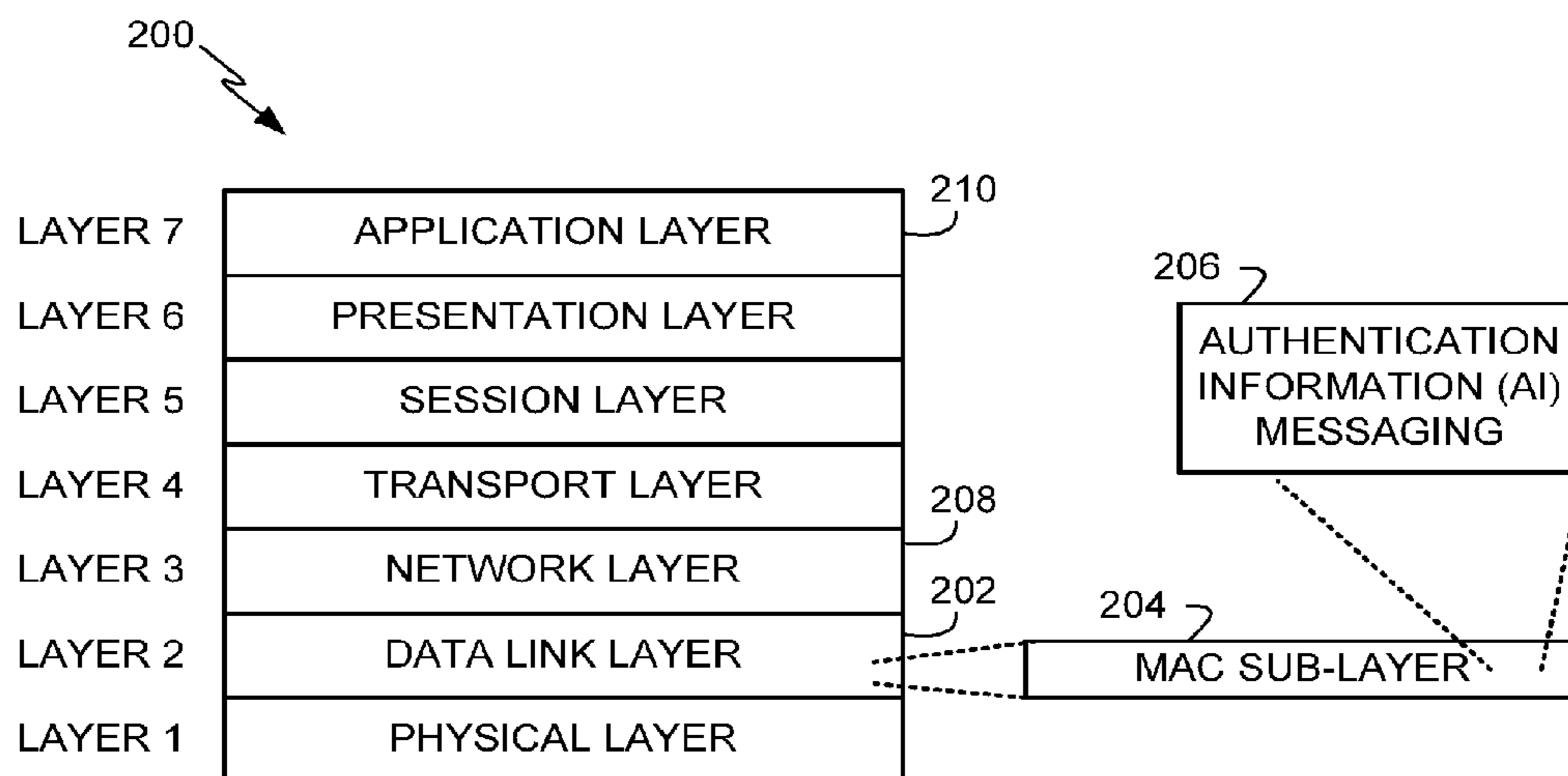
COMMUNICATION LAYER ARCHITECTURE
