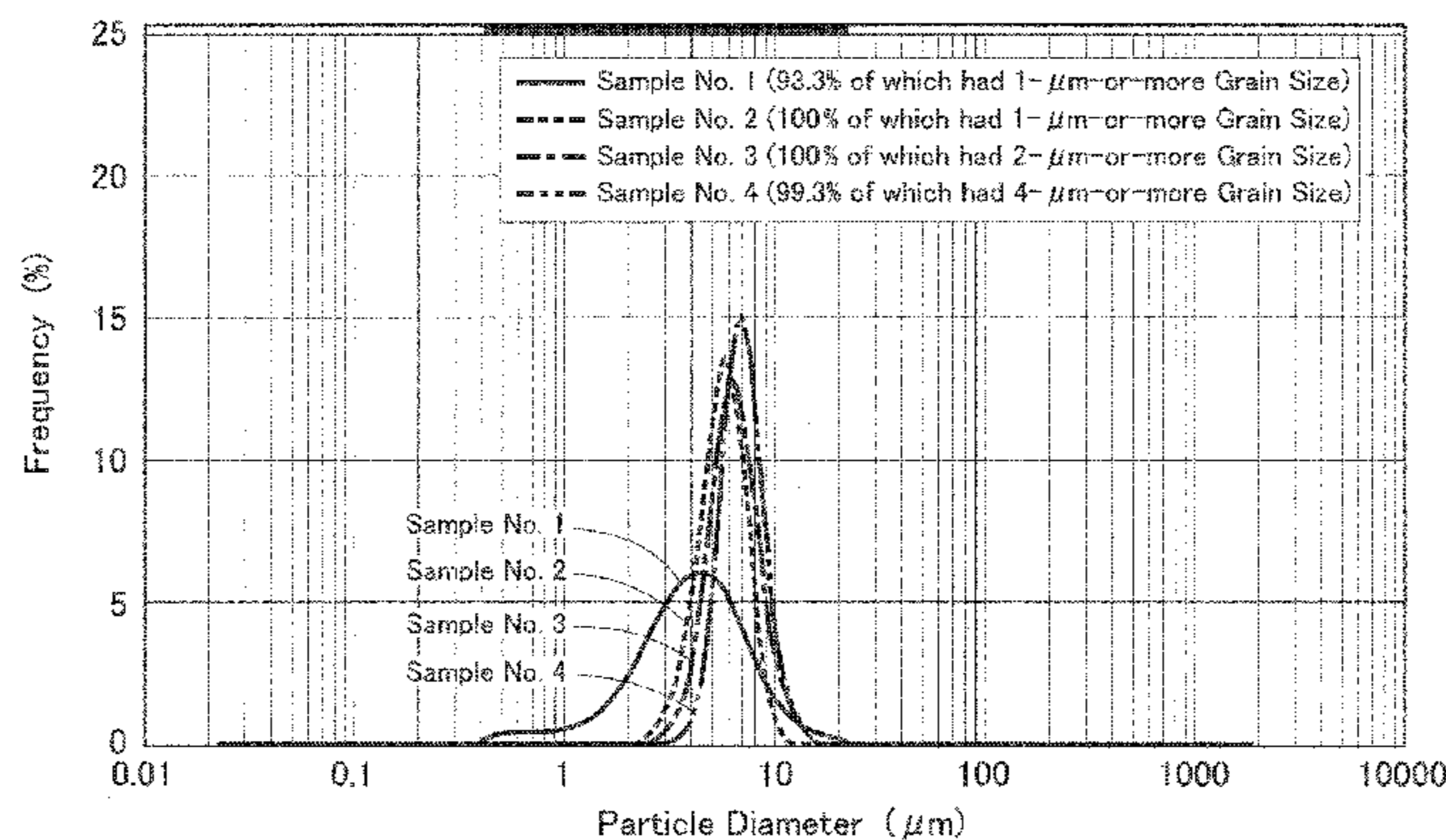
Grain-size Distribution
