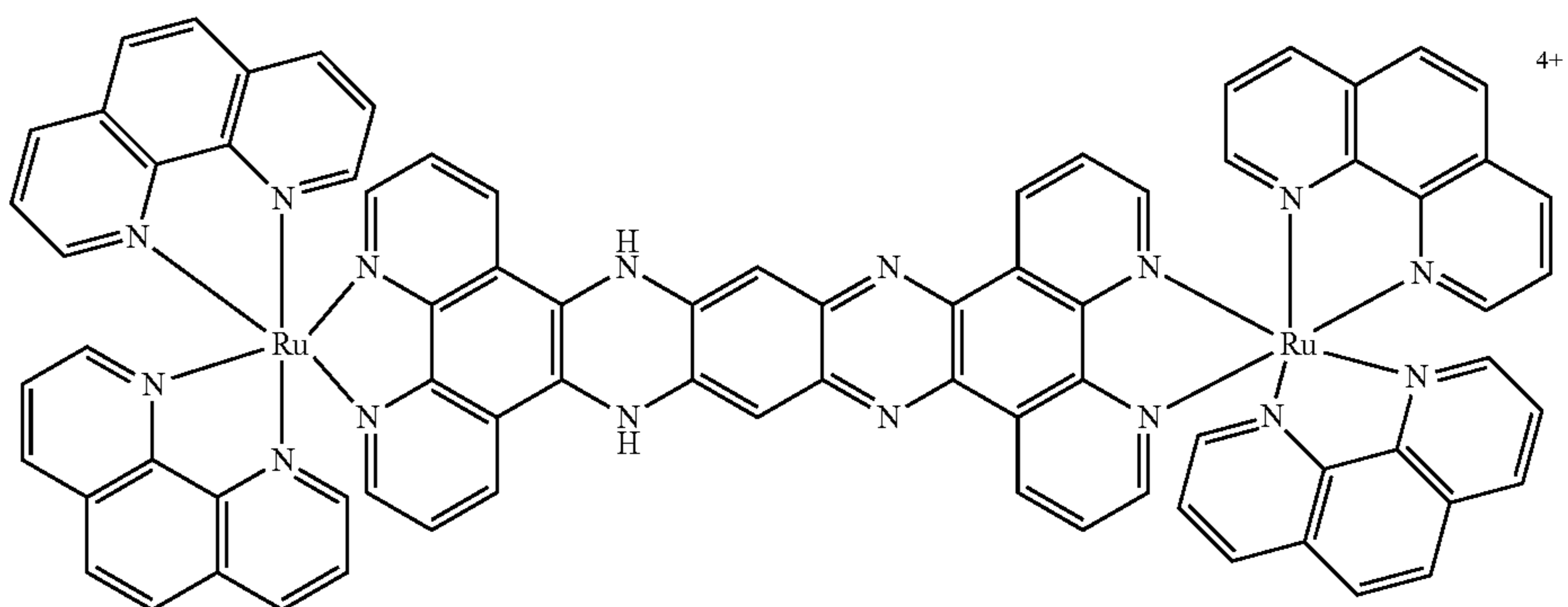
Scheme 6.
