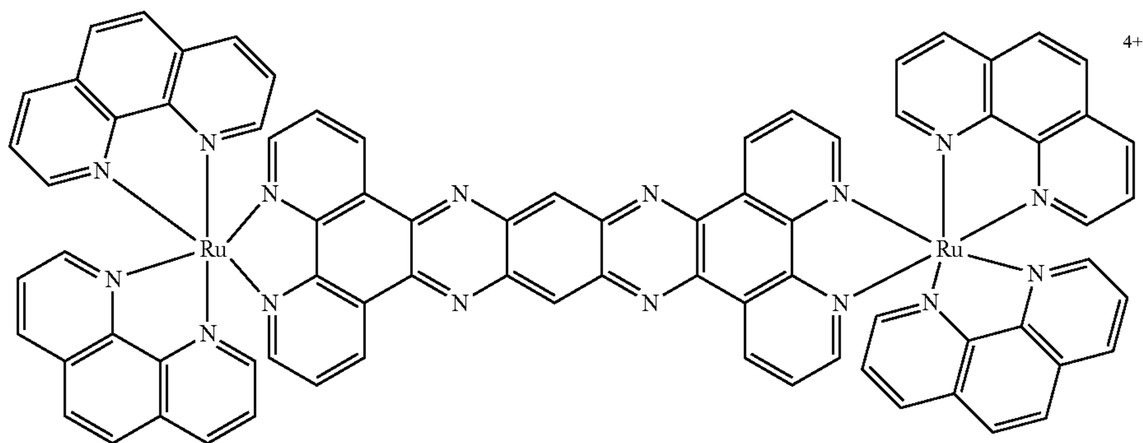
Scheme 4.
