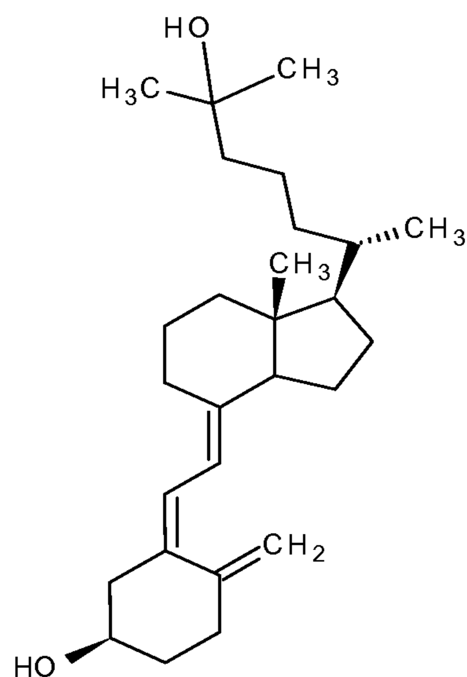
3-epi-25-hydroxyvitamin D 3
