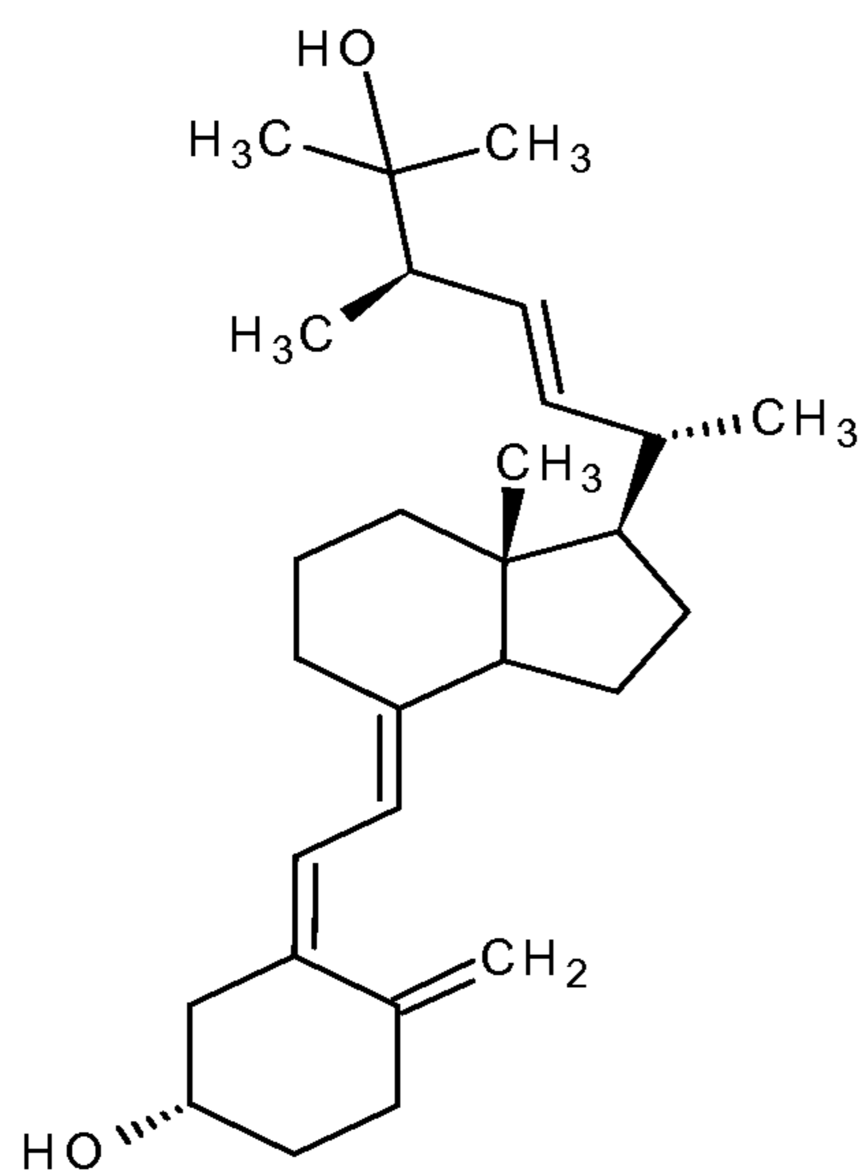
25-hydroxyvitamin D 2
