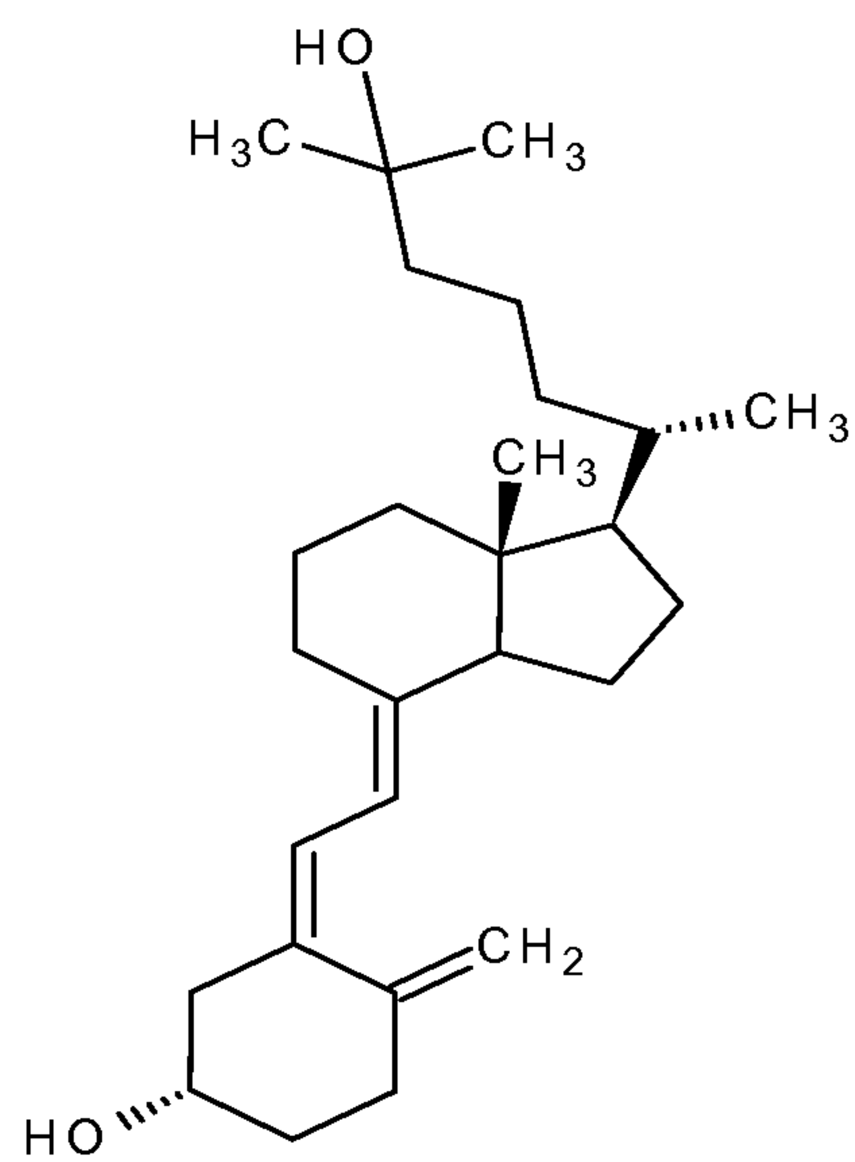
25-hydroxyvitamin D 3
