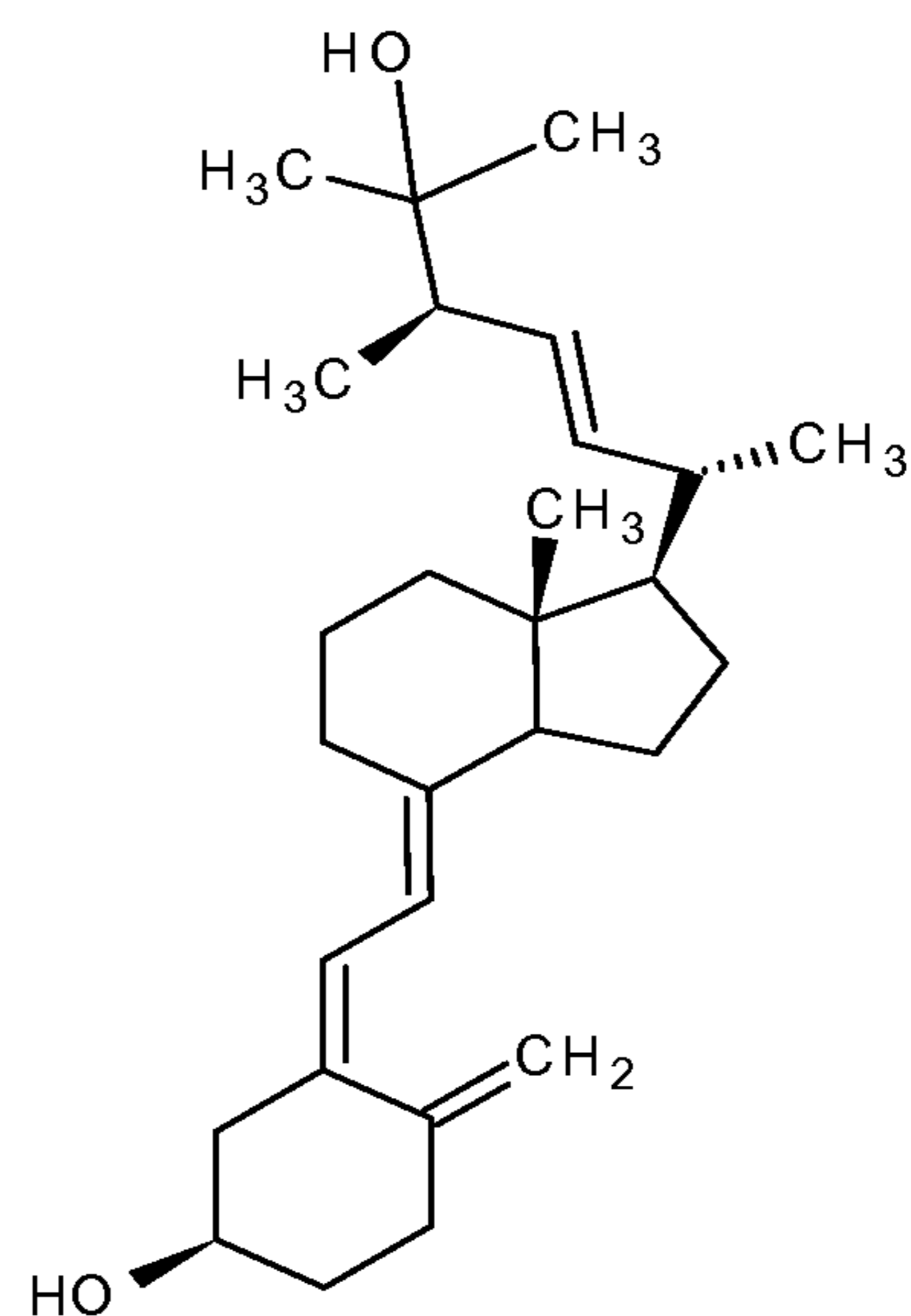
3-epi-25-hydroxyvitamin D 2
