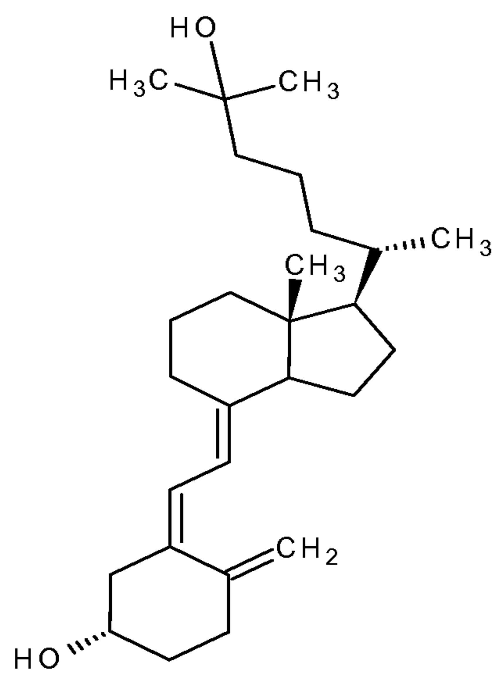
25-hydroxyvitamin D 3
