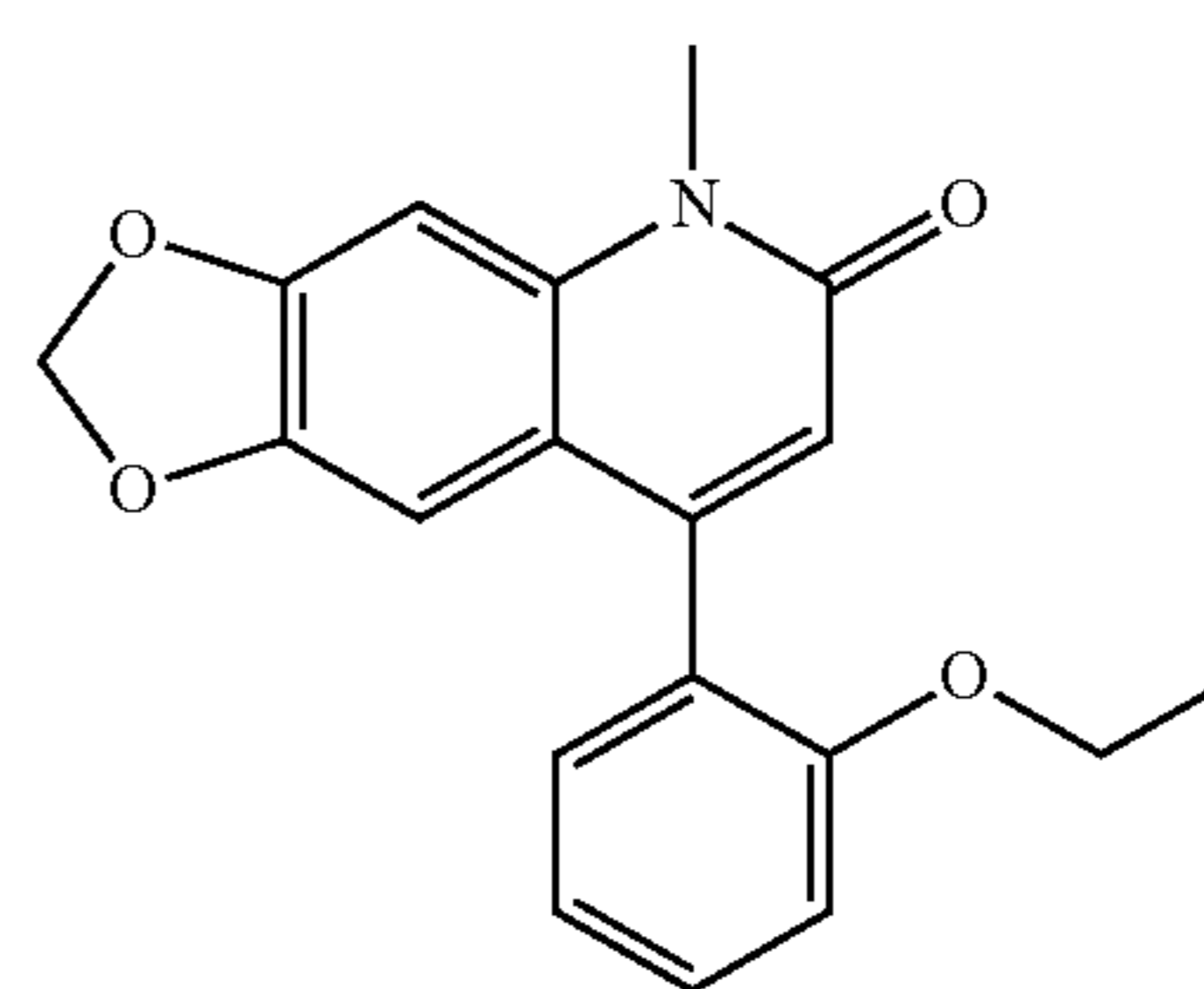
C1-NCH3
