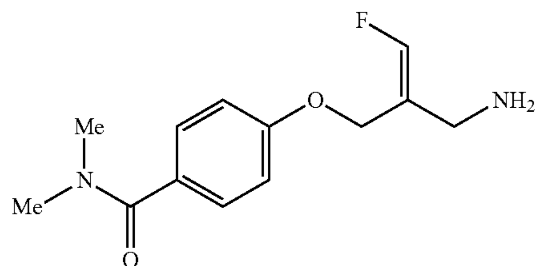
(Z)-4-(2-(Aminomethyl)-3-fluoroallyloxy)-N,N-dimethylbenzamide
