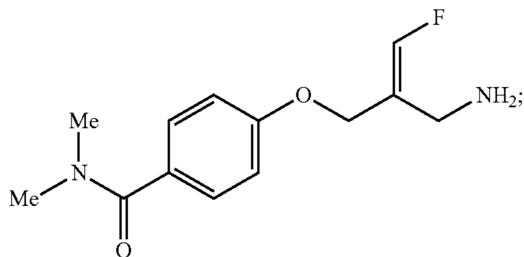
(E)-4-(2-(Aminomethyl)-3-fluoroallyloxy)-N,N-dimethylbenzamide
