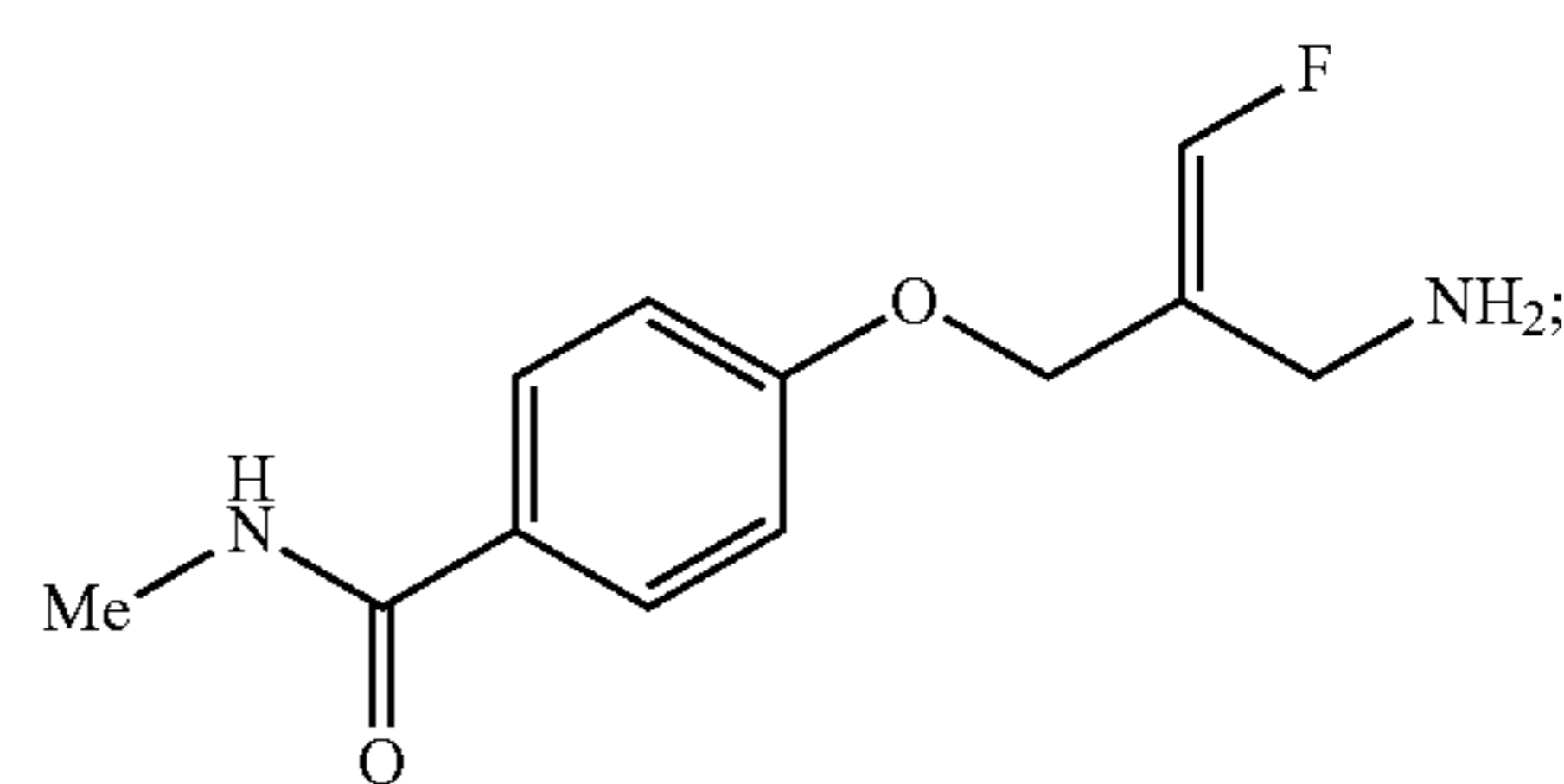
(E)-4-(2-(Aminomethyl)-3-fluoroallyloxy)-N-methylbenzamide
