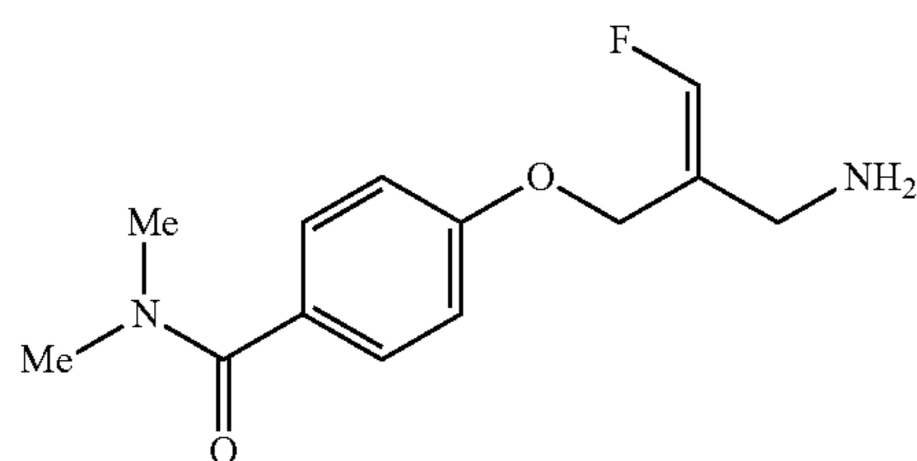
(Z)-4-(2-(Aminomethyl)-3-fluoroallyloxy)-N,N-dimethylbenzamide
