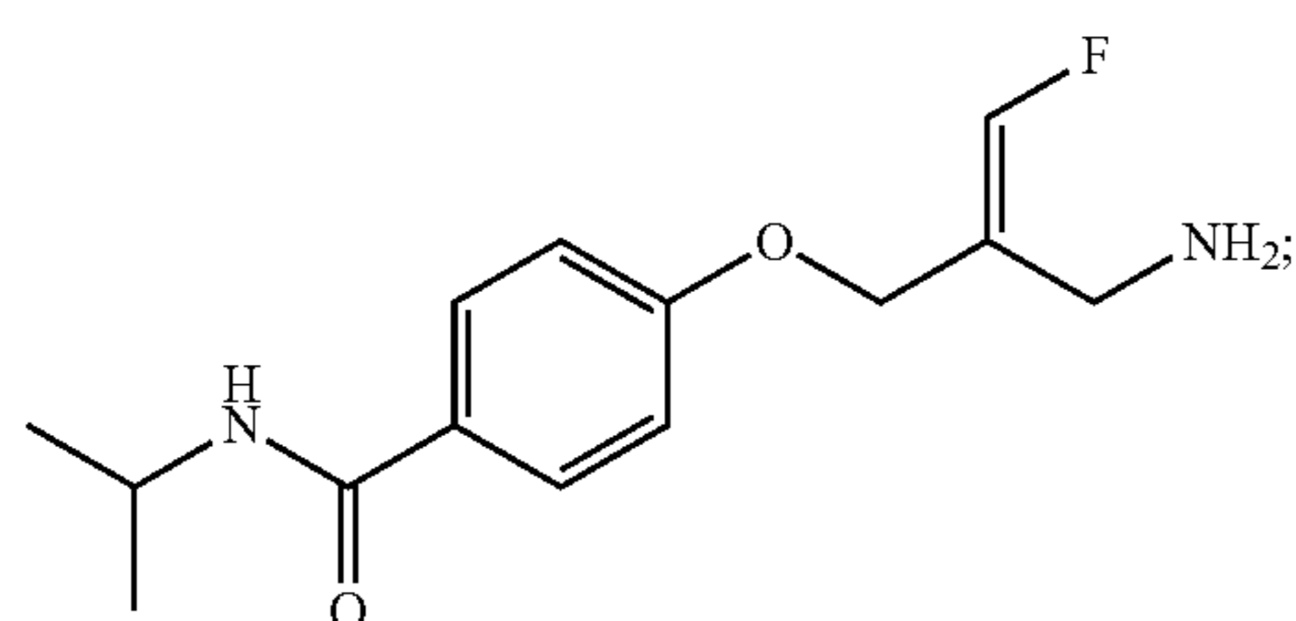
(E)-4-(2-(Aminomethyl)-3-fluoroallyloxy)-N-isopropylbenzamide
