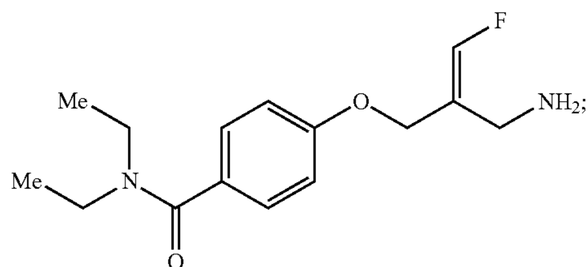
(E)-4-(2-(Aminomethyl)-3-fluoroallyloxy)-N,N-diethylbenzamide
