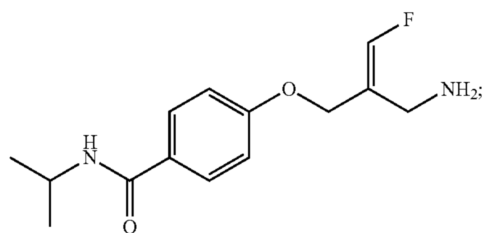
(E)-4-(2-(Aminomethyl)-3-fluoroallyloxy)-N-isopropylbenzamide
