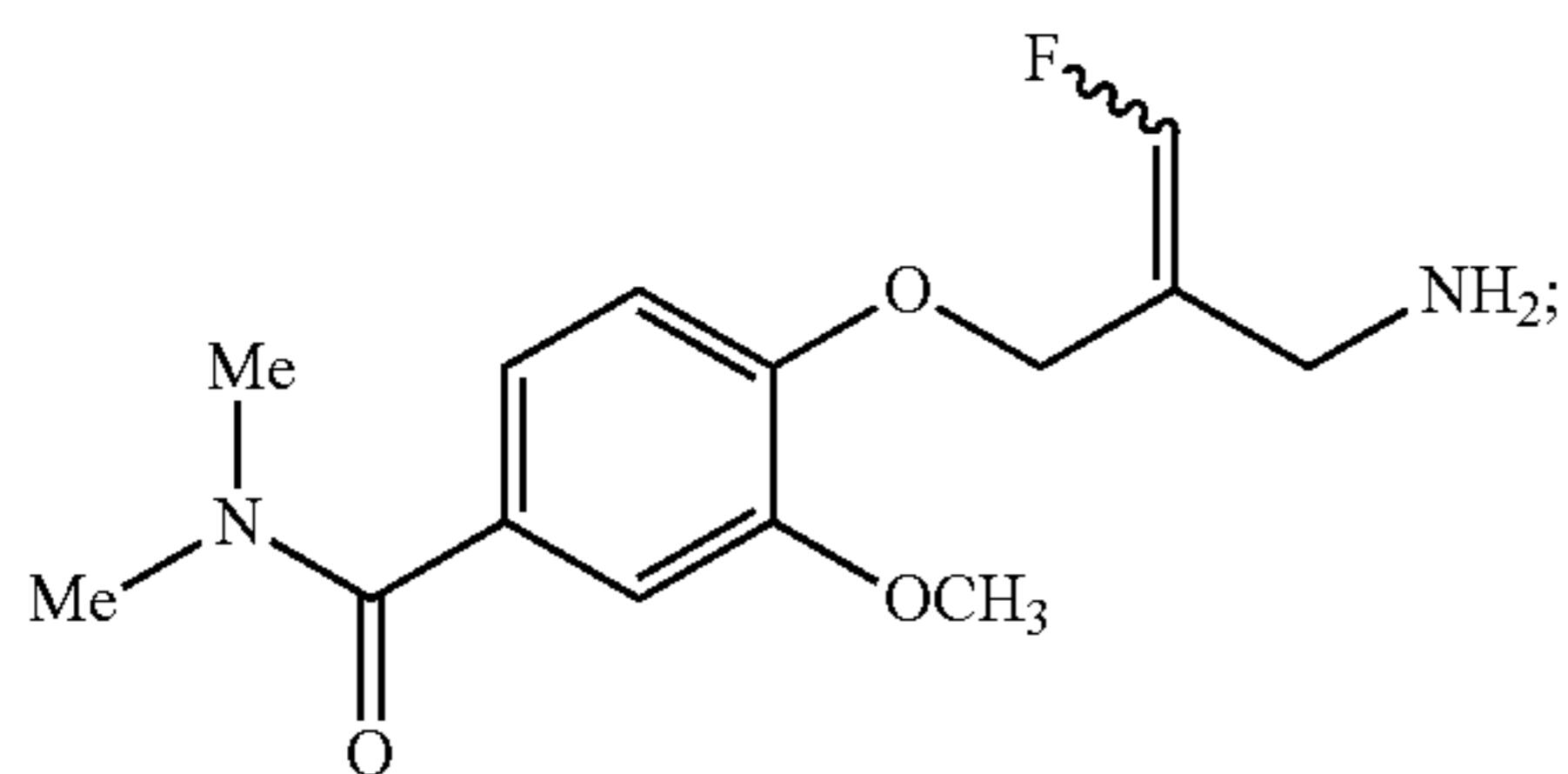
4-(2-(Aminomethyl)-3-fluoroallyloxy)-3-methoxy-N,N-dimethylbenzamide
