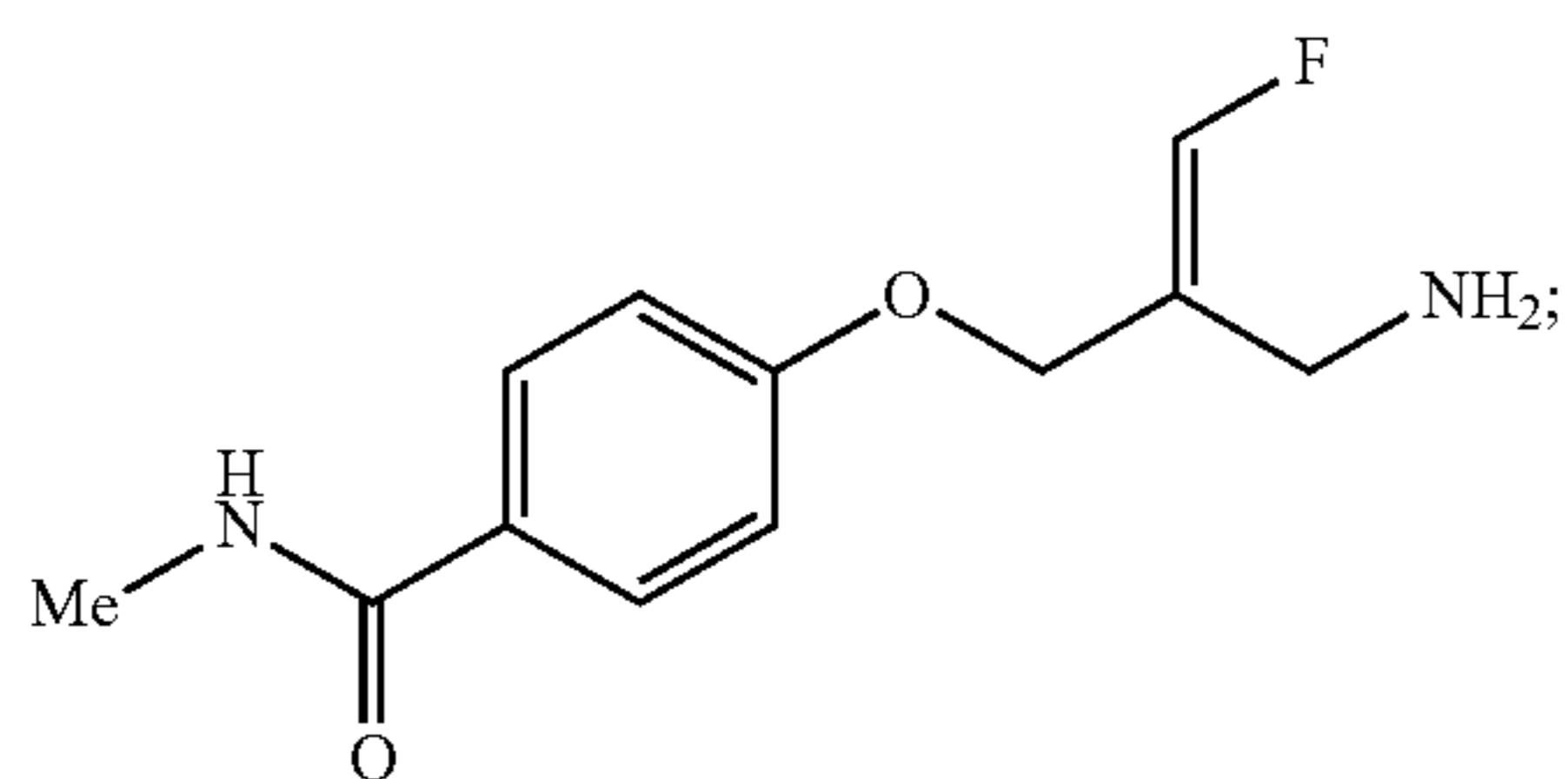
(E)-4-(2-(Aminomethyl)-3-fluoroallyloxy)-N-methylbenzamide
