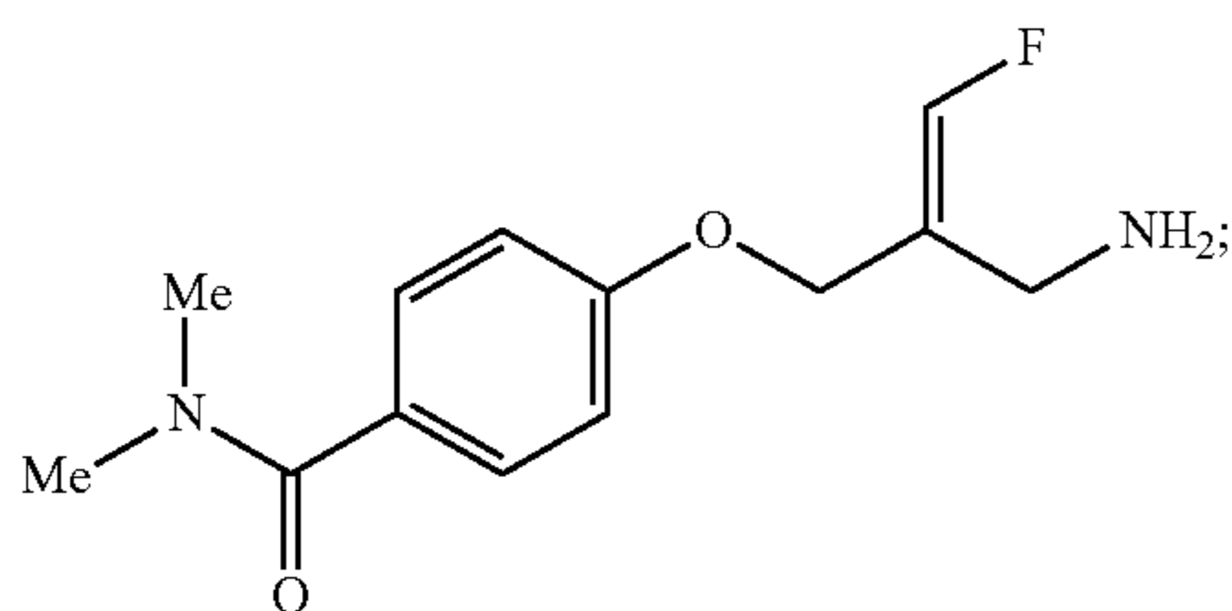
(E)-4-(2-(Aminomethyl)-3-fluoroallyloxy)-N,N-dimethylbenzamide
