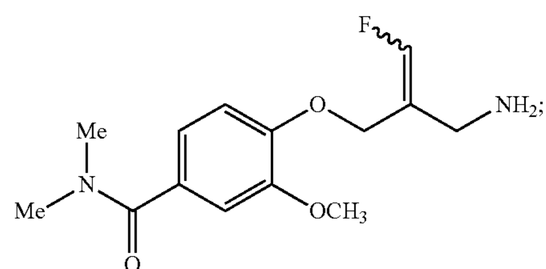
4-(2-(Aminomethyl)-3-fluoroallyloxy)-3-methoxy-N,N-dimethylbenzamide
