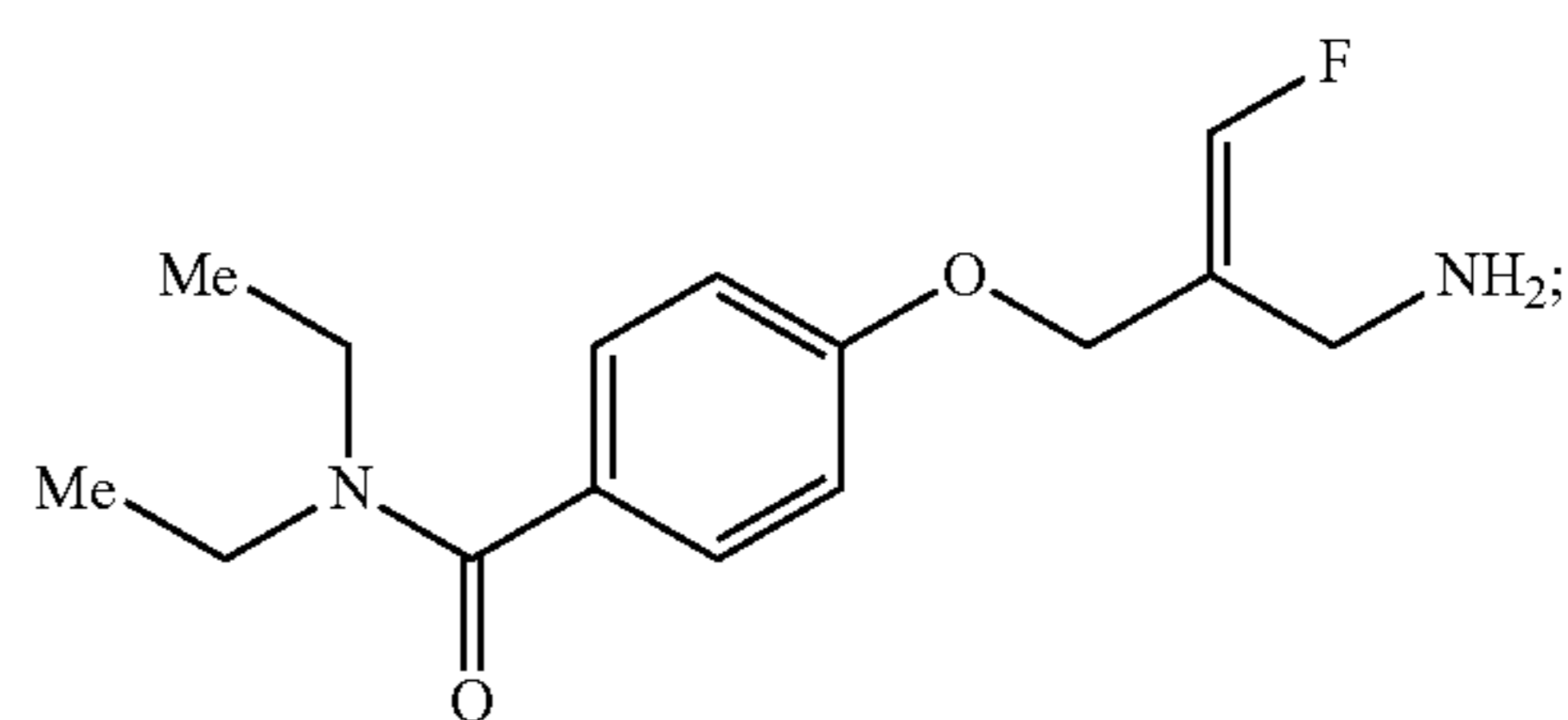
(E)-4-(2-(Aminomethyl)-3-fluoroallyloxy)-N,N-diethylbenzamide
