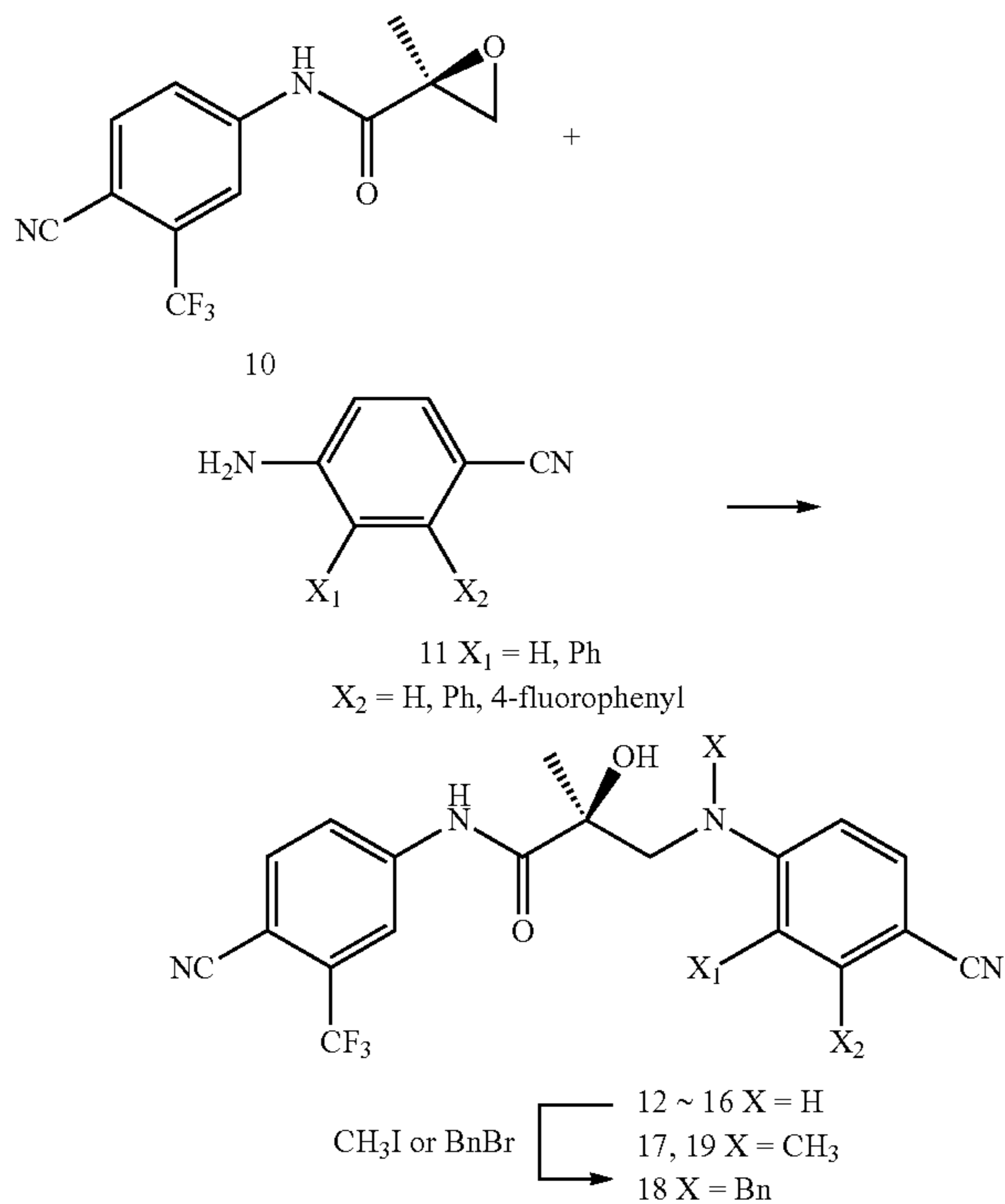
Scheme 3. Preparation of SARs 12-19.
