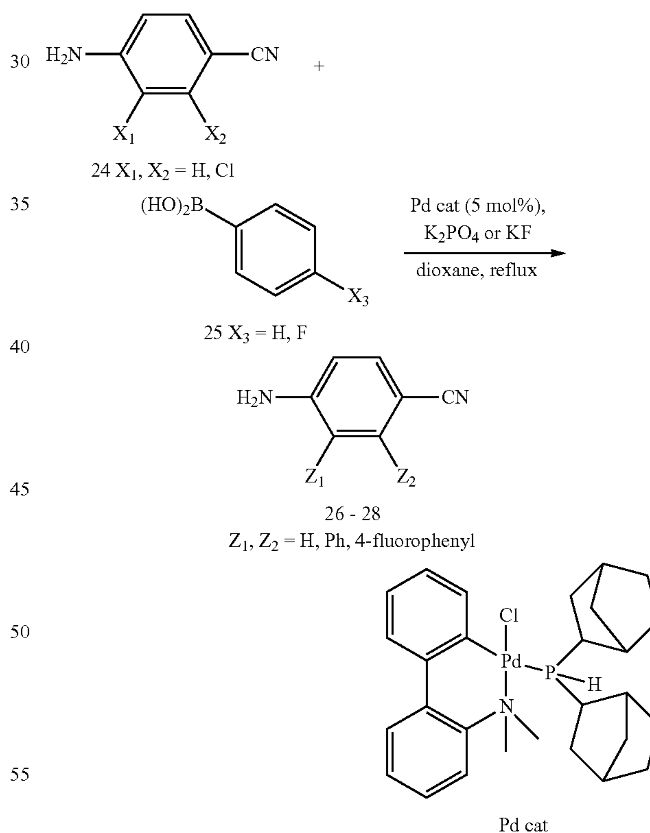
Scheme 2. Preparation of 4-cyano 2,3-substituted anilines (26-28).
