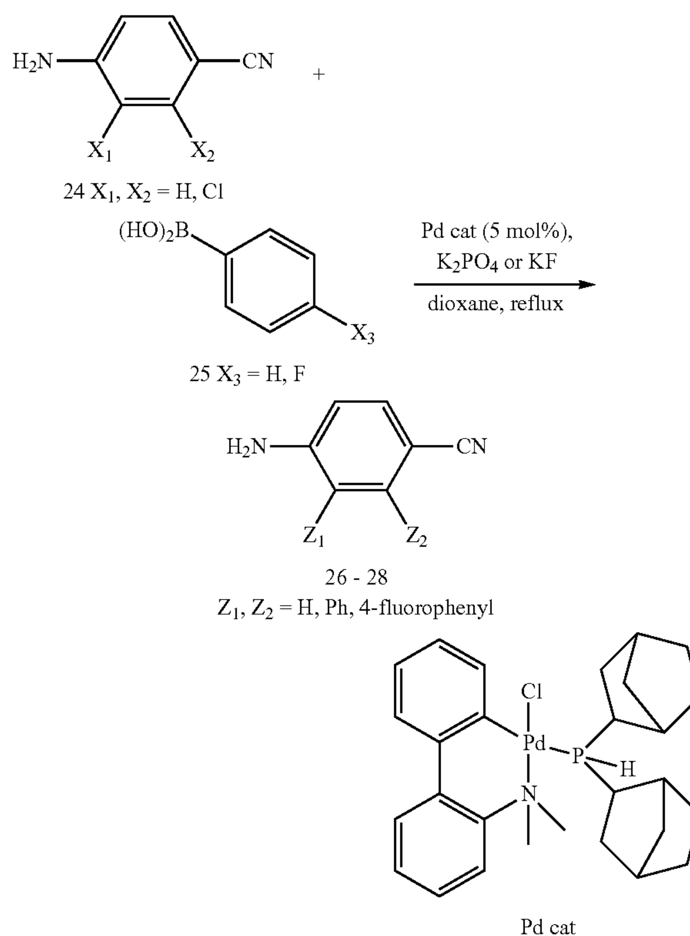
Scheme 2. Preparation of 4-cyano 2,3-substituted anilines (26-28).
