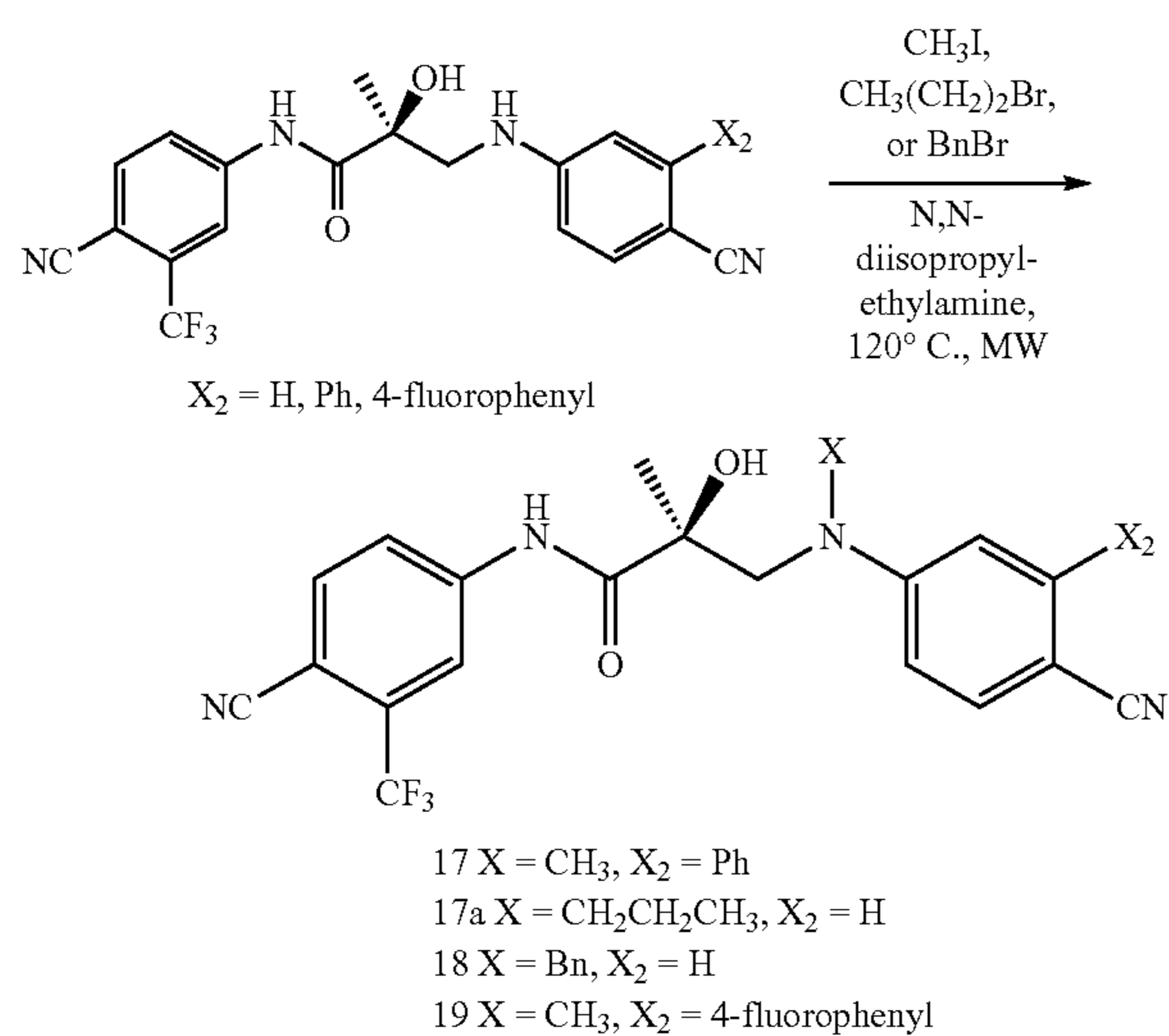
Scheme 4. Preparation of SARs 17-19 and 17a.
