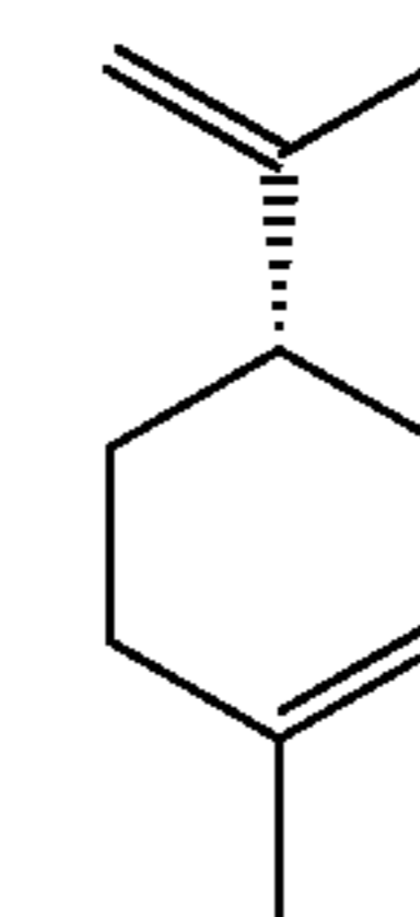
(-)-limonene
