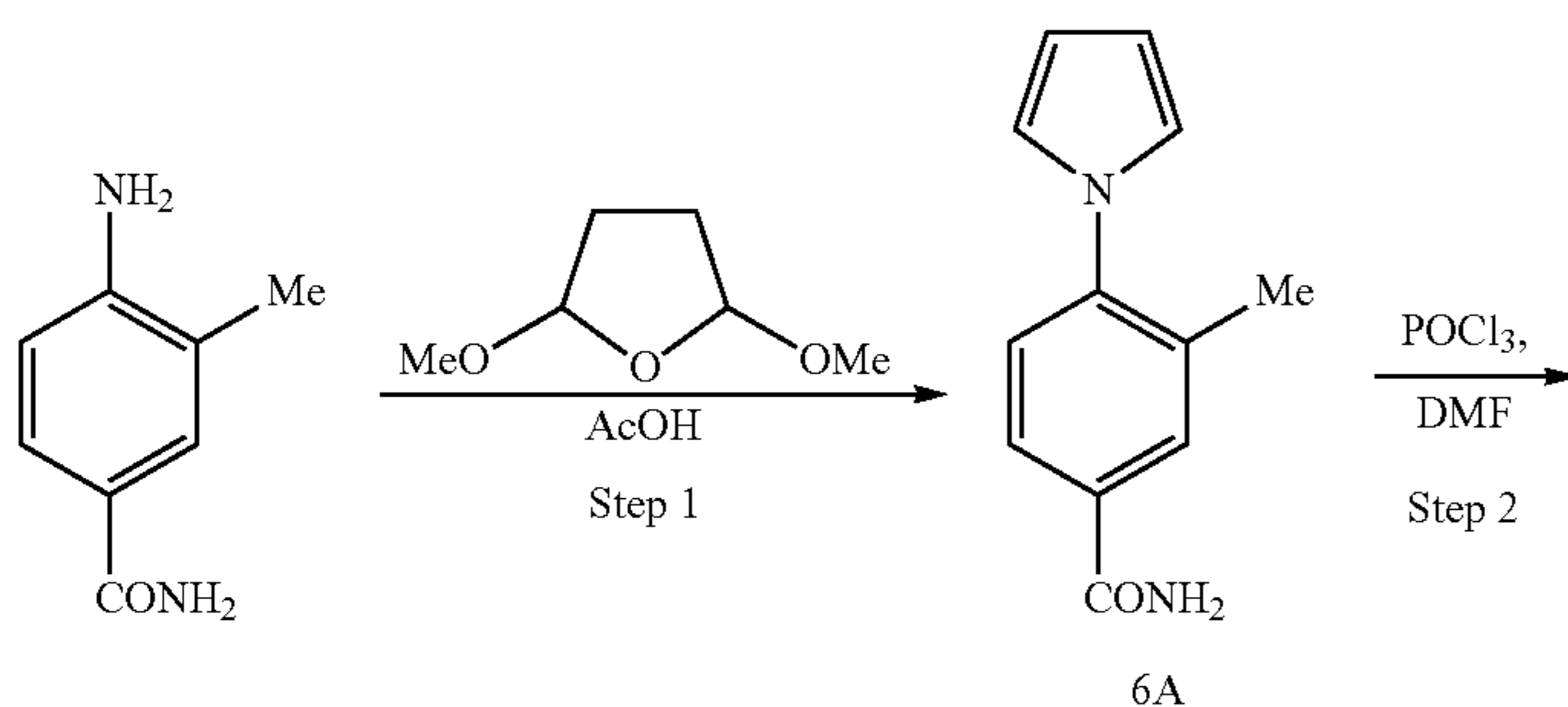
Scheme 6: A general scheme for preparing GSNOR inhibitors with structure 6H
