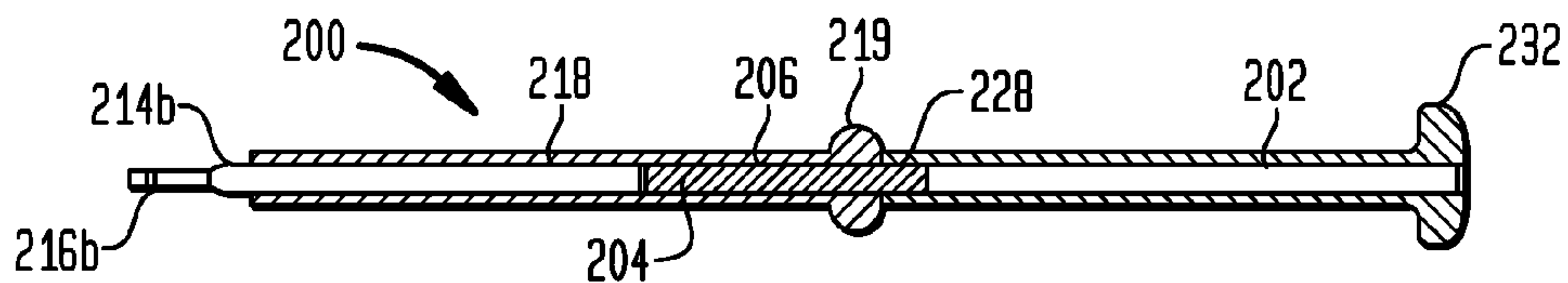
FIG. 31 (SECTION A-A OF FIG. 22)
