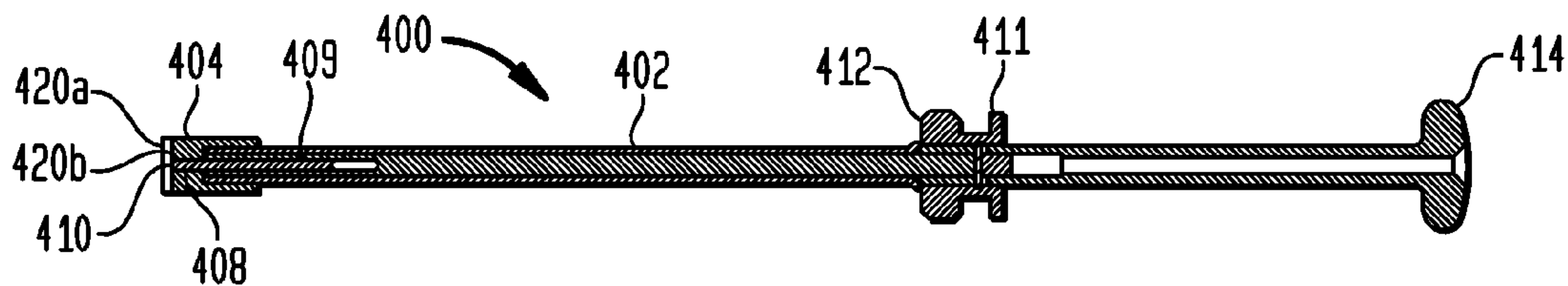
FIG. 57 (SECTION A-A OF FIG. 56)
