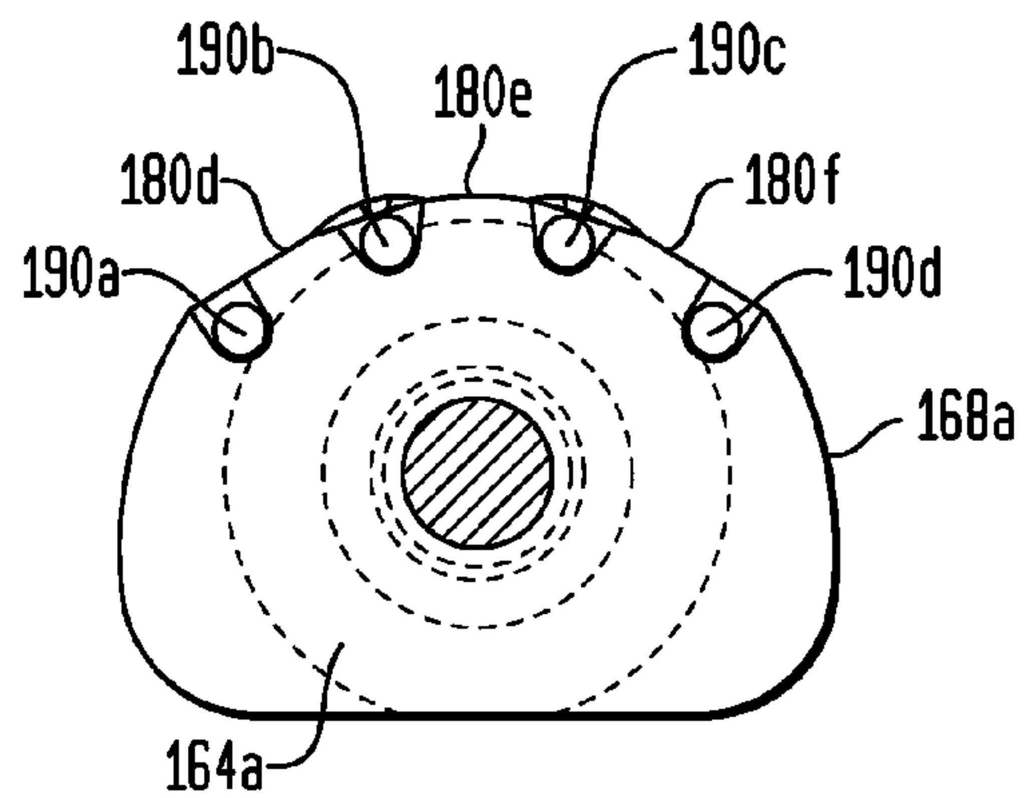
FIG. 17 (SECTION A-A OF FIG. 13)
