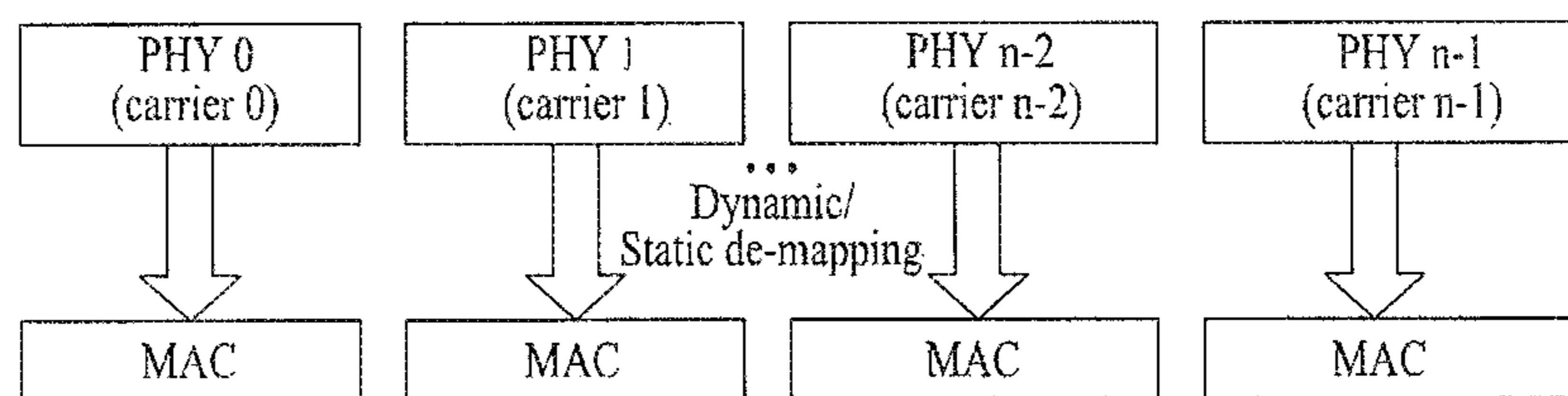
(b) Receiver
