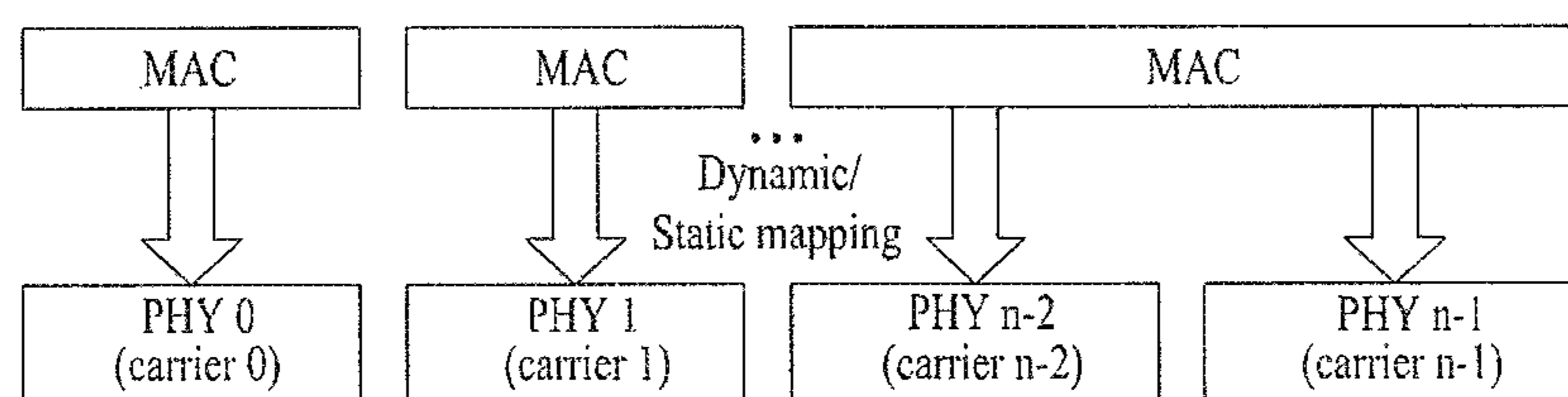
(a) Transmitter
