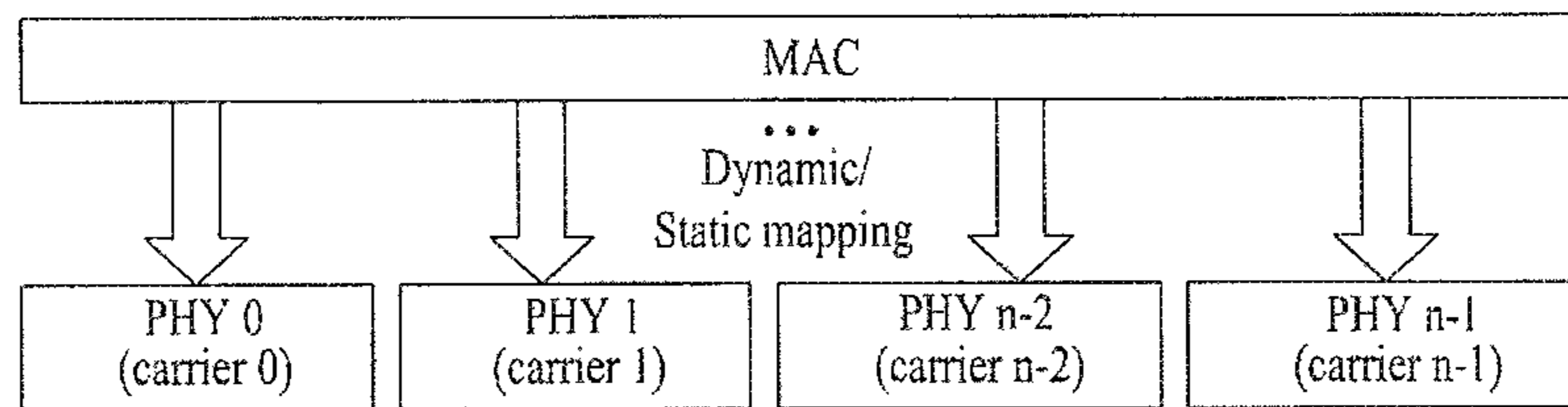
(a) Transmitter
