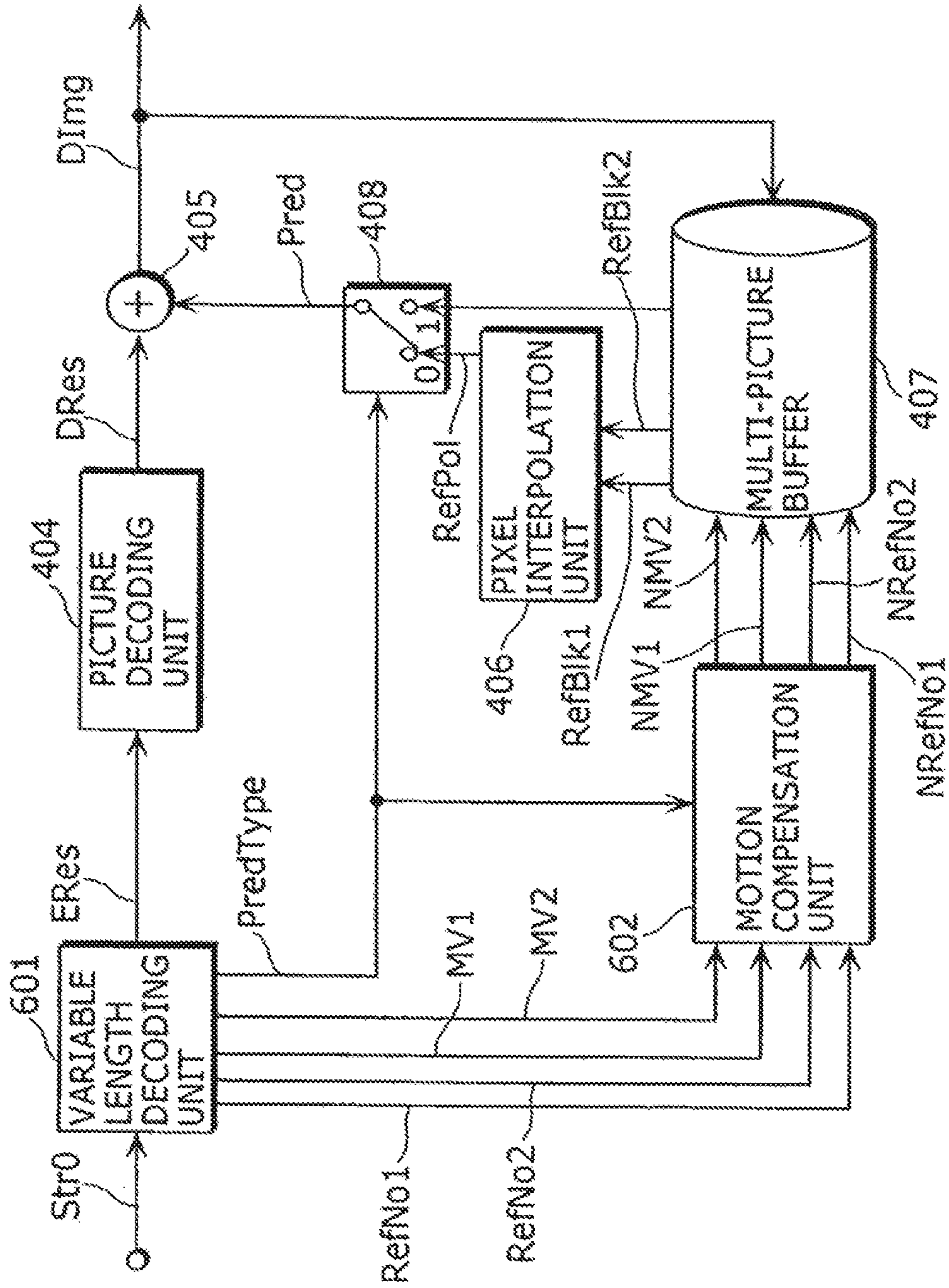
FIG. 4 PRIOR ART
