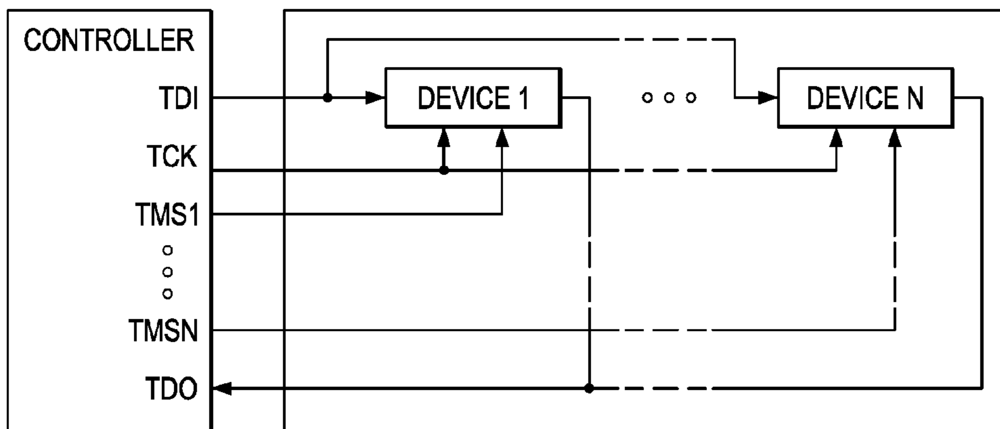
FIG. 5 (PRIOR ART)
