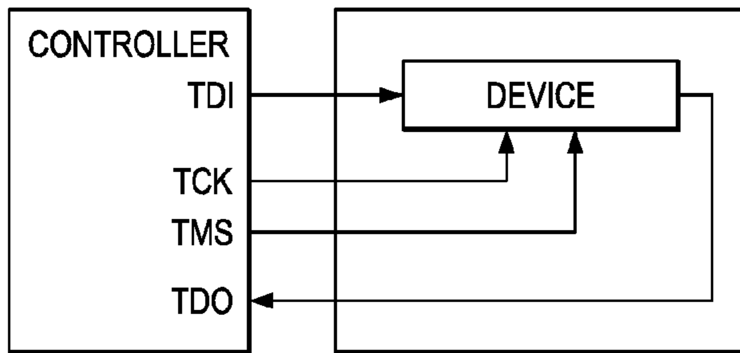
FIG. 4 (PRIOR ART)
