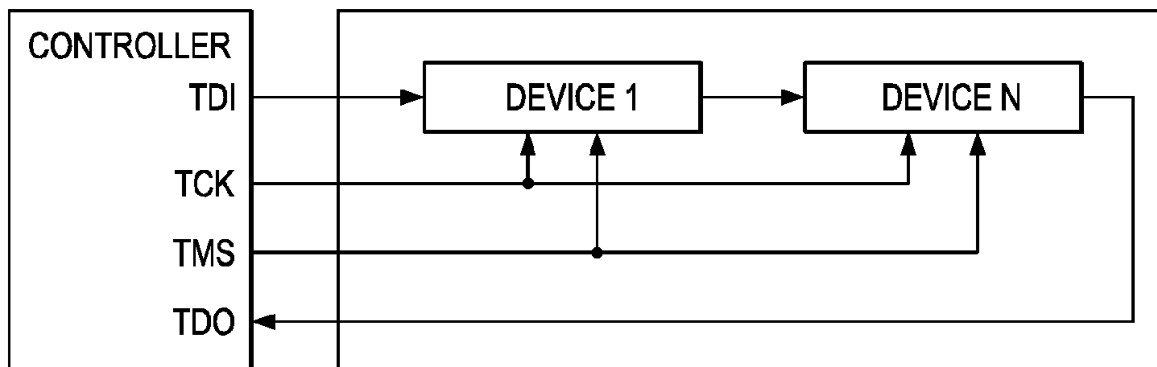
FIG. 6 (PRIOR ART)
