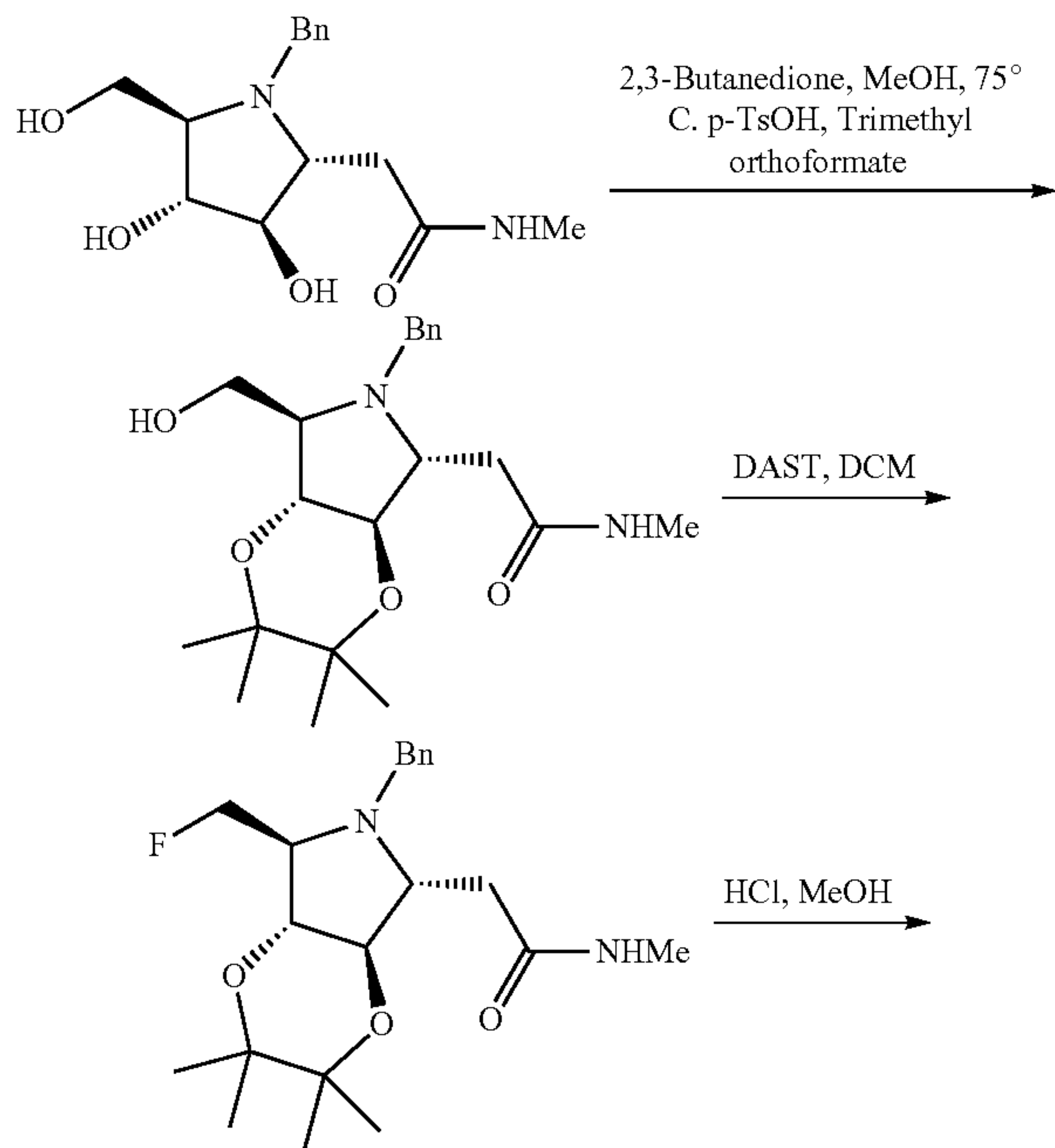
Scheme 19
