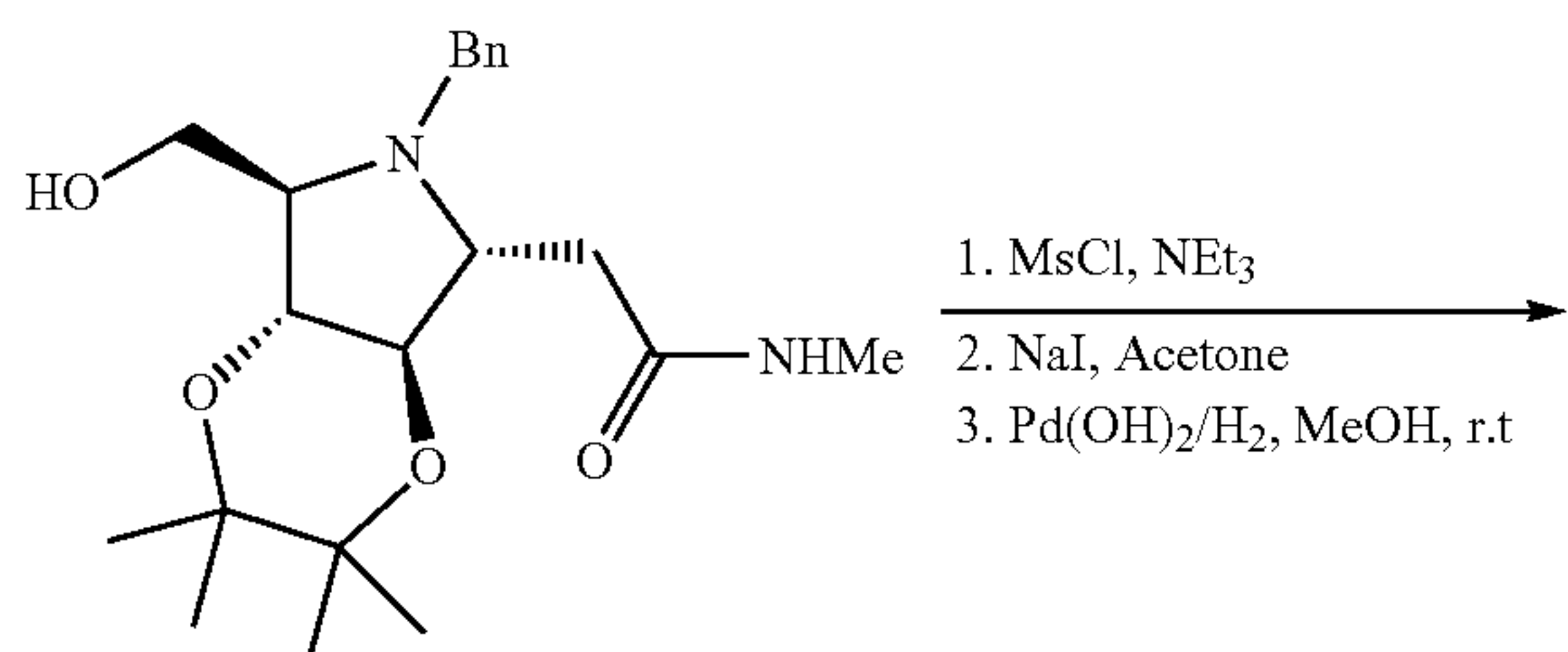
Scheme 21
