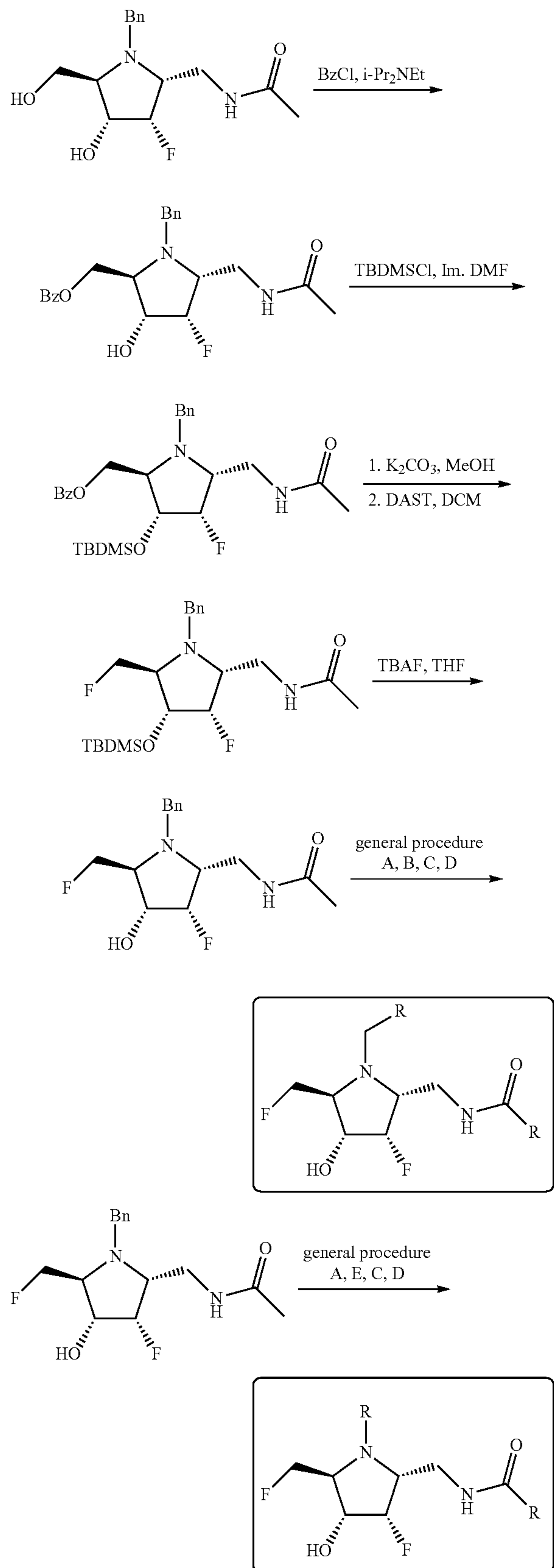
Scheme 14
