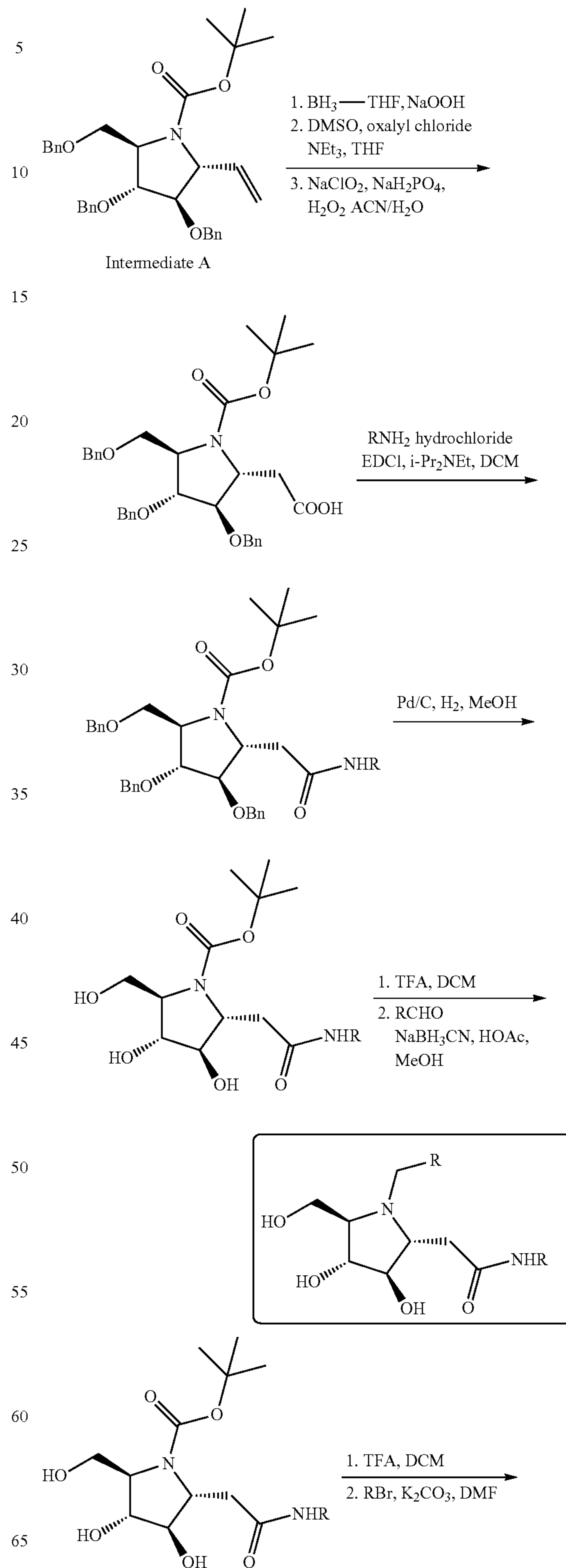
Scheme 15
