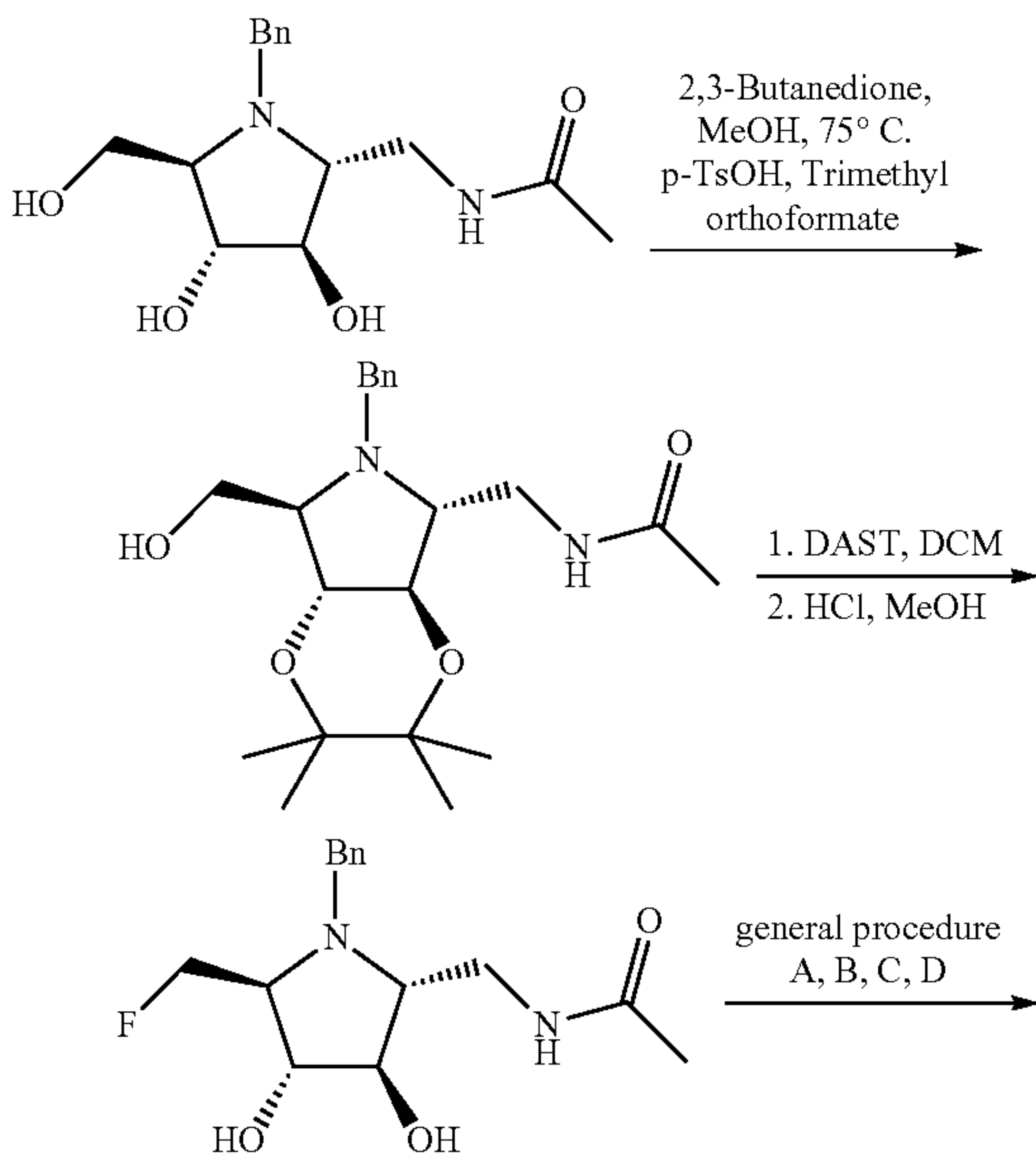
Scheme 7
