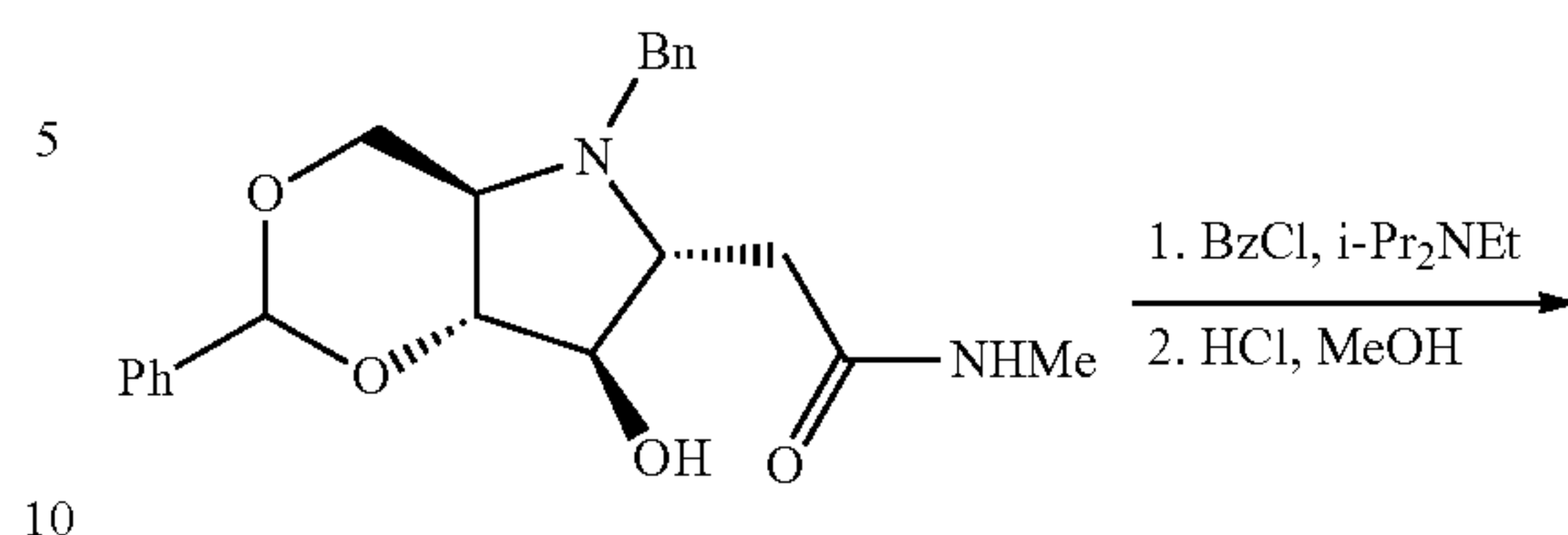
Scheme 22
