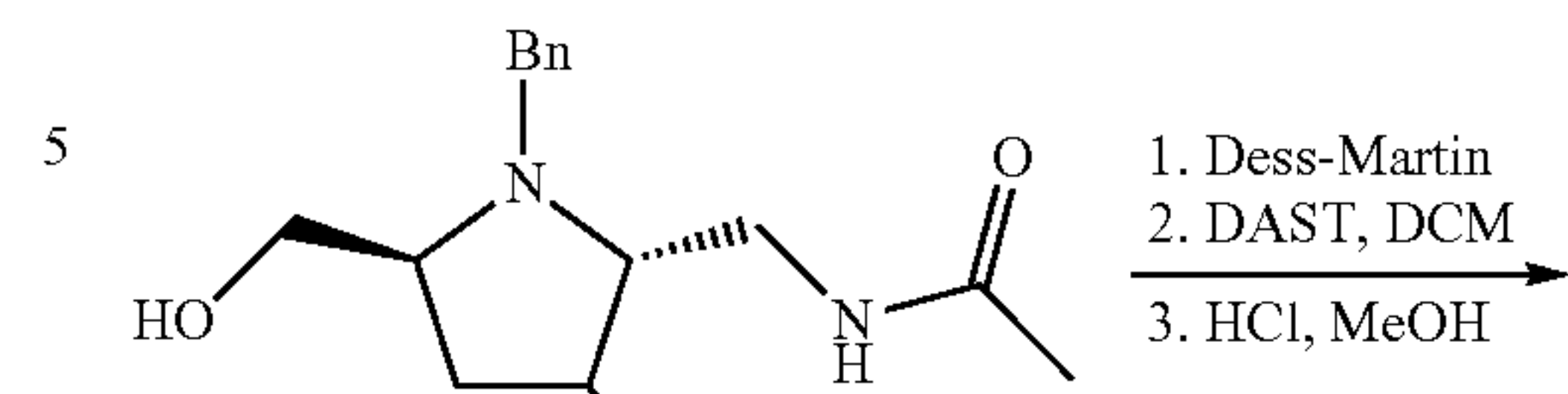
Scheme 8
