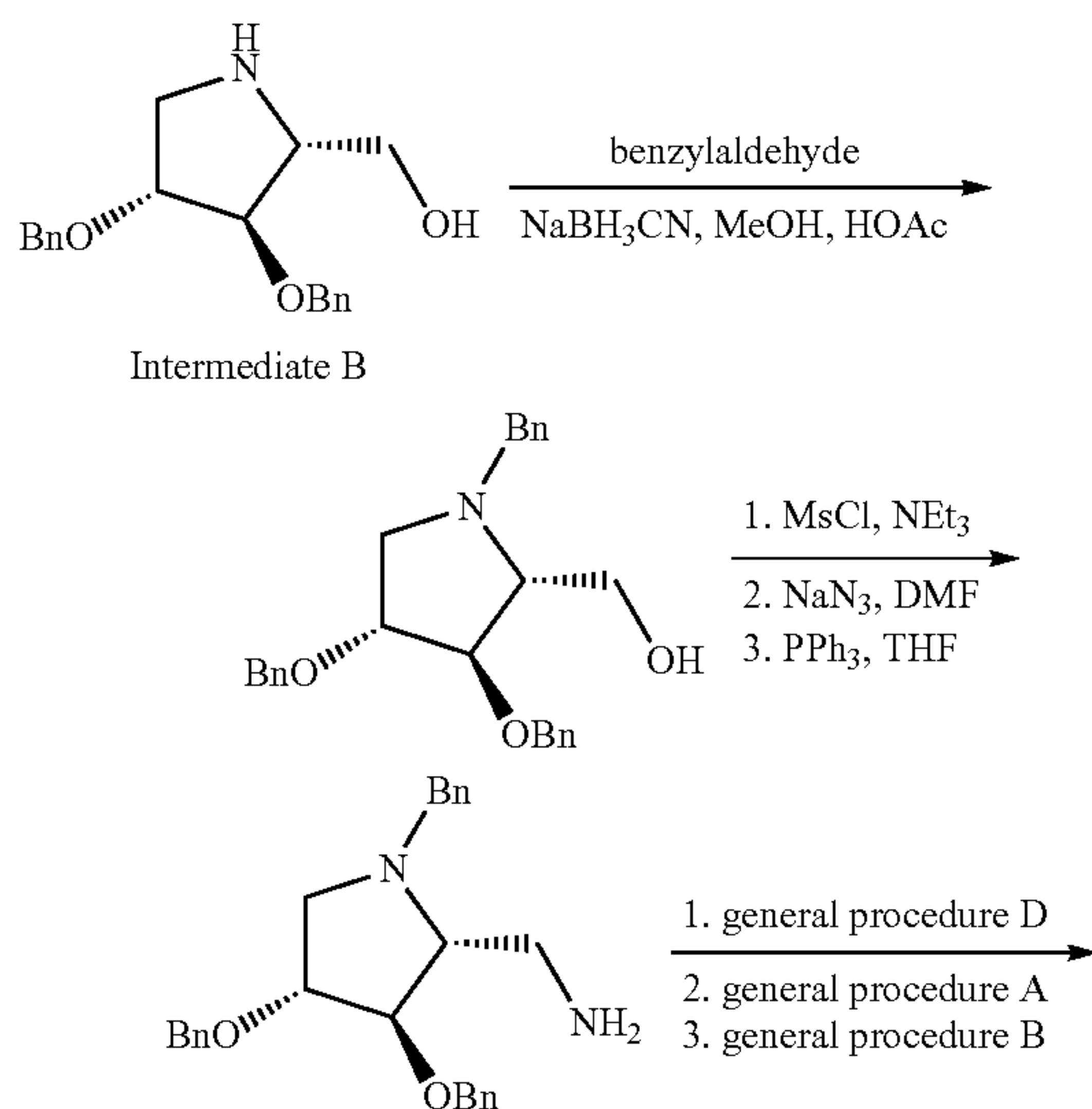
Scheme 26
