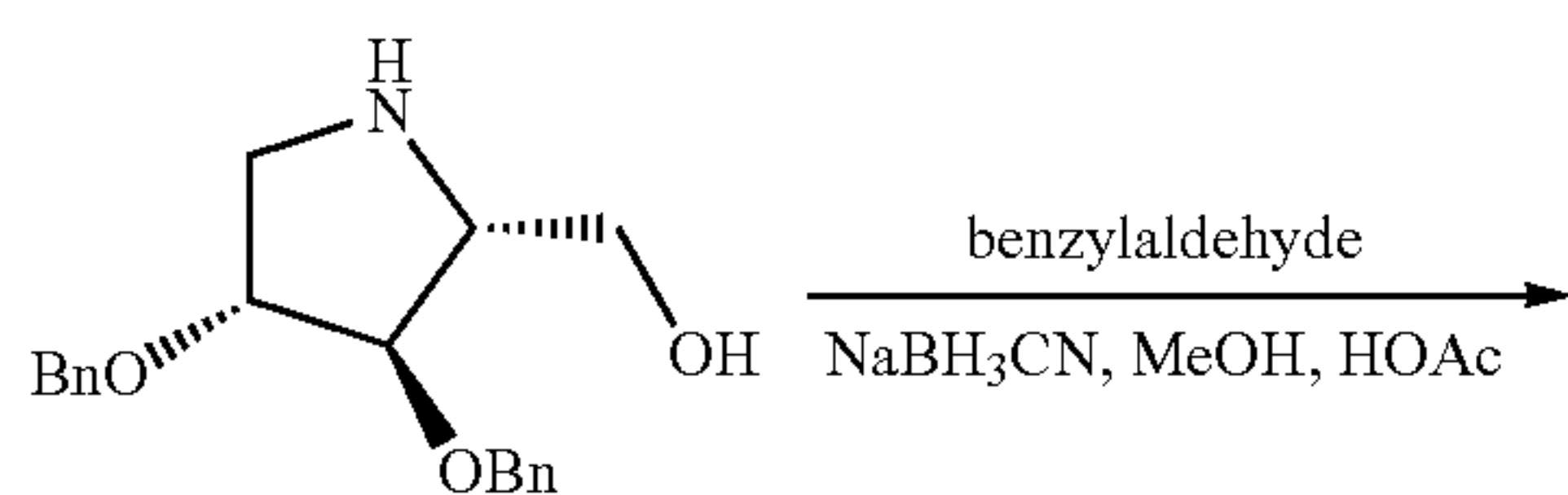
Scheme 27
