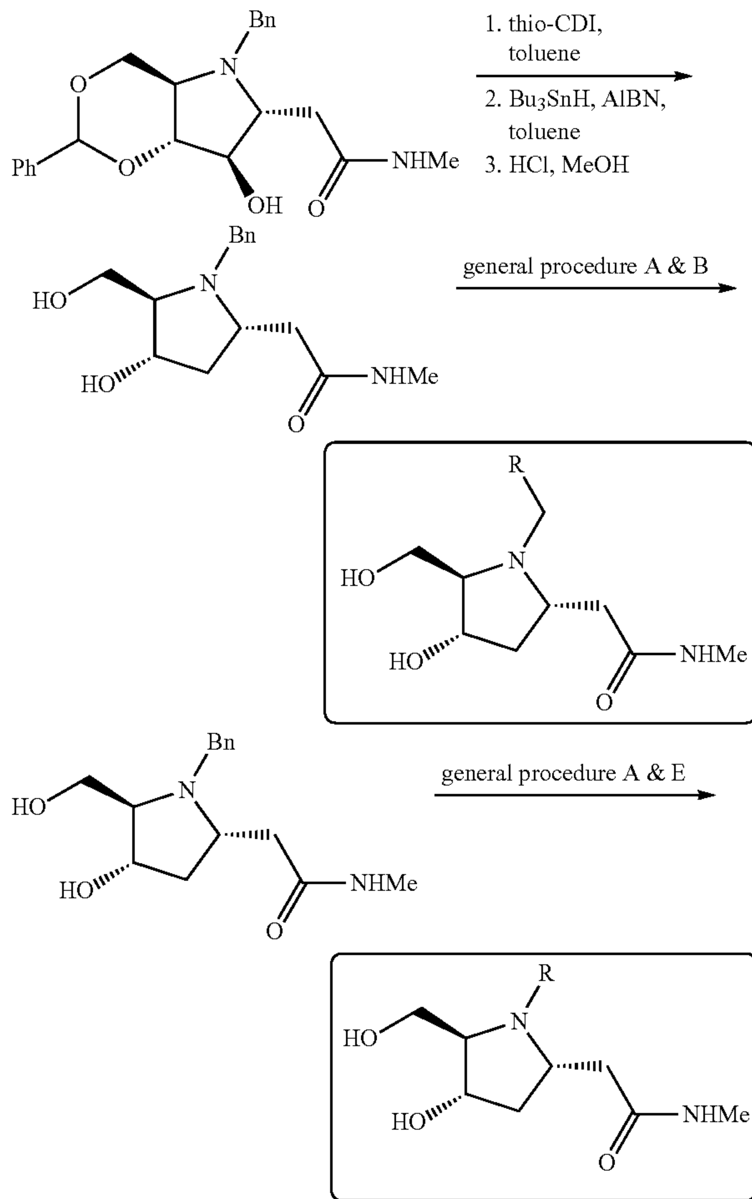
Scheme 18
