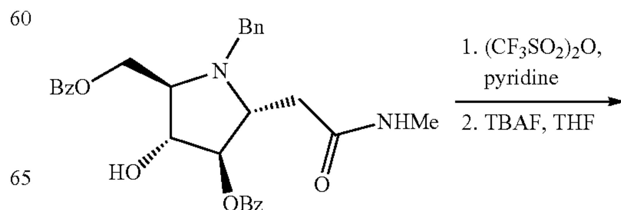
Scheme 23
