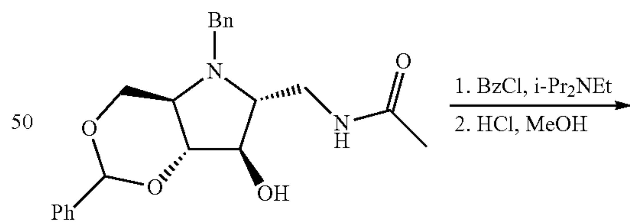
Scheme 9
