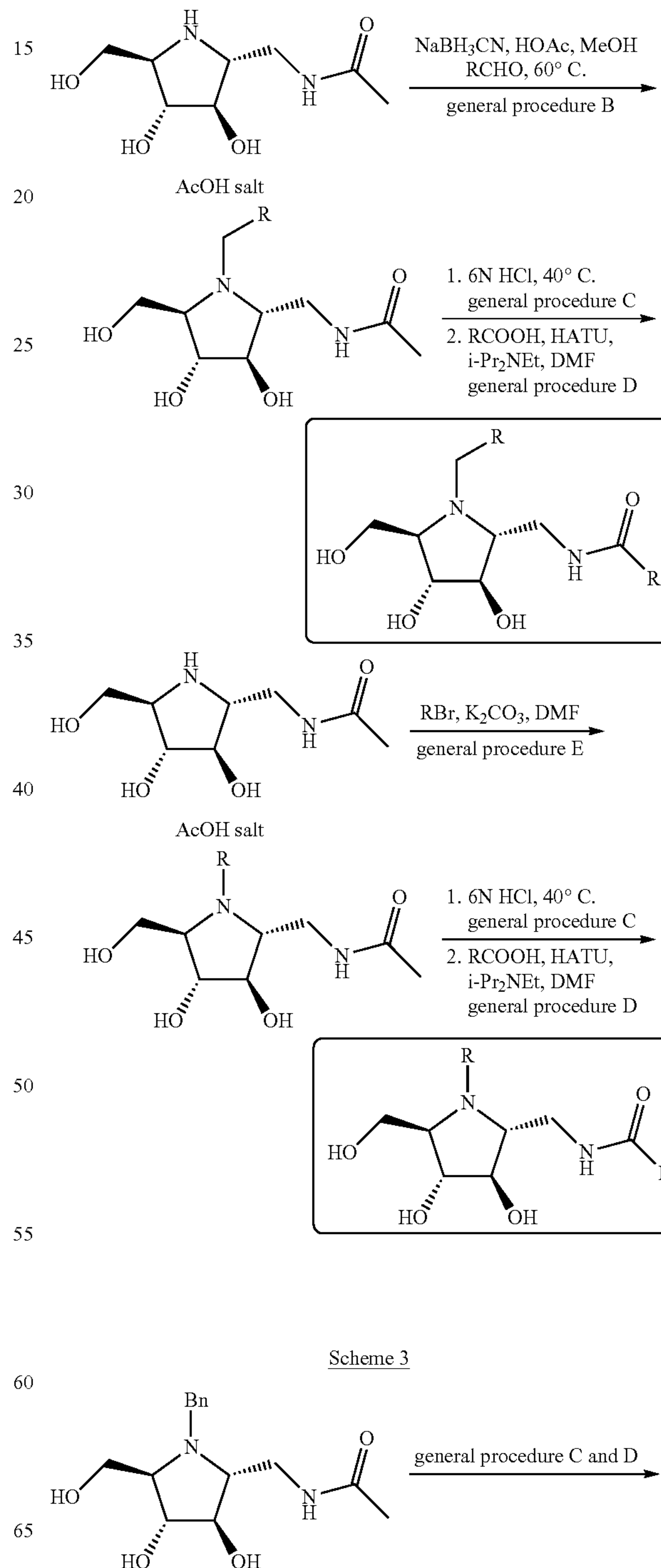
Scheme 2
