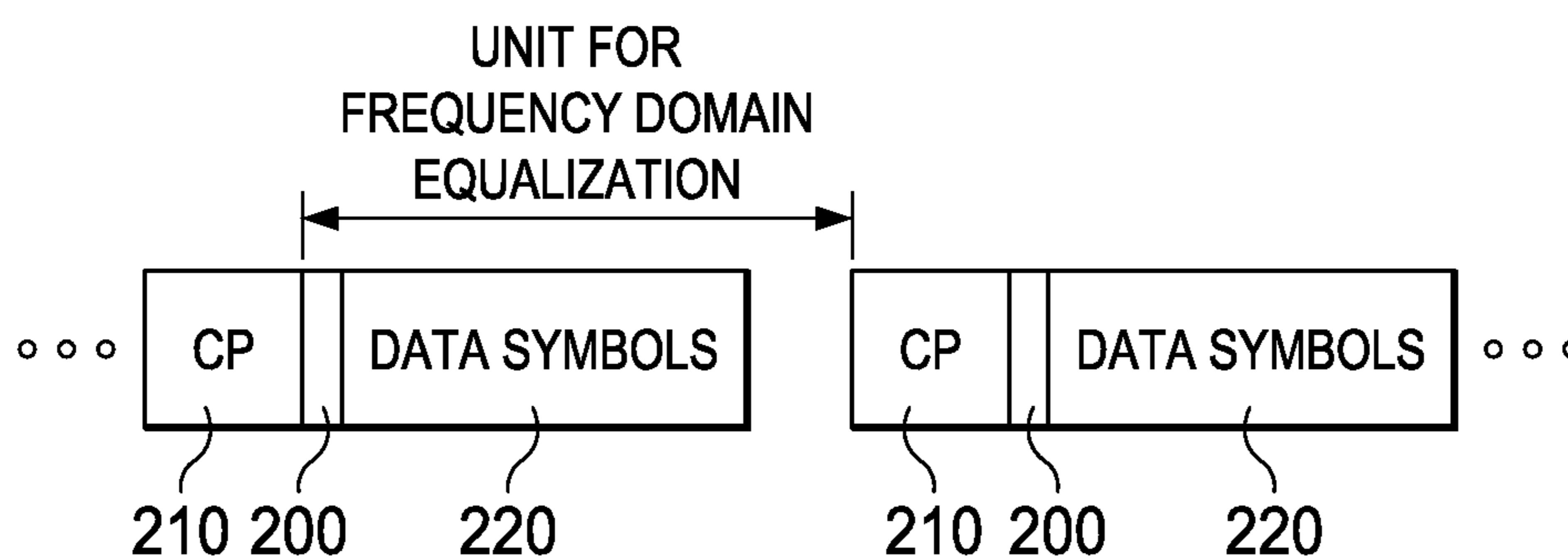
FIG. 2 (PRIOR ART)
