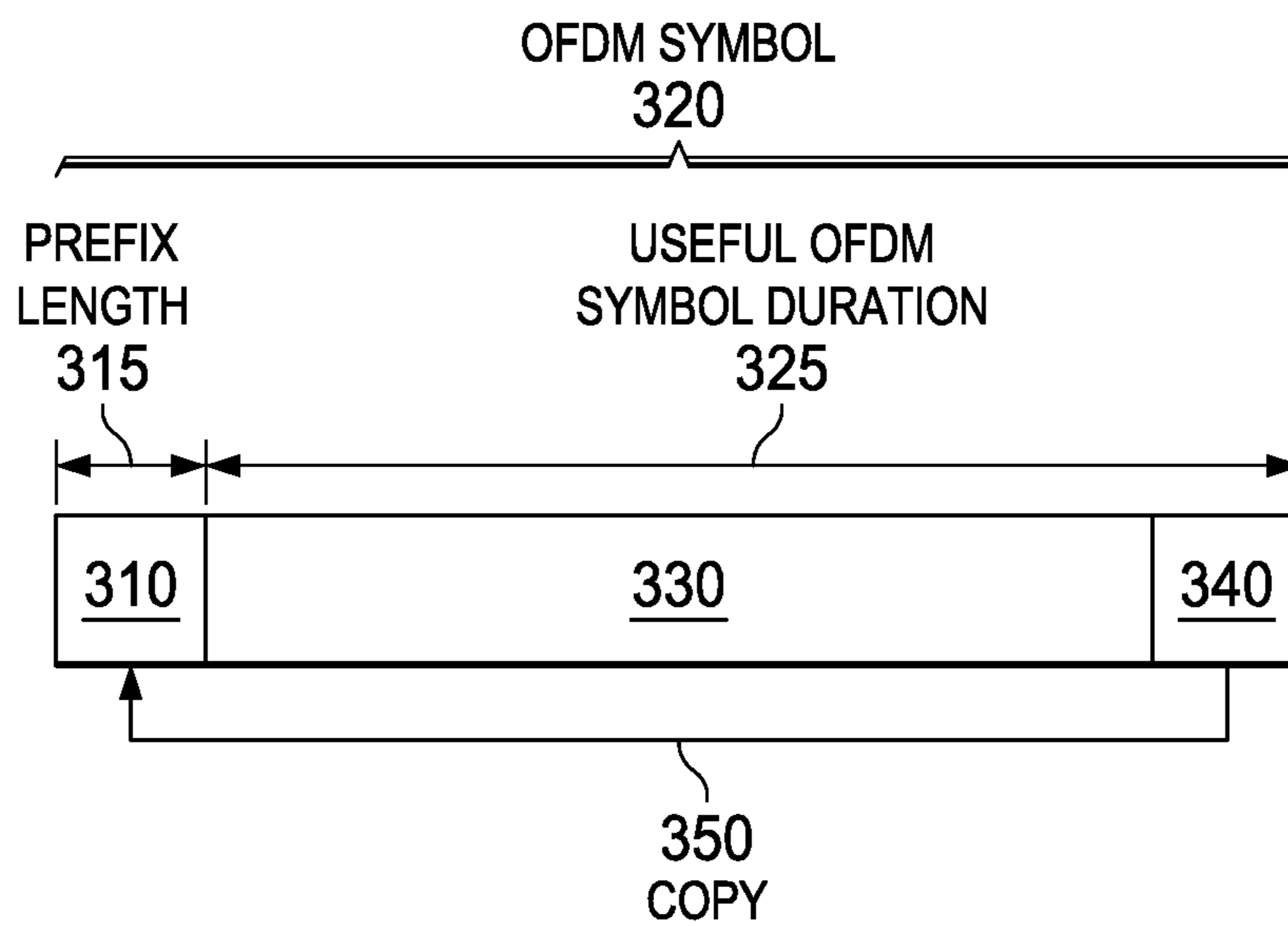
FIG. 3 (PRIOR ART)
