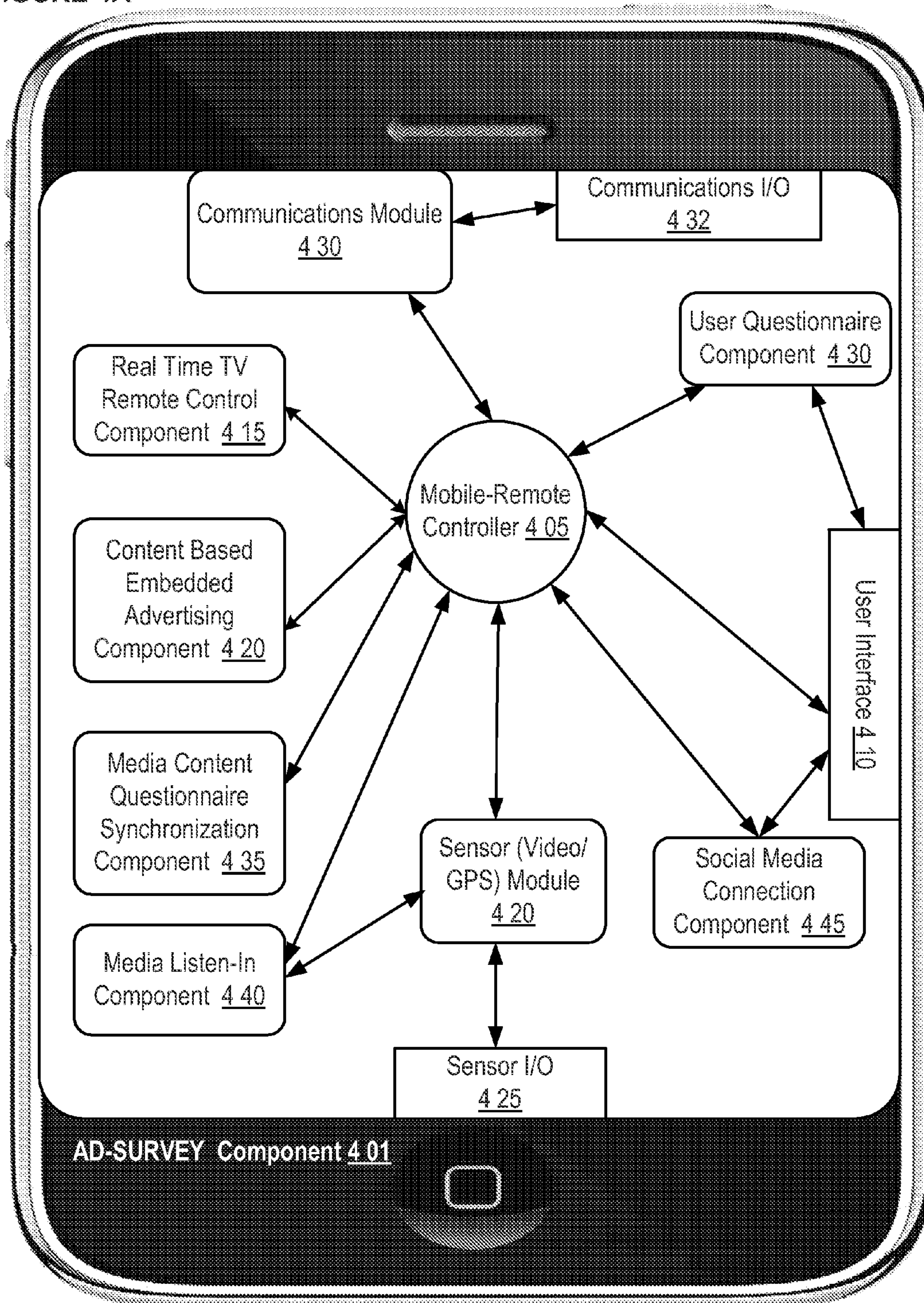
AD-SURVEY Example Client Mobile App Block View
