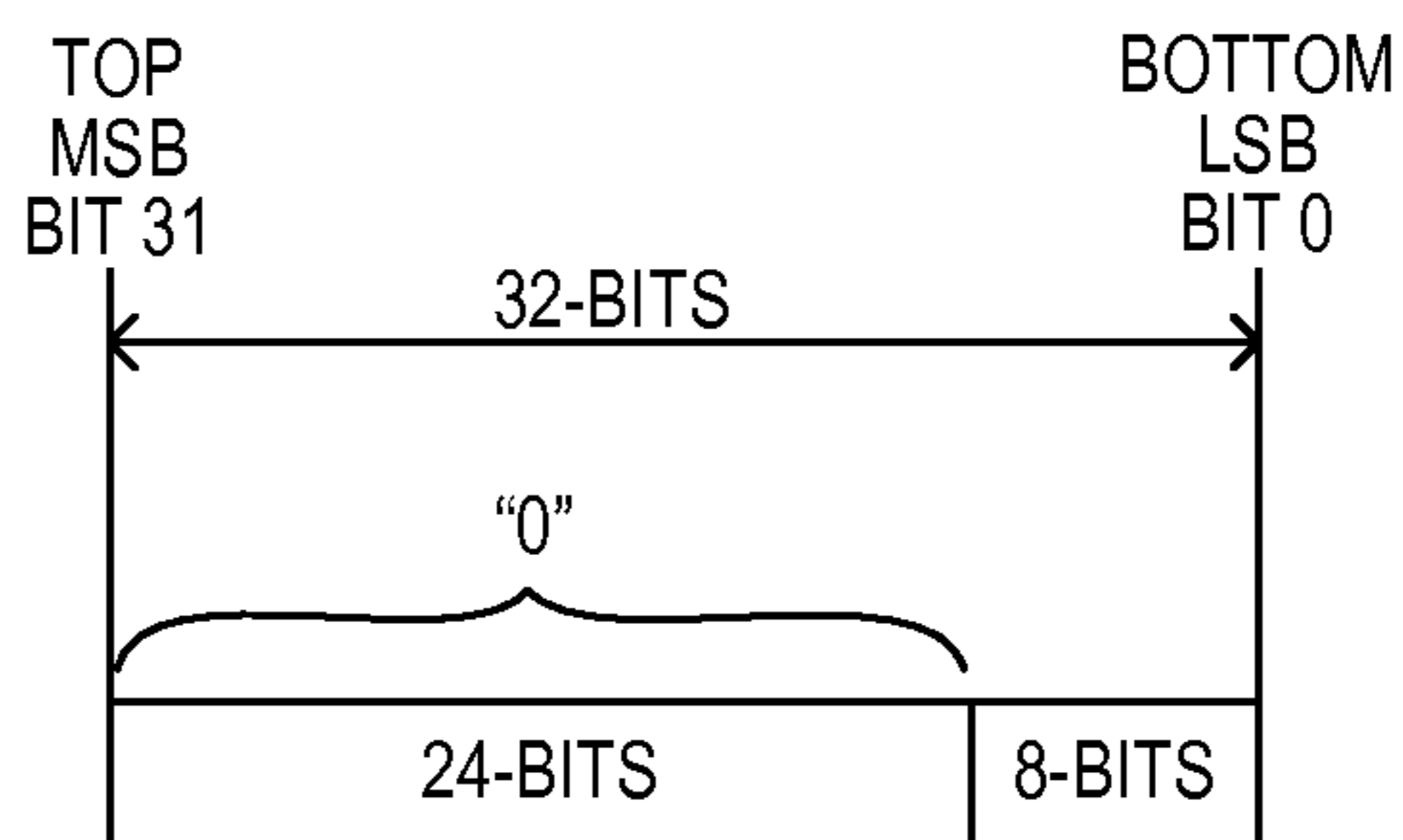
OUTPUT FROM REDUCE TABLE B (32-BITS)
