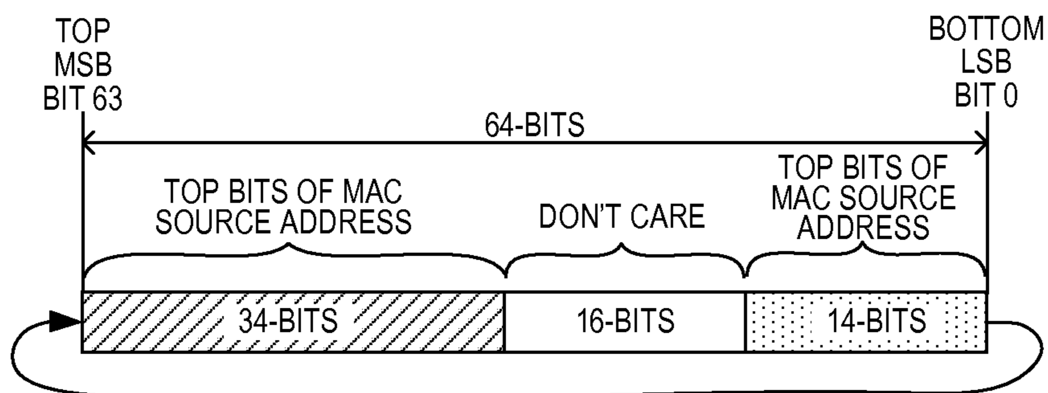
OUTPUT OF BARREL SHIFTER (64-BITS)
