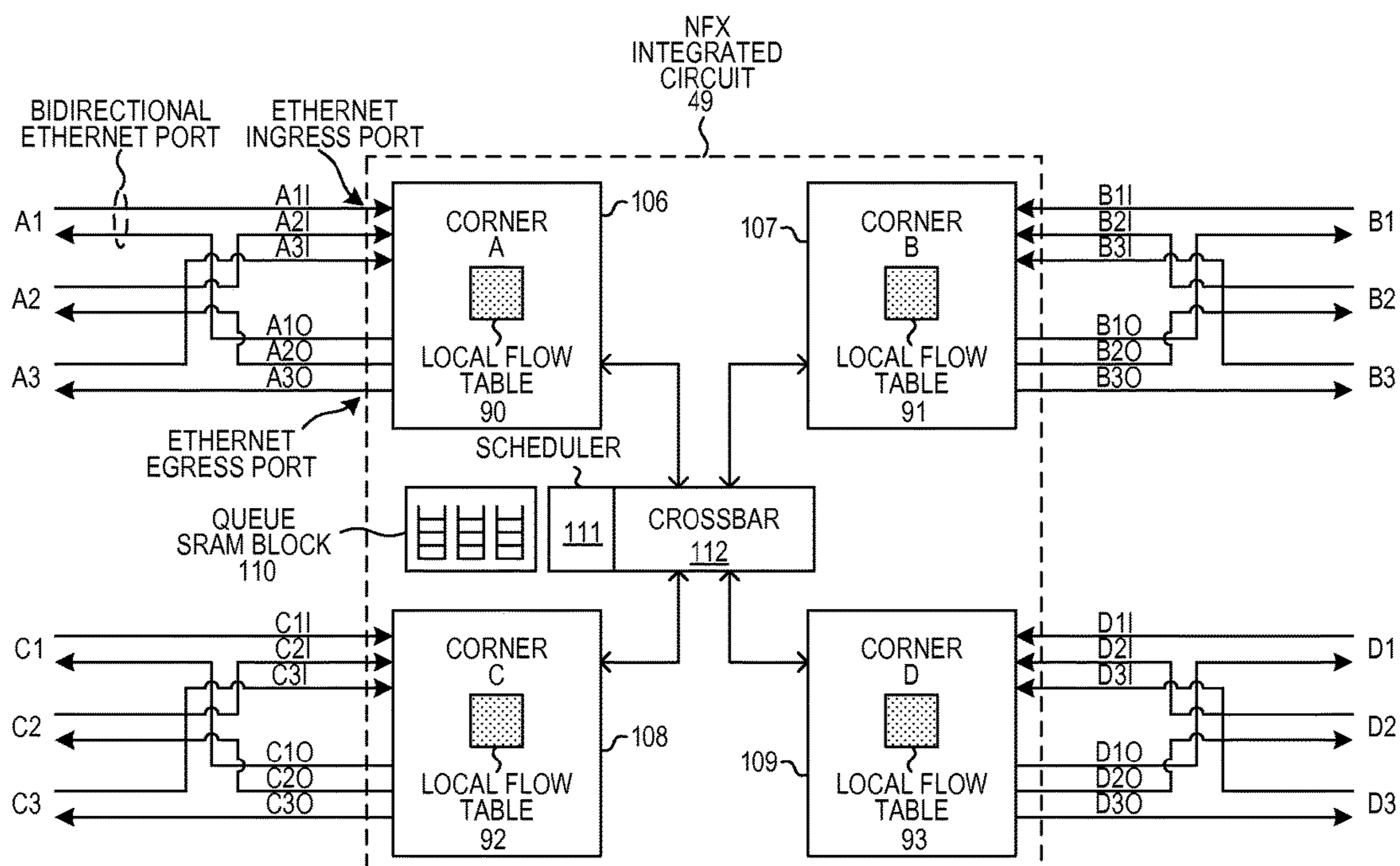
ONE NFX CIRCUIT
