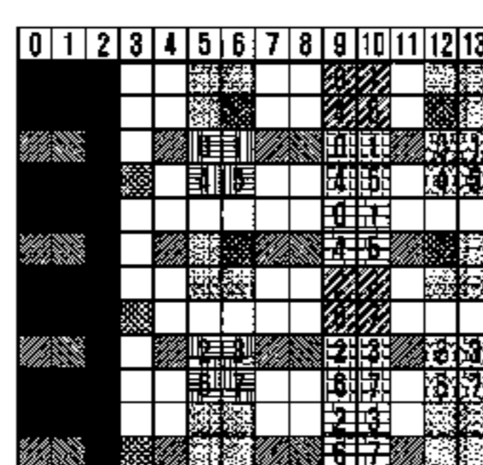
(c) 8 CSI-RS ports
