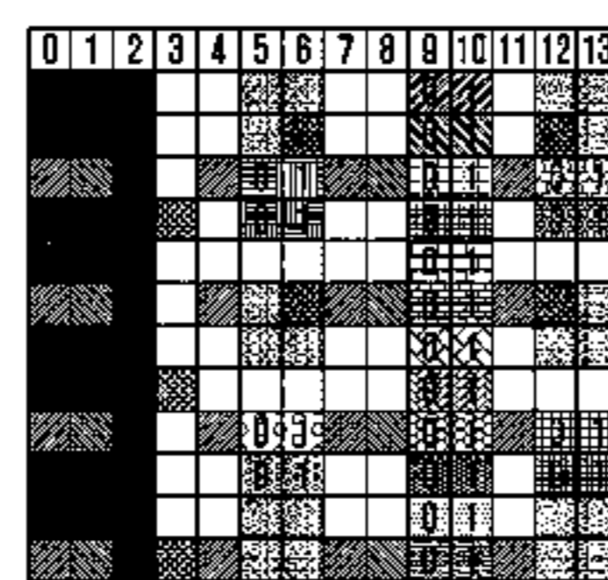
(a) 2 CSI-RS ports
